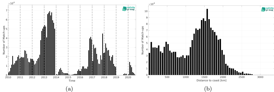
Figure 1: Number of match-ups between Surface drifters and SMOS SSS L4 v1 - Monthly (CMEMS-CNR) SSS as a function of time (a) and as function of the distance to coast (b) over the Global Ocean Pi-MEP region and for the full satellite product period.
