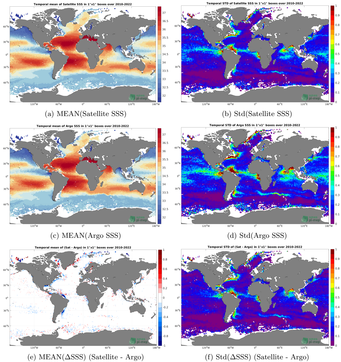
Figure 6: Temporal mean (left) and Std (right) of SSS from SMOS SSS L4 v1 - Monthly (CMEMS-CNR) (top), Argo (middle), and of \Delta SSS (Satellite - Argo). Only match-up pairs are used to generate these maps.
