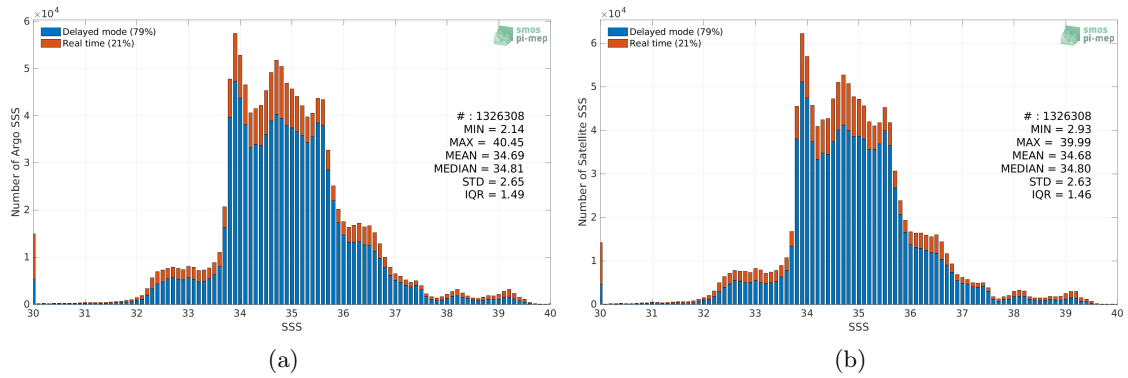
Figure 2: Histograms of SSS from Argo (a) and SMOS SSS L4 v1 - Monthly (CMEMS-CNR) (b) considering all match-up pairs per bins of 0.1 over the Global Ocean Pi-MEP region and for the full satellite product period.
