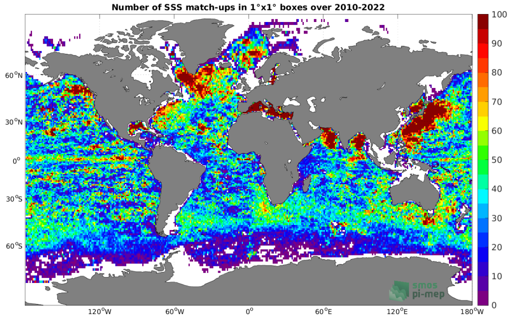
Figure 4: Number of SSS match-ups between Argo SSS and the SMOS SSS L4 v1 - Monthly (CMEMS-CNR) SSS product for the Global Ocean Pi-MEP region over 1^\circ \times 1^\circ boxes and for the full satellite product period.
