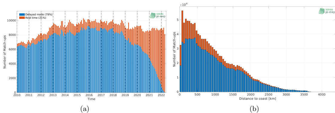
Figure 1: Number of match-ups between Argo and SMOS SSS L4 v1 - Monthly (CMEMS-CNR) SSS as a function of time (a) and as function of the distance to coast (b) over the Global Ocean Pi-MEP region and for the full satellite product period.
