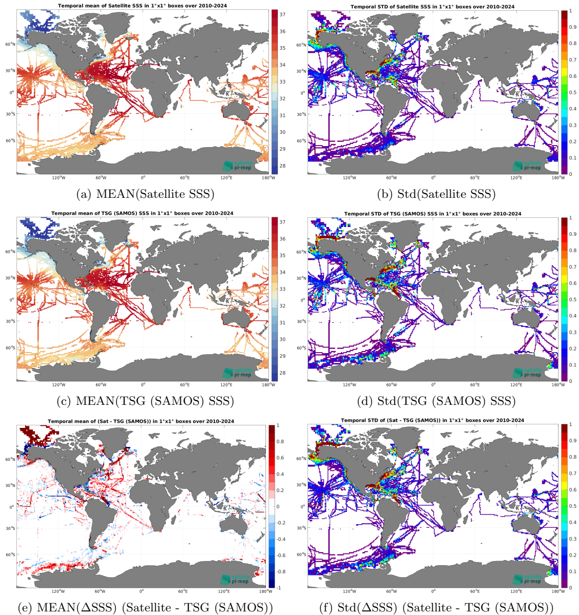
Figure 7: Temporal mean (left) and Std (right) of SSS from SMOS SSS L4 v1 - Daily (CMEMS-CNR) (top), TSG (SAMOS) (middle), and of \Delta SSS (Satellite - TSG (SAMOS)). Only match-up pairs are used to generate these maps.
