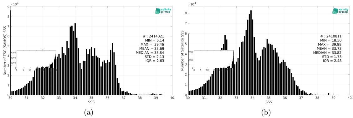
Figure 3: Histograms of SSS from TSG (SAMOS) (a) and SMOS SSS L4 v1 - Daily (CMEMS-CNR) (b) considering all match-up pairs per bins of 0.1 over the Global Ocean Pi-MEP region and for the full satellite product period.
