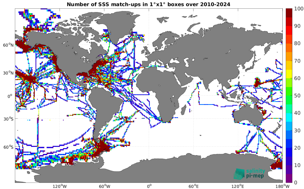
Figure 5: Number of SSS match-ups between TSG (SAMOS) SSS and the SMOS SSS L4 v1 - Daily (CMEMS-CNR) SSS product for the Global Ocean Pi-MEP region over 1^\circ \times 1^\circ boxes and for the full satellite product period.
