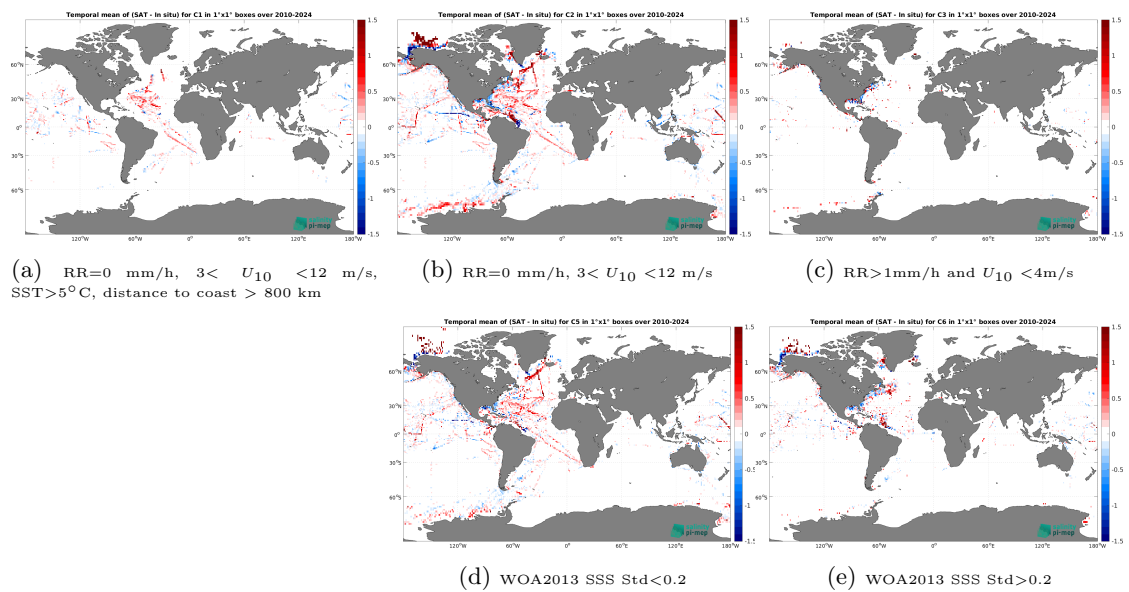
Figure 14: Temporal mean gridded over spatial boxes of size 1^\circ \times 1^\circ of \Delta SSS (SMOS SSS L4 v1 - Daily (CMEMS-CNR) - TSG (SAMOS)) for 5 different subdatasets corresponding to:RR=0 mm/h, 3 < U_{10} < 12 m/s, SST>5°C, distance to coast > 800 km (a), RR=0 mm/h, 3 < U_{10} < 12 m/s (b), RR>1mm/h and U_{10} < 4 m/s (c), WOA2013 SSS Std<0.2 (d), WOA2013 SSS Std>0.2 (e).
