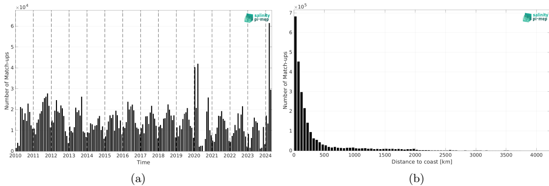
Figure 2: Number of match-ups between TSG (SAMOS) and SMOS SSS L4 v1 - Daily (CMEMS-CNR) SSS as a function of time (a) and as function of the distance to coast (b) over the Global Ocean Pi-MEP region and for the full satellite product period.
