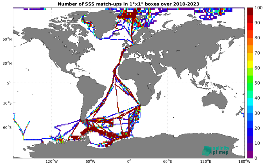
Figure 5: Number of SSS match-ups between TSG (Polarstern) SSS and the SMOS SSS L4 v1 - Daily (CMEMS-CNR) SSS product for the Global Ocean Pi-MEP region over 1^\circ \times 1^\circ boxes and for the full satellite product period.
