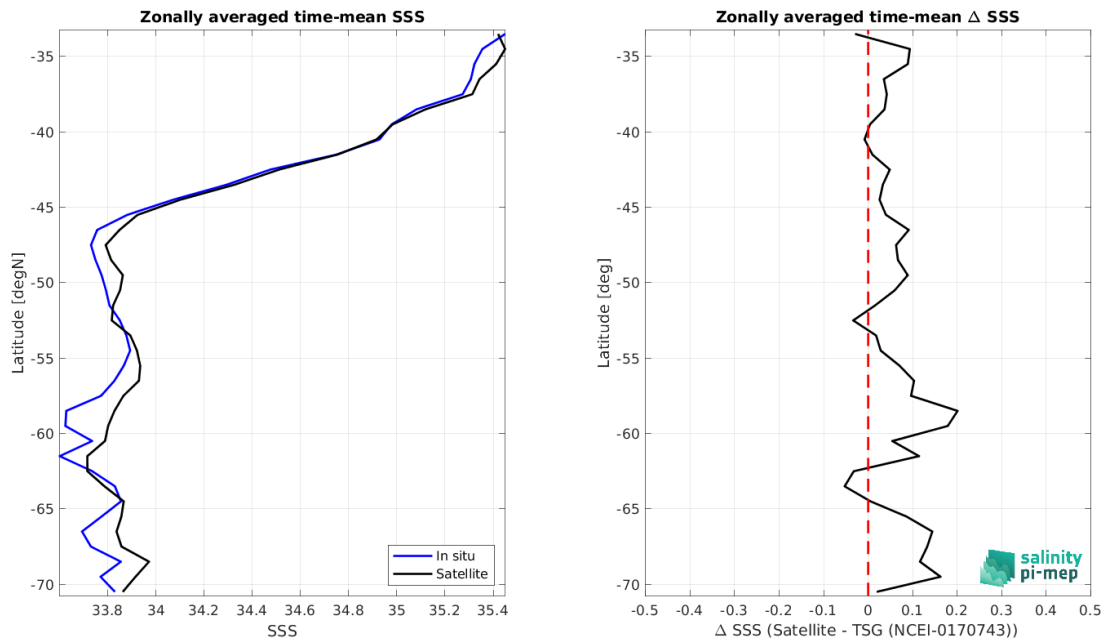
Figure 9: Left panel: Zonal mean SSS from SMOS SSS L4 v1 - Daily (CMEMS-CNR) satellite product (black) and from TSG (NCEI-0170743) (blue). Right panel: Zonal mean of \Delta SSS (Satellite - TSG (NCEI-0170743)) for all the collected Pi-MEP match-up pairs estimated over the full satellite product period.
