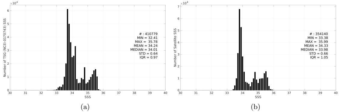
Figure 3: Histograms of SSS from TSG (NCEI-0170743) (a) and SMOS SSS L4 v1 - Daily (CMEMS-CNR) (b) considering all match-up pairs per bins of 0.1 over the Global Ocean Pi-MEP region and for the full satellite product period.
