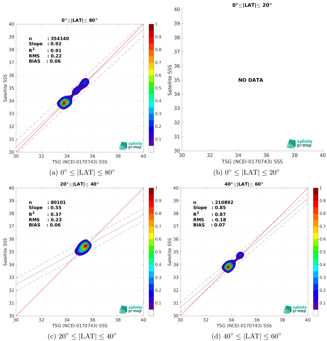
Figure 10: Contour maps of the concentration of SMOS SSS L4 v1 - Daily (CMEMS-CNR) SSS (y-axis) versus TSG (NCEI-0170743) SSS (x-axis) at match-up pairs for different latitude bands. For each plot, the red line shows x=y . The black thin and dashed lines indicate a linear fit through the data cloud and the \pm 95\% confidence levels, respectively. The number match-up pairs n , the slope and R^2 coefficient of the linear fit, the root mean square (RMS) and the mean bias between satellite and in situ data are indicated for each latitude band in each plots.
