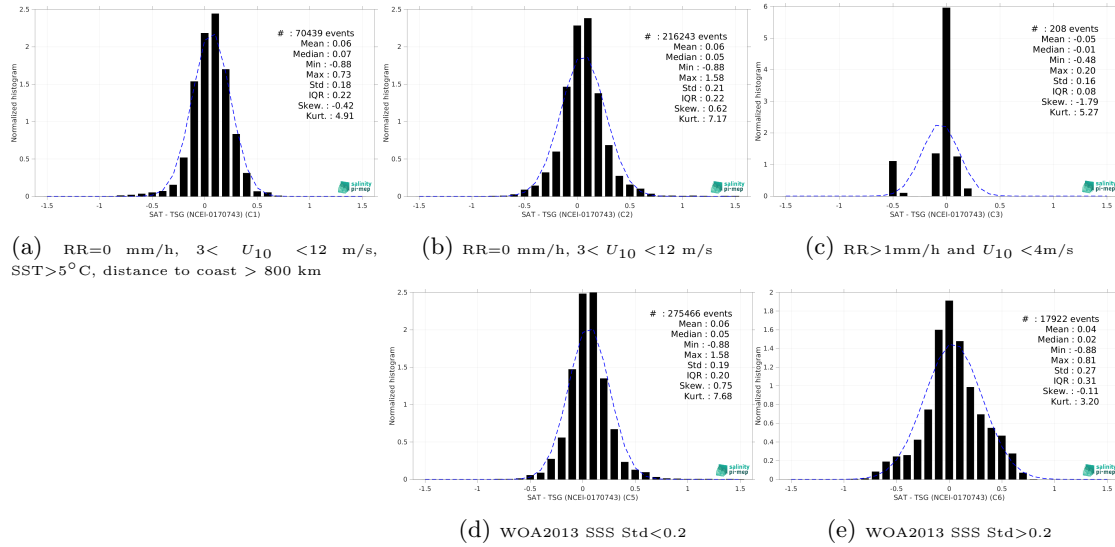
Figure 15: Normalized histogram of \Delta\text{SSS} (SMOS SSS L4 v1 - Daily (CMEMS-CNR) - TSG (NCEI-0170743)) for 5 different subdatasets corresponding to: RR=0 mm/h, 3 < U_{10} < 12 m/s, SST >5^{\circ}\text{C} , distance to coast > 800 km (a), RR=0 mm/h, 3 < U_{10} < 12 m/s (b), RR>1\text{mm/h} and U_{10} < 4\text{m/s} (c), WOA2013 SSS Std <0.2 (d), WOA2013 SSS Std >0.2 (e).
