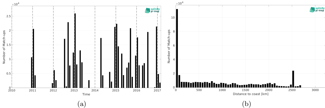
Figure 2: Number of match-ups between TSG (NCEI-0170743) and SMOS SSS L4 v1 - Daily (CMEMS-CNR) SSS as a function of time (a) and as function of the distance to coast (b) over the Global Ocean Pi-MEP region and for the full satellite product period.
