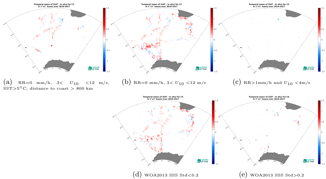
Figure 14: Temporal mean gridded over spatial boxes of size 1^\circ \times 1^\circ of \Delta SSS (SMOS SSS L4 v1 - Daily (CMEMS-CNR) - TSG (NCEI-0170743)) for 5 different subdatasets corresponding to:RR=0 mm/h, 3 < U_{10} < 12 m/s, SST >5^\circ\text{C} , distance to coast > 800 km (a), RR=0 mm/h, 3 < U_{10} < 12 m/s (b), RR >1 mm/h and U_{10} < 4 m/s (c), WOA2013 SSS Std <0.2 (d), WOA2013 SSS Std >0.2 (e).
