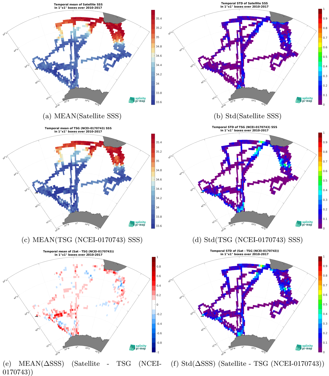
Figure 7: Temporal mean (left) and Std (right) of SSS from SMOS SSS L4 v1 - Daily (CMEMS-CNR) (top), TSG (NCEI-0170743) (middle), and of \Delta SSS (Satellite - TSG (NCEI-0170743)). Only match-up pairs are used to generate these maps.
