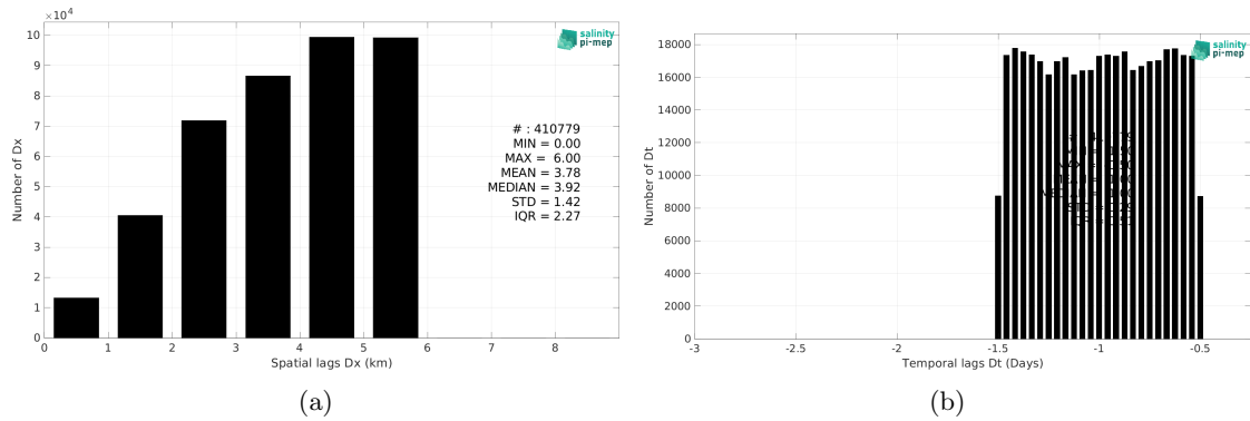
Figure 6: Histograms of the spatial (a) and temporal (b) lags between the location/time of the TSG (NCEI-0170743) measurement and the date of the corresponding SMOS SSS L4 v1 - Daily (CMEMS-CNR) SSS pixel.
