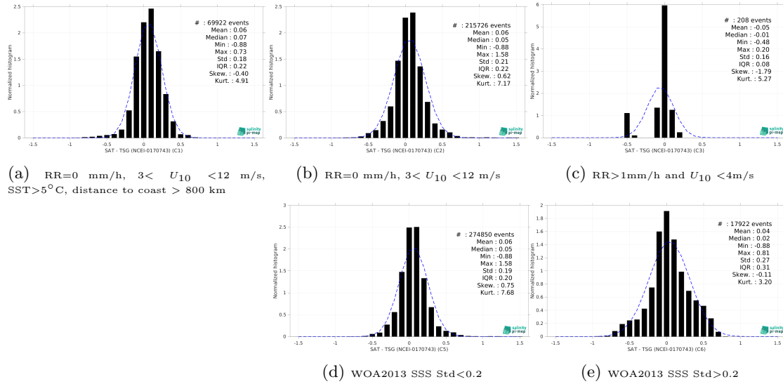
Figure 15: Normalized histogram of \Delta SSS (SMOS SSS L4 v1 - Daily (CMEMS-CNR) - TSG (NCEI-0170743)) for 5 different subdatasets corresponding to: RR=0 mm/h, 3 < U_{10} < 12 m/s, SST>5°C, distance to coast > 800 km (a), RR=0 mm/h, 3 < U_{10} < 12 m/s (b), RR>1mm/h and U_{10} < 4 m/s (c), WOA2013 SSS Std<0.2 (d), WOA2013 SSS Std>0.2 (e).
