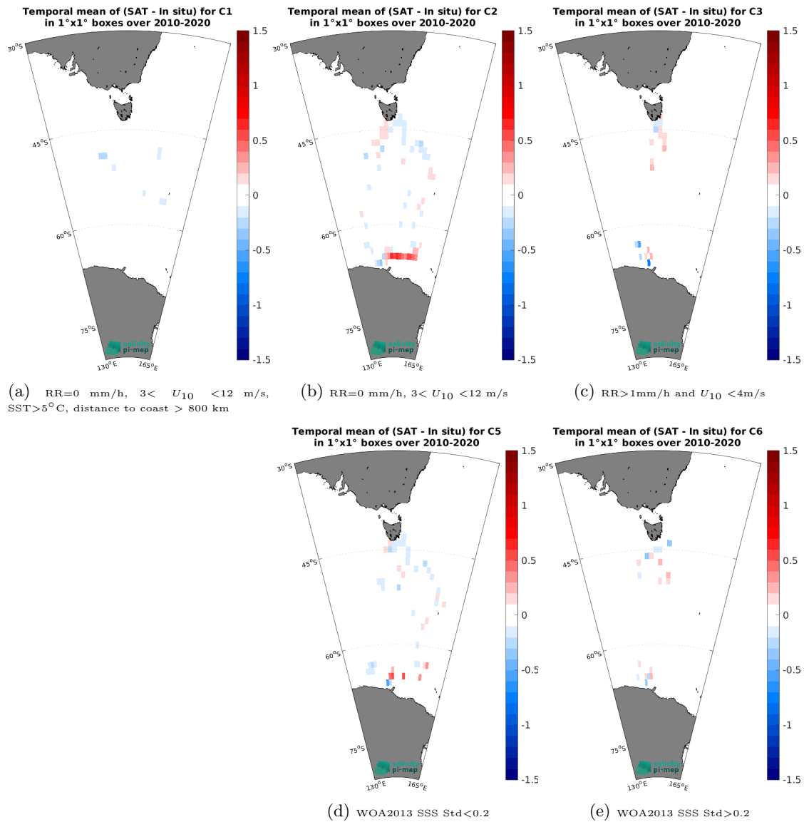
Figure 14: Temporal mean gridded over spatial boxes of size 1°x1° of \Delta SSS (SMOS SSS L4 v1 - Daily (CMEMS-CNR) - TSG (LEGOS-Survostral)) for 5 different subdatasets corresponding to:RR=0 mm/h, 3 < U_{10} < 12 m/s, SST>5°C, distance to coast > 800 km (a), RR=0 mm/h, 3 < U_{10} < 12 m/s (b), RR>1mm/h and U_{10} < 4 m/s (c), WOA2013 SSS Std<0.2 (d), WOA2013 SSS Std>0.2 (e).
