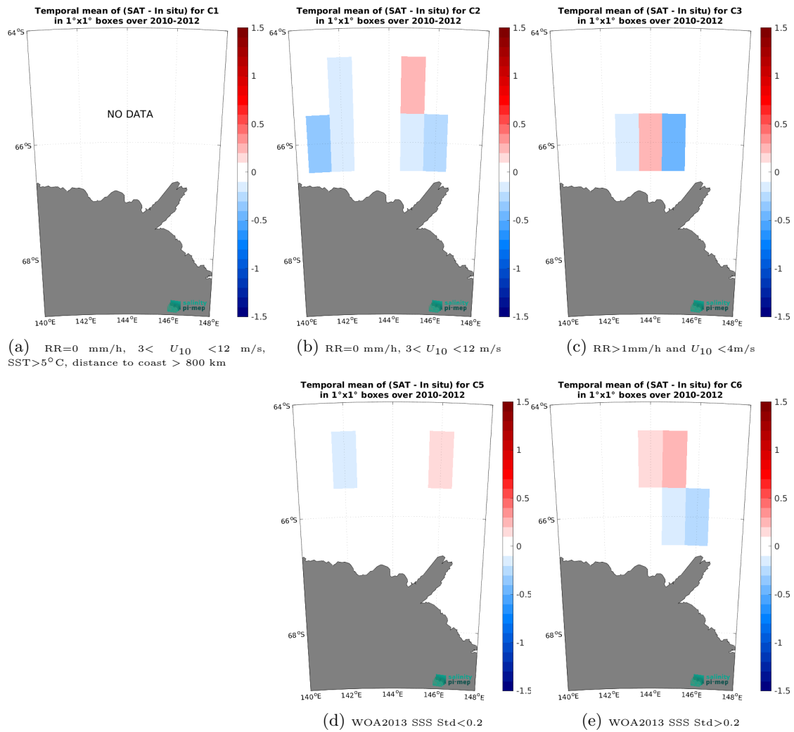
Figure 14: Temporal mean gridded over spatial boxes of size 1^\circ \times 1^\circ of \Delta SSS (SMOS SSS L4 v1 - Daily (CMEMS-CNR) - TSG (LEGOS-Surv-Adel)) for 5 different subdatasets corresponding to: RR=0 mm/h, 3 < U_{10} < 12 m/s, SST>5°C, distance to coast > 800 km (a), RR=0 mm/h, 3 < U_{10} < 12 m/s (b), RR>1mm/h and U_{10} < 4 m/s (c), WOA2013 SSS Std<0.2 (d), WOA2013 SSS Std>0.2 (e).
