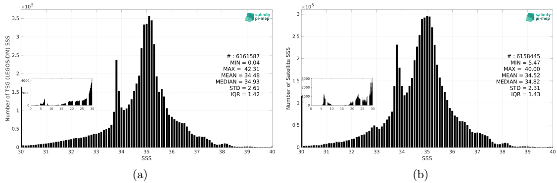
Figure 3: Histograms of SSS from TSG (LEGOS-DM) (a) and SMOS SSS L4 v1 - Daily (CMEMS-CNR) (b) considering all match-up pairs per bins of 0.1 over the Global Ocean Pi-MEP region and for the full satellite product period.
