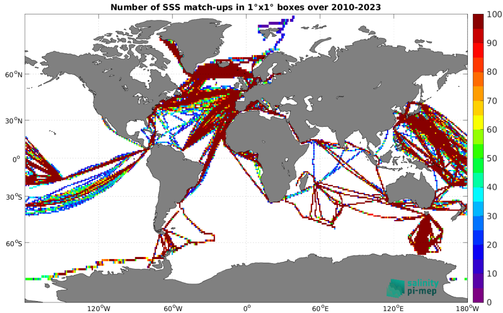
Figure 5: Number of SSS match-ups between TSG (LEGOS-DM) SSS and the SMOS SSS L4 v1 - Daily (CMEMS-CNR) SSS product for the Global Ocean Pi-MEP region over 1^\circ \times 1^\circ boxes and for the full satellite product period.
