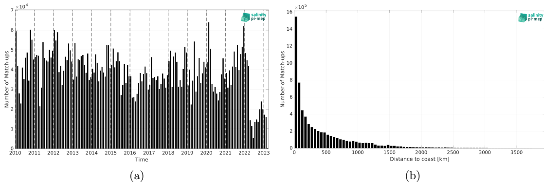
Figure 2: Number of match-ups between TSG (LEGOS-DM) and SMOS SSS L4 v1 - Daily (CMEMS-CNR) SSS as a function of time (a) and as function of the distance to coast (b) over the Global Ocean Pi-MEP region and for the full satellite product period.
