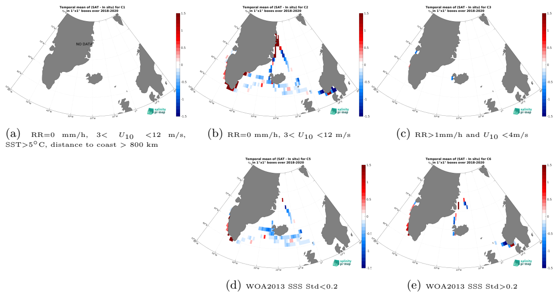
Figure 14: Temporal mean gridded over spatial boxes of size 1^\circ \times 1^\circ of \Delta SSS (SMOS SSS L4 v1 - Daily (CMEMS-CNR) - TSG (Lauge-Koch)) for 5 different subdatasets corresponding to:RR=0 mm/h, 3 < U_{10} < 12 m/s, SST > 5^\circ\text{C} , distance to coast > 800 km (a), RR=0 mm/h, 3 < U_{10} < 12 m/s (b), RR > 1 mm/h and U_{10} < 4 m/s (c), WOA2013 SSS Std < 0.2 (d), WOA2013 SSS Std > 0.2 (e).
