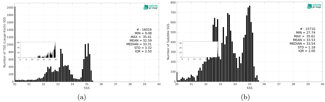
Figure 3: Histograms of SSS from TSG (Lauge-Koch) (a) and SMOS SSS L4 v1 - Daily (CMEMS-CNR) (b) considering all match-up pairs per bins of 0.1 over the Global Ocean Pi-MEP region and for the full satellite product period.
