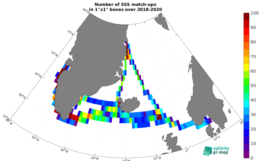
Figure 5: Number of SSS match-ups between TSG (Lauge-Koch) SSS and the SMOS SSS L4 v1 - Daily (CMEMS-CNR) SSS product for the Global Ocean Pi-MEP region over 1^\circ \times 1^\circ boxes and for the full satellite product period.
