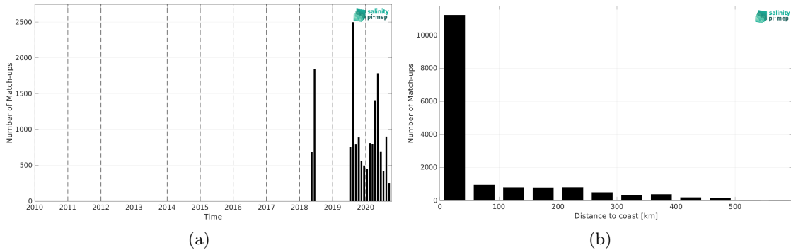
Figure 2: Number of match-ups between TSG (Lauge-Koch) and SMOS SSS L4 v1 - Daily (CMEMS-CNR) SSS as a function of time (a) and as function of the distance to coast (b) over the Global Ocean Pi-MEP region and for the full satellite product period.
