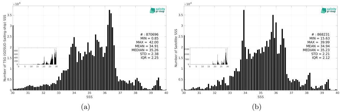
Figure 3: Histograms of SSS from TSG (GOSUD-Sailing-ship) (a) and SMOS SSS L4 v1 - Daily (CMEMS-CNR) (b) considering all match-up pairs per bins of 0.1 over the Global Ocean Pi-MEP region and for the full satellite product period.
