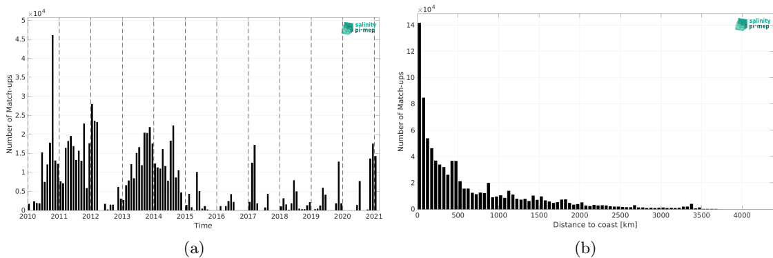
Figure 2: Number of match-ups between TSG (GOSUD-Sailing-ship) and SMOS SSS L4 v1 - Daily (CMEMS-CNR) SSS as a function of time (a) and as function of the distance to coast (b) over the Global Ocean Pi-MEP region and for the full satellite product period.
