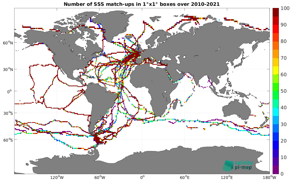
Figure 5: Number of SSS match-ups between TSG (GOSUD-Sailing-ship) SSS and the SMOS SSS L4 v1 - Daily (CMEMS-CNR) SSS product for the Global Ocean Pi-MEP region over 1^\circ \times 1^\circ boxes and for the full satellite product period.
