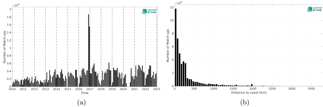
Figure 2: Number of match-ups between TSG (GOSUD-Research-vessel) and SMOS SSS L4 v1 - Daily (CMEMS-CNR) SSS as a function of time (a) and as function of the distance to coast (b) over the Global Ocean Pi-MEP region and for the full satellite product period.
