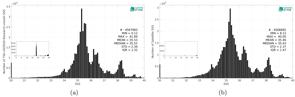
Figure 3: Histograms of SSS from TSG (GOSUD-Research-vessel) (a) and SMOS SSS L4 v1 - Daily (CMEMS-CNR) (b) considering all match-up pairs per bins of 0.1 over the Global Ocean Pi-MEP region and for the full satellite product period.
