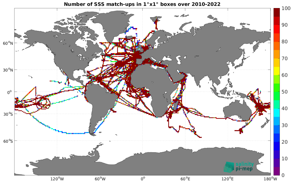
Figure 5: Number of SSS match-ups between TSG (GOSUD-Research-vessel) SSS and the SMOS SSS L4 v1 - Daily (CMEMS-CNR) SSS product for the Global Ocean Pi-MEP region over 1^\circ \times 1^\circ boxes and for the full satellite product period.
