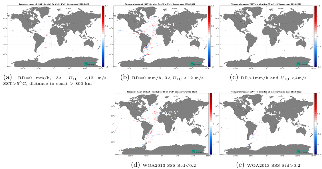
Figure 14: Temporal mean gridded over spatial boxes of size 1^\circ \times 1^\circ of \Delta\text{SSS} (SMOS SSS L4 v1 - Daily (CMEMS-CNR) - TSG (CSIC-UTM)) for 5 different subdatasets corresponding to:RR=0 mm/h, 3 < U_{10} < 12 m/s, SST > 5^\circ\text{C} , distance to coast > 800 km (a), RR=0 mm/h, 3 < U_{10} < 12 m/s (b), RR > 1 mm/h and U_{10} < 4 m/s (c), WOA2013 SSS Std < 0.2 (d), WOA2013 SSS Std > 0.2 (e).
