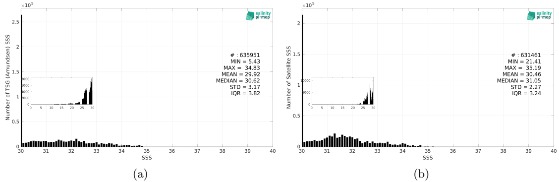
Figure 3: Histograms of SSS from TSG (Amundsen) (a) and SMOS SSS L4 v1 - Daily (CMEMS-CNR) (b) considering all match-up pairs per bins of 0.1 over the Global Ocean Pi-MEP region and for the full satellite product period.
