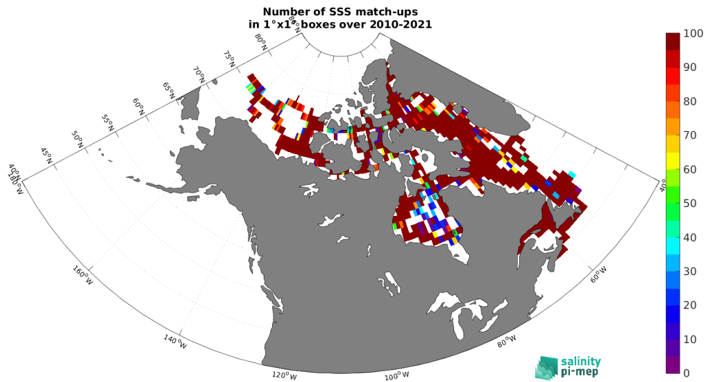
Figure 5: Number of SSS match-ups between TSG (Amundsen) SSS and the SMOS SSS L4 v1 - Daily (CMEMS-CNR) SSS product for the Global Ocean Pi-MEP region over 1^\circ \times 1^\circ boxes and for the full satellite product period.
