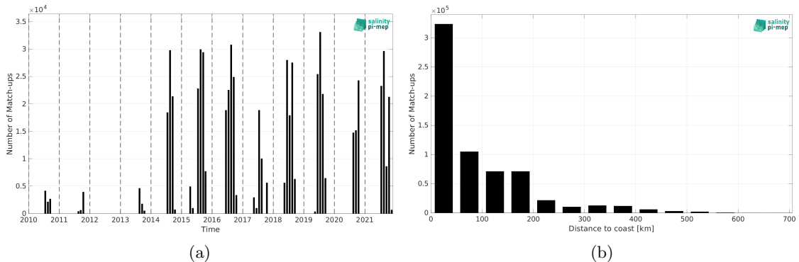
Figure 2: Number of match-ups between TSG (Amundsen) and SMOS SSS L4 v1 - Daily (CMEMS-CNR) SSS as a function of time (a) and as function of the distance to coast (b) over the Global Ocean Pi-MEP region and for the full satellite product period.
