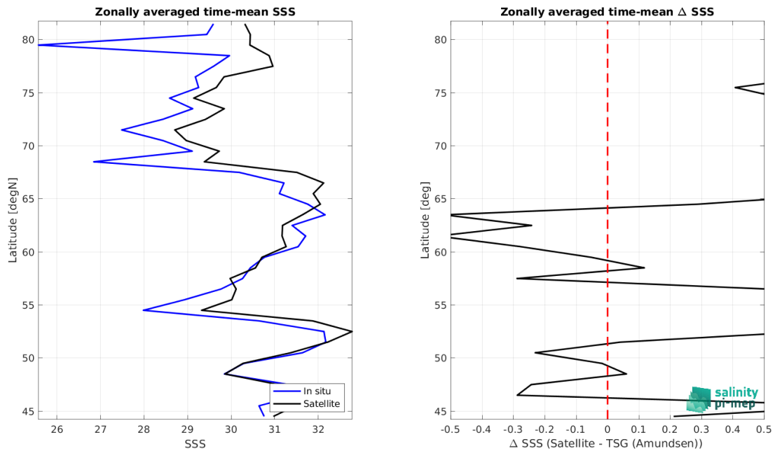
Figure 9: Left panel: Zonal mean SSS from SMOS SSS L4 v1 - Daily (CMEMS-CNR) satellite product (black) and from TSG (Amundsen) (blue). Right panel: Zonal mean of \Delta SSS (Satellite - TSG (Amundsen)) for all the collected Pi-MEP match-up pairs estimated over the full satellite product period.
