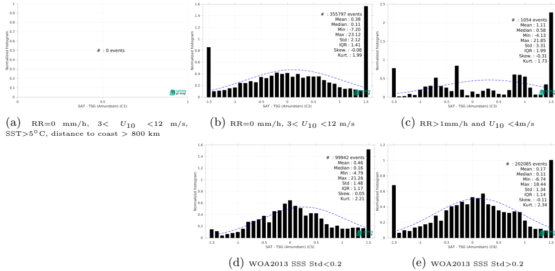
Figure 15: Normalized histogram of \Delta SSS (SMOS SSS L4 v1 - Daily (CMEMS-CNR) - TSG (Amundsen)) for 5 different subdatasets corresponding to: RR=0 mm/h, 3 < U_{10} < 12 m/s, SST>5°C, distance to coast > 800 km (a), RR=0 mm/h, 3 < U_{10} < 12 m/s (b), RR>1mm/h and U_{10} < 4 m/s (c), WOA2013 SSS Std<0.2 (d), WOA2013 SSS Std>0.2 (e).
