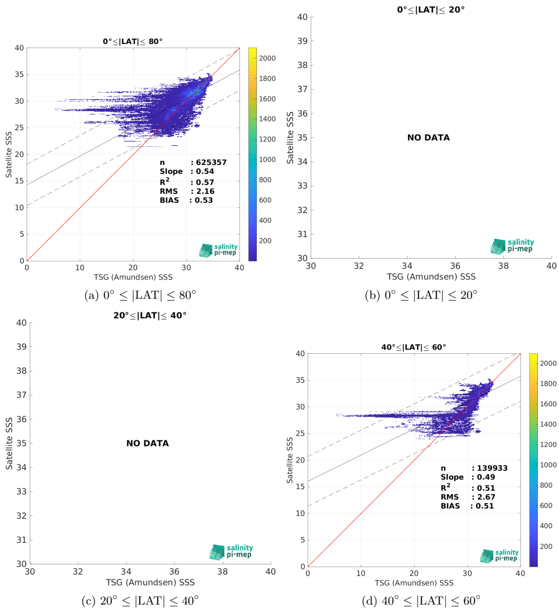
Figure 10: Contour maps of the concentration of SMOS SSS L4 v1 - Daily (CMEMS-CNR) SSS (y-axis) versus TSG (Amundsen) SSS (x-axis) at match-up pairs for different latitude bands. For each plot, the red line shows x=y . The black thin and dashed lines indicate a linear fit through the data cloud and the \pm 95\% confidence levels, respectively. The number match-up pairs n , the slope and R^2 coefficient of the linear fit, the root mean square (RMS) and the mean bias between satellite and in situ data are indicated for each latitude band in each plots.
