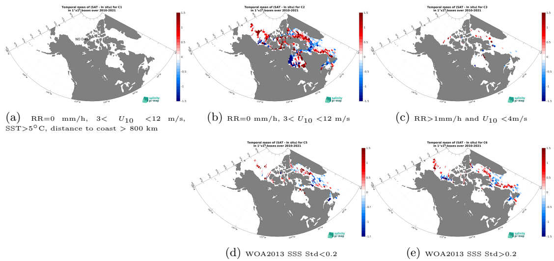
Figure 14: Temporal mean gridded over spatial boxes of size 1^\circ \times 1^\circ of \Delta SSS (SMOS SSS L4 v1 - Daily (CMEMS-CNR) - TSG (Amundsen)) for 5 different subdatasets corresponding to:RR=0 mm/h, 3 < U_{10} < 12 m/s, SST >5^\circ C, distance to coast > 800 km (a), RR=0 mm/h, 3 < U_{10} < 12 m/s (b), RR >1 mm/h and U_{10} < 4 m/s (c), WOA2013 SSS Std <0.2 (d), WOA2013 SSS Std >0.2 (e).
