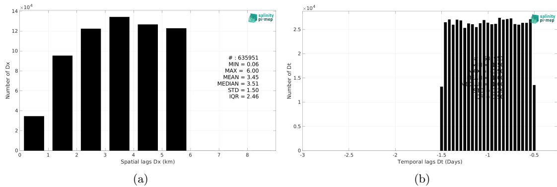
Figure 6: Histograms of the spatial (a) and temporal (b) lags between the location/time of the TSG (Amundsen) measurement and the date of the corresponding SMOS SSS L4 v1 - Daily (CMEMS-CNR) SSS pixel.
