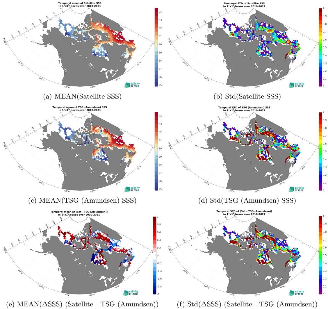
Figure 7: Temporal mean (left) and Std (right) of SSS from SMOS SSS L4 v1 - Daily (CMEMS-CNR) (top), TSG (Amundsen) (middle), and of \Delta SSS (Satellite - TSG (Amundsen)). Only match-up pairs are used to generate these maps.
