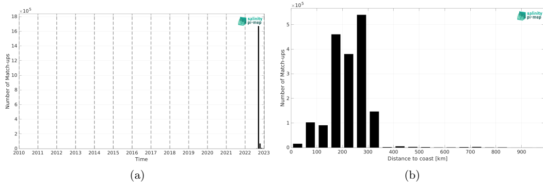
Figure 2: Number of match-ups between SASSIE and SMOS SSS L4 v1 - Daily (CMEMS-CNR) SSS as a function of time (a) and as function of the distance to coast (b) over the Global Ocean Pi-MEP region and for the full satellite product period.
