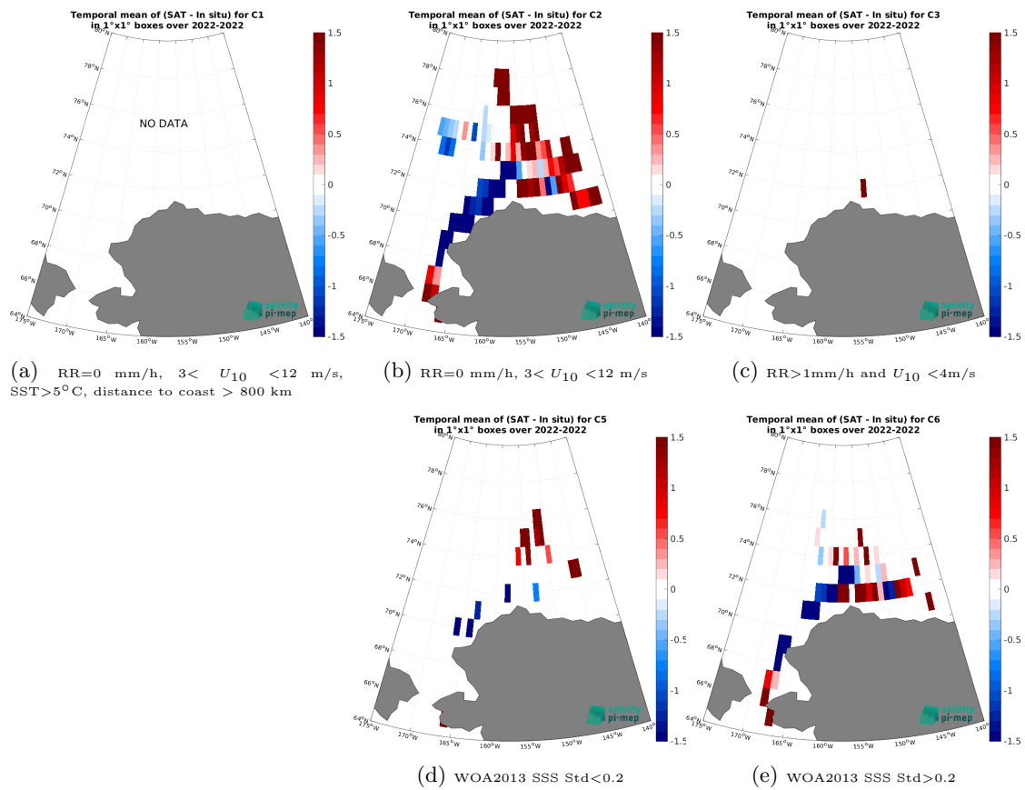
Figure 14: Temporal mean gridded over spatial boxes of size 1^\circ \times 1^\circ of \Delta SSS (SMOS SSS L4 v1 - Daily (CMEMS-CNR) - SASSIE) for 5 different subdatasets corresponding to:RR=0 mm/h, 3 < U_{10} < 12 m/s, SST>5°C, distance to coast > 800 km (a), RR=0 mm/h, 3 < U_{10} < 12 m/s (b), RR>1mm/h and U_{10} < 4 m/s (c), WOA2013 SSS Std<0.2 (d), WOA2013 SSS Std>0.2 (e).
