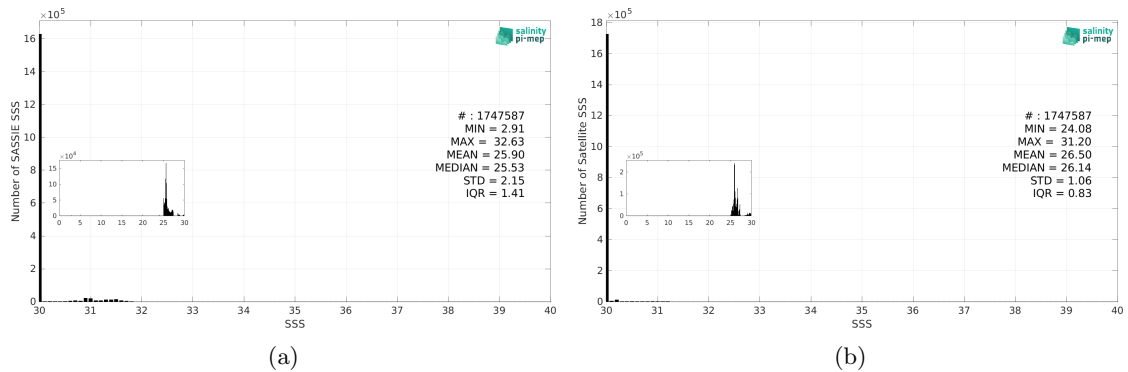
Figure 3: Histograms of SSS from SASSIE (a) and SMOS SSS L4 v1 - Daily (CMEMS-CNR) (b) considering all match-up pairs per bins of 0.1 over the Global Ocean Pi-MEP region and for the full satellite product period.
