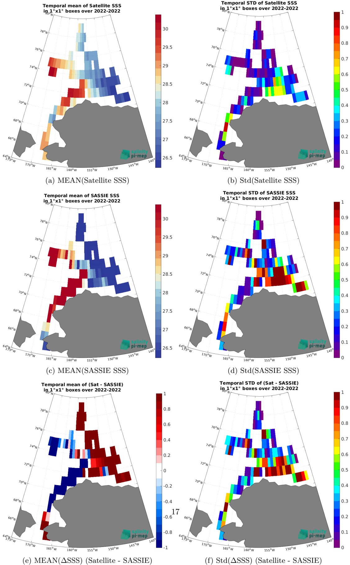
Figure 7: Temporal mean (left) and Std (right) of SSS from SMOS SSS L4 v1 - Daily (CMEMS-CNR) (top), SASSIE (middle), and of \Delta\text{SSS} (Satellite - SASSIE). Only match-up pairs are used to generate these maps.
