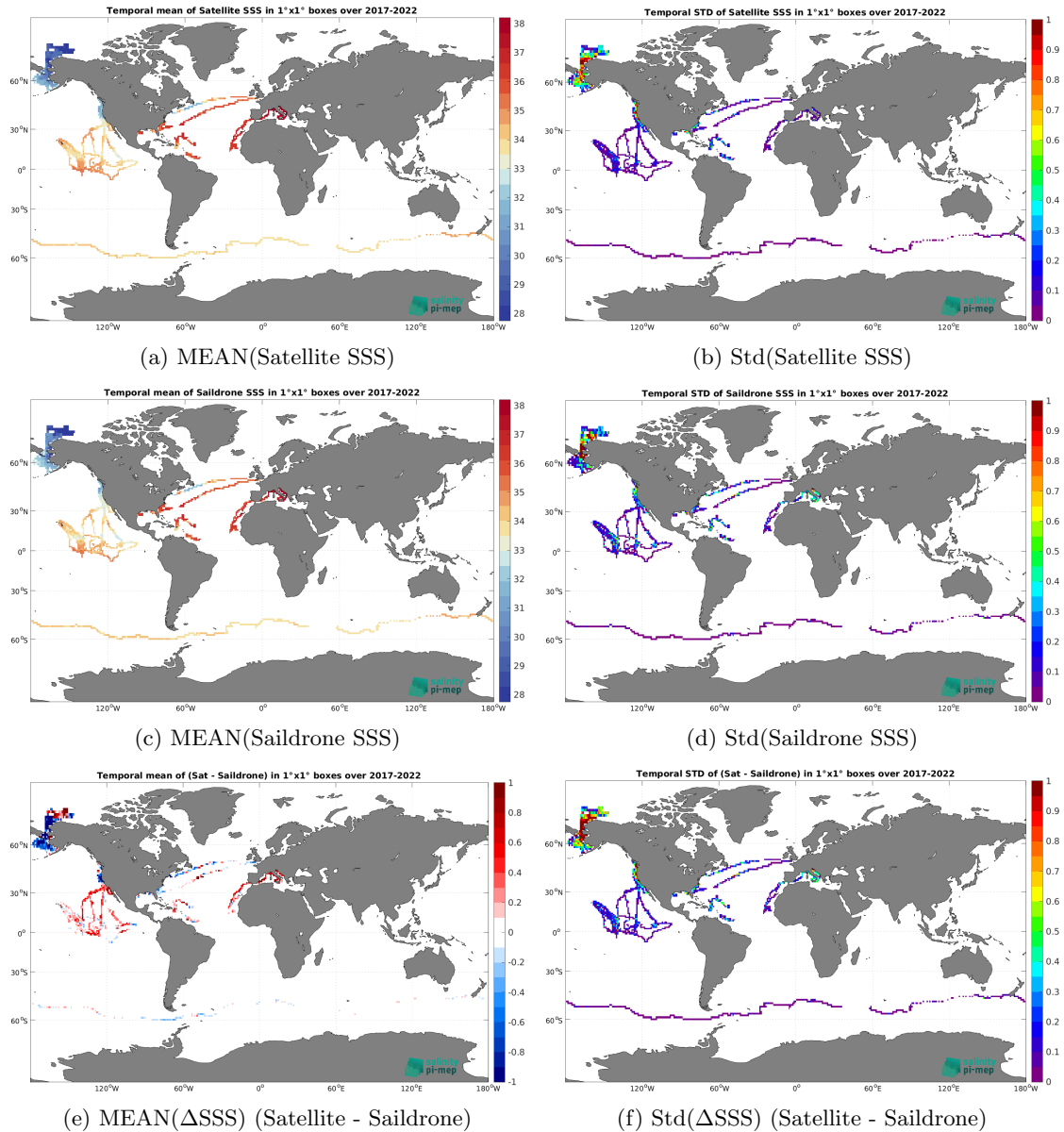
Figure 7: Temporal mean (left) and Std (right) of SSS from SMOS SSS L4 v1 - Daily (CMEMS-CNR) (top), Saildrone (middle), and of \Delta SSS (Satellite - Saildrone). Only match-up pairs are used to generate these maps.
