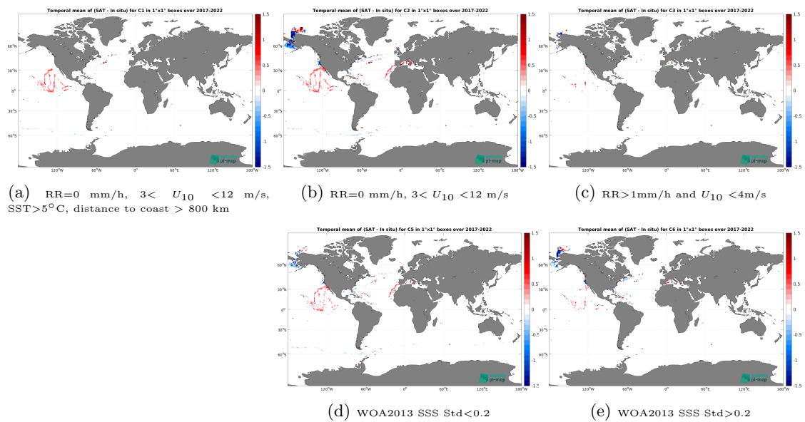
Figure 14: Temporal mean gridded over spatial boxes of size 1^\circ \times 1^\circ of \Delta SSS (SMOS SSS L4 v1 - Daily (CMEMS-CNR) - Saildrone) for 5 different subdatasets corresponding to:RR=0 mm/h, 3 < U_{10} < 12 m/s, SST > 5^\circ\text{C} , distance to coast > 800 km (a), RR=0 mm/h, 3 < U_{10} < 12 m/s (b), RR > 1 mm/h and U_{10} < 4 m/s (c), WOA2013 SSS Std < 0.2 (d), WOA2013 SSS Std > 0.2 (e).
