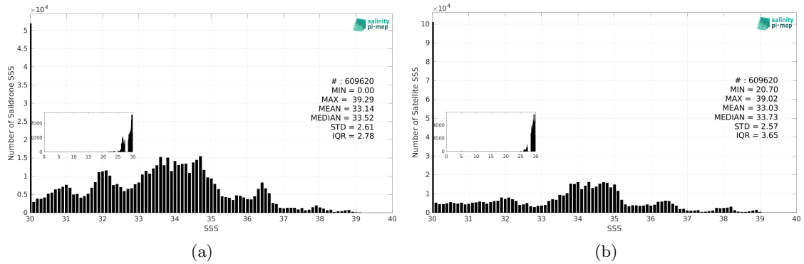
Figure 3: Histograms of SSS from Saildrone (a) and SMOS SSS L4 v1 - Daily (CMEMS-CNR) (b) considering all match-up pairs per bins of 0.1 over the Global Ocean Pi-MEP region and for the full satellite product period.
