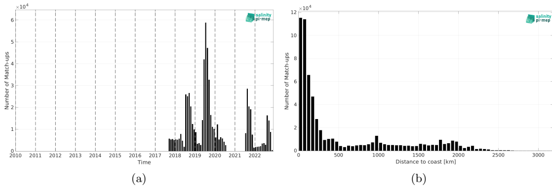
Figure 2: Number of match-ups between Saildrone and SMOS SSS L4 v1 - Daily (CMEMS-CNR) SSS as a function of time (a) and as function of the distance to coast (b) over the Global Ocean Pi-MEP region and for the full satellite product period.
