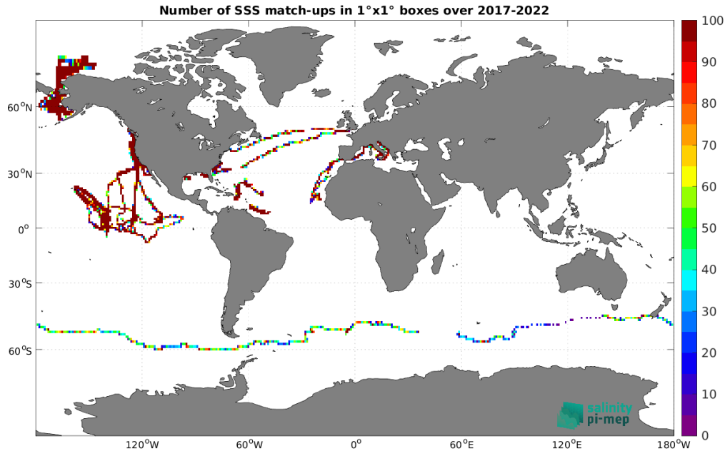
Figure 5: Number of SSS match-ups between Saildrone SSS and the SMOS SSS L4 v1 - Daily (CMEMS-CNR) SSS product for the Global Ocean Pi-MEP region over 1^\circ \times 1^\circ boxes and for the full satellite product period.
