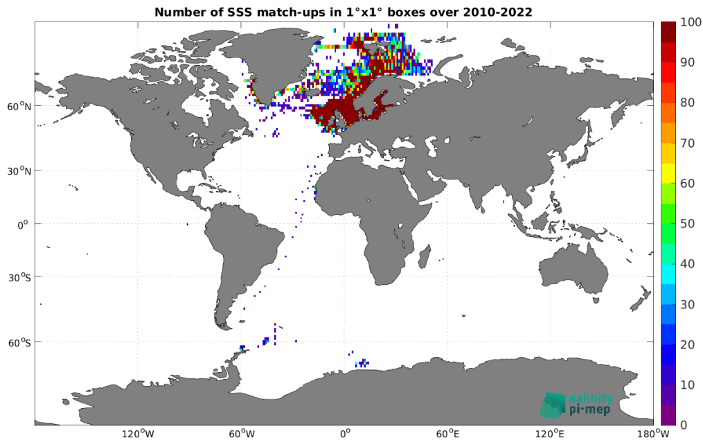
Figure 5: Number of SSS match-ups between ICES SSS and the SMOS SSS L4 v1 - Daily (CMEMS-CNR) SSS product for the Global Ocean Pi-MEP region over 1^\circ \times 1^\circ boxes and for the full satellite product period.
