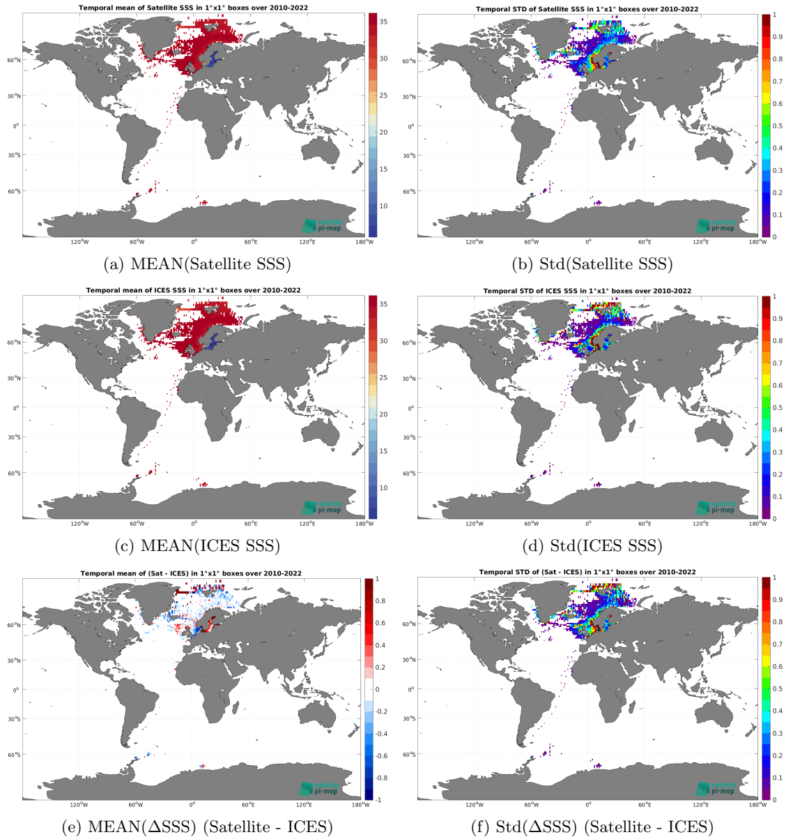
Figure 7: Temporal mean (left) and Std (right) of SSS from SMOS SSS L4 v1 - Daily (CMEMS-CNR) (top), ICES (middle), and of \Delta SSS (Satellite - ICES). Only match-up pairs are used to generate these maps.
