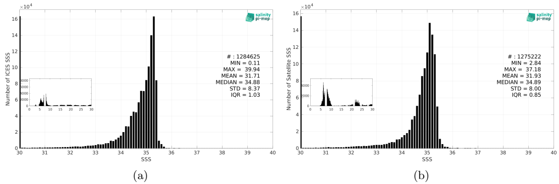
Figure 3: Histograms of SSS from ICES (a) and SMOS SSS L4 v1 - Daily (CMEMS-CNR) (b) considering all match-up pairs per bins of 0.1 over the Global Ocean Pi-MEP region and for the full satellite product period.
