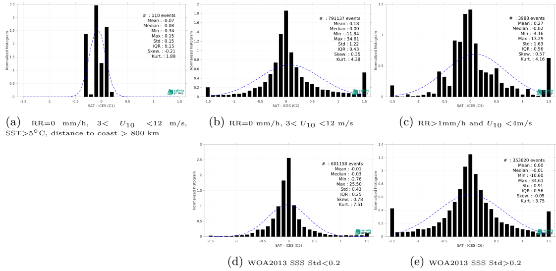
Figure 15: Normalized histogram of \Delta SSS (SMOS SSS L4 v1 - Daily (CMEMS-CNR) - ICES) for 5 different subdatasets corresponding to: RR=0 mm/h, 3 < U_{10} < 12 m/s, SST > 5°C, distance to coast > 800 km (a), RR=0 mm/h, 3 < U_{10} < 12 m/s (b), RR > 1mm/h and U_{10} < 4 m/s (c), WOA2013 SSS Std < 0.2 (d), WOA2013 SSS Std > 0.2 (e).
