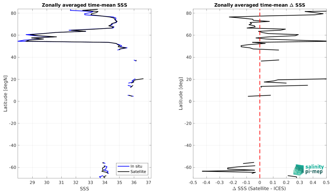
Figure 9: Left panel: Zonal mean SSS from SMOS SSS L4 v1 - Daily (CMEMS-CNR) satellite product (black) and from ICES (blue). Right panel: Zonal mean of \Delta SSS (Satellite - ICES) for all the collected Pi-MEP match-up pairs estimated over the full satellite product period.
