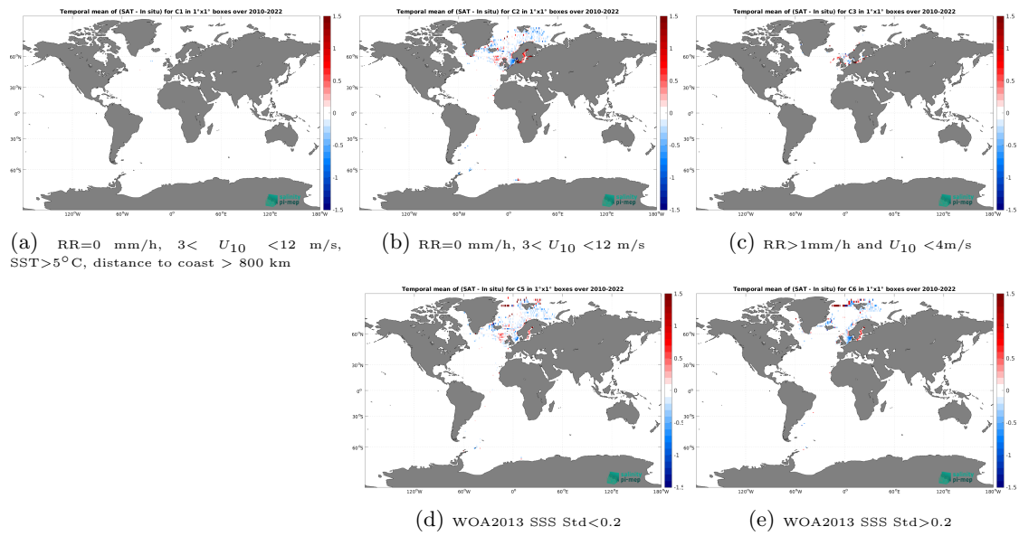
Figure 14: Temporal mean gridded over spatial boxes of size 1^\circ \times 1^\circ of \Delta SSS (SMOS SSS L4 v1 - Daily (CMEMS-CNR) - ICES) for 5 different subdatasets corresponding to:RR=0 mm/h, 3 < U_{10} < 12 m/s, SST > 5^\circ\text{C} , distance to coast > 800 km (a), RR=0 mm/h, 3 < U_{10} < 12 m/s (b), RR > 1 mm/h and U_{10} < 4 m/s (c), WOA2013 SSS Std < 0.2 (d), WOA2013 SSS Std > 0.2 (e).
