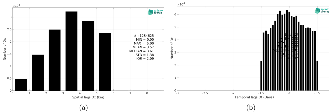
Figure 6: Histograms of the spatial (a) and temporal (b) lags between the location/time of the ICES measurement and the date of the corresponding SMOS SSS L4 v1 - Daily (CMEMS-CNR) SSS pixel.
