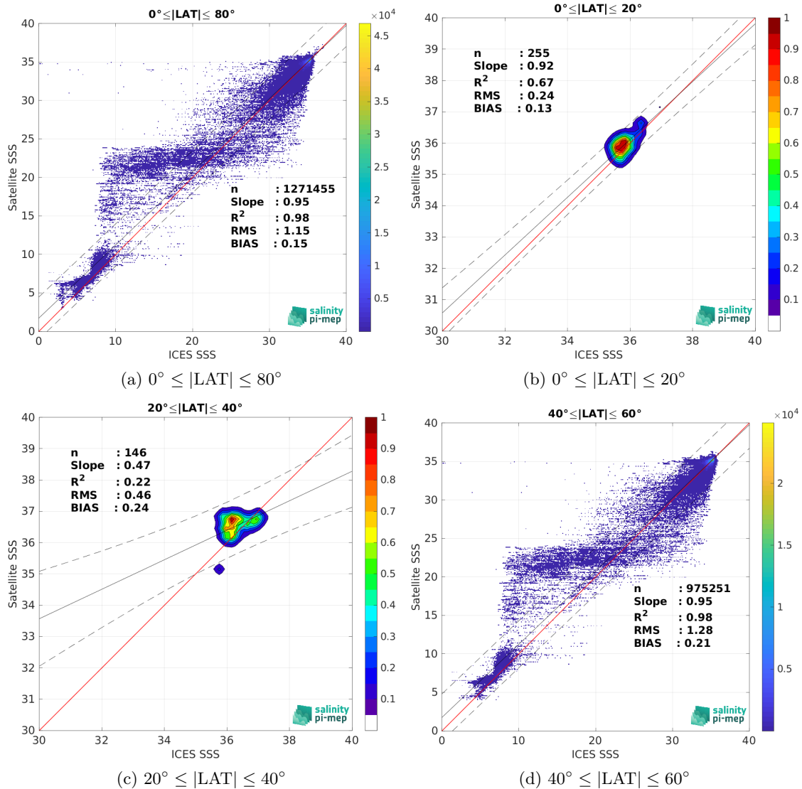
Figure 10: Contour maps of the concentration of SMOS SSS L4 v1 - Daily (CMEMS-CNR) SSS (y-axis) versus ICES SSS (x-axis) at match-up pairs for different latitude bands. For each plot, the red line shows x=y . The black thin and dashed lines indicate a linear fit through the data cloud and the \pm 95\% confidence levels, respectively. The number match-up pairs n , the slope and R^2 coefficient of the linear fit, the root mean square (RMS) and the mean bias between satellite and in situ data are indicated for each latitude band in each plots.
