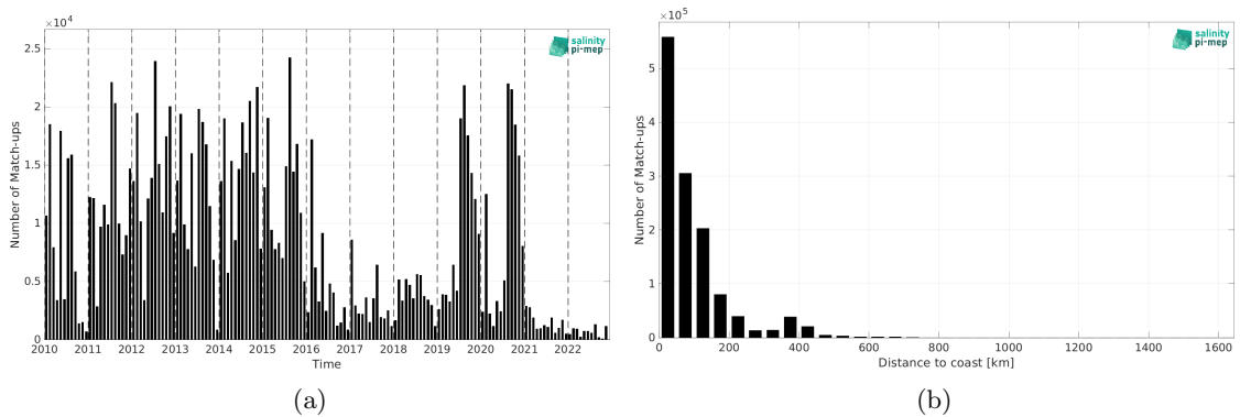
Figure 2: Number of match-ups between ICES and SMOS SSS L4 v1 - Daily (CMEMS-CNR) SSS as a function of time (a) and as function of the distance to coast (b) over the Global Ocean Pi-MEP region and for the full satellite product period.
