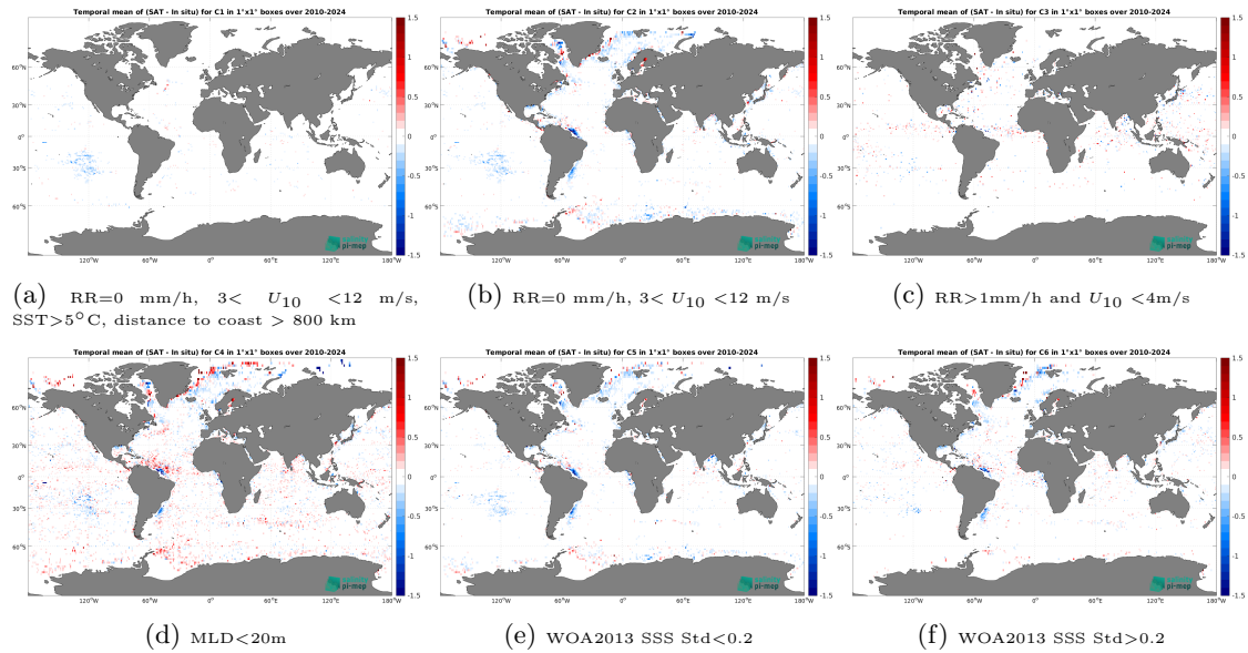
Figure 14: Temporal mean gridded over spatial boxes of size 1^\circ \times 1^\circ of \Delta SSS (SMOS SSS L4 v1 - Daily (CMEMS-CNR) - Argo) for 6 different subdatasets corresponding to:RR=0 mm/h, 3 < U_{10} < 12 m/s, SST >5^\circ C, distance to coast > 800 km (a), RR=0 mm/h, 3 < U_{10} < 12 m/s (b), RR >1 mm/h and U_{10} < 4 m/s (c),MLD <20 m (d),WOA2013 SSS Std <0.2 (e),WOA2013 SSS Std >0.2 (f).
