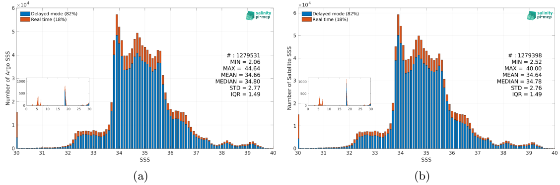
Figure 3: Histograms of SSS from Argo (a) and SMOS SSS L4 v1 - Daily (CMEMS-CNR) (b) considering all match-up pairs per bins of 0.1 over the Global Ocean Pi-MEP region and for the full satellite product period.
