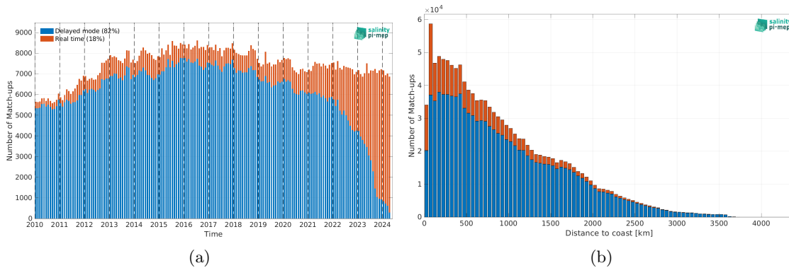
Figure 2: Number of match-ups between Argo and SMOS SSS L4 v1 - Daily (CMEMS-CNR) SSS as a function of time (a) and as function of the distance to coast (b) over the Global Ocean Pi-MEP region and for the full satellite product period.
