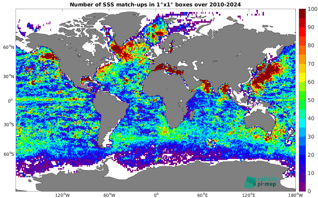
Figure 5: Number of SSS match-ups between Argo SSS and the SMOS SSS L4 v1 - Daily (CMEMS-CNR) SSS product for the Global Ocean Pi-MEP region over 1^\circ \times 1^\circ boxes and for the full satellite product period.
