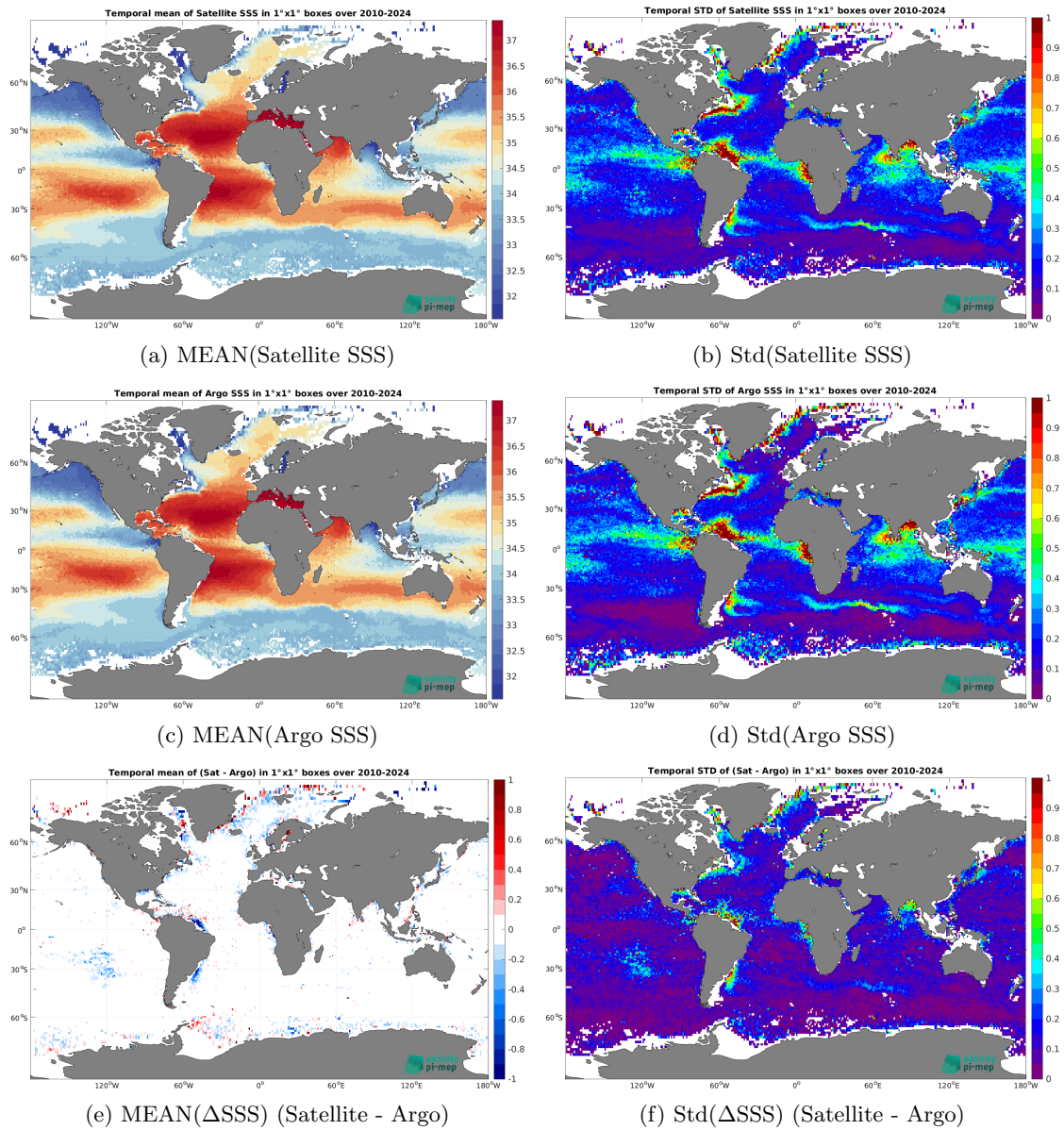
Figure 7: Temporal mean (left) and Std (right) of SSS from SMOS SSS L4 v1 - Daily (CMEMS-CNR) (top), Argo (middle), and of \Delta SSS (Satellite - Argo). Only match-up pairs are used to generate these maps.
