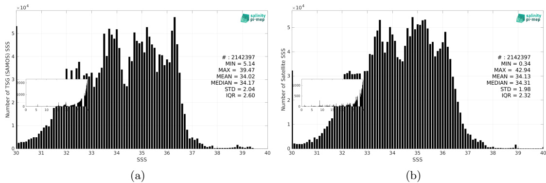
Figure 3: Histograms of SSS from TSG (SAMOS) (a) and SMOS SSS L4 OI v346 - Weekly (CMEMS-CATDS-LOPS) (b) considering all match-up pairs per bins of 0.1 over the Global Ocean Pi-MEP region and for the full satellite product period.
