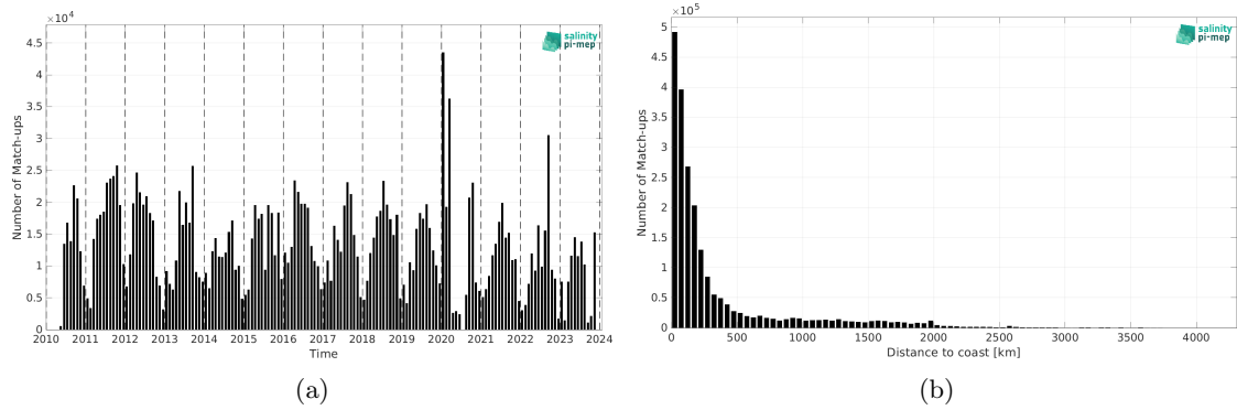
Figure 2: Number of match-ups between TSG (SAMOS) and SMOS SSS L4 OI v346 - Weekly (CMEMS-CATDS-LOPS) SSS as a function of time (a) and as function of the distance to coast (b) over the Global Ocean Pi-MEP region and for the full satellite product period.
