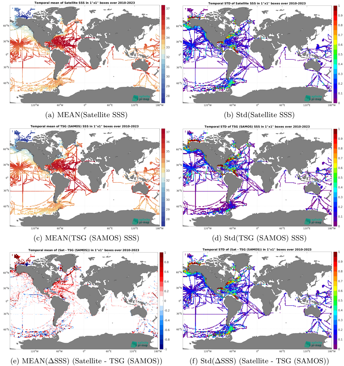
Figure 7: Temporal mean (left) and Std (right) of SSS from SMOS SSS L4 OI v346 - Weekly (CMEMS-CATDS-LOPS) (top), TSG (SAMOS) (middle), and of \Delta SSS (Satellite - TSG (SAMOS)). Only match-up pairs are used to generate these maps.
