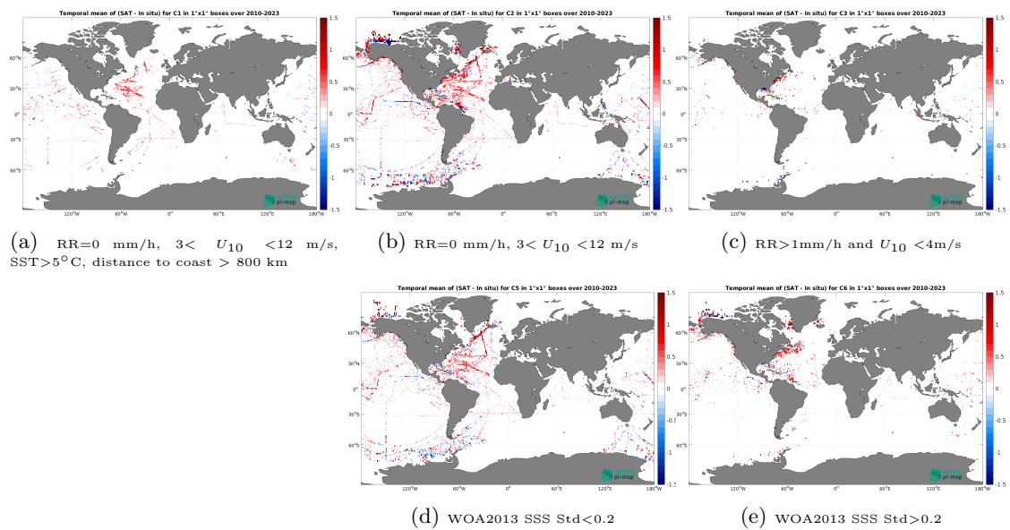
Figure 14: Temporal mean gridded over spatial boxes of size 1^\circ \times 1^\circ of \Delta SSS (SMOS SSS L4 OI v346 - Weekly (CMEMS-CATDS-LOPS) - TSG (SAMOS)) for 5 different subdatasets corresponding to:RR=0 mm/h, 3 < U_{10} < 12 m/s, SST > 5^\circ\text{C} , distance to coast > 800 km (a), RR=0 mm/h, 3 < U_{10} < 12 m/s (b), RR > 1 mm/h and U_{10} < 4 m/s (c), WOA2013 SSS Std < 0.2 (d), WOA2013 SSS Std > 0.2 (e).
