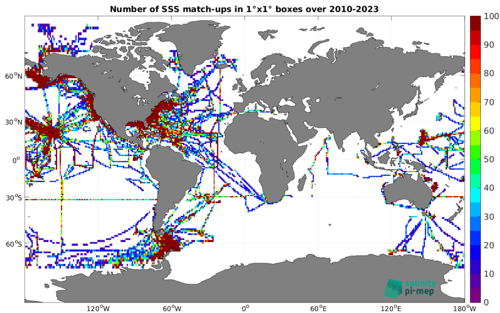
Figure 5: Number of SSS match-ups between TSG (SAMOS) SSS and the SMOS SSS L4 OI v346 - Weekly (CMEMS-CATDS-LOPS) SSS product for the Global Ocean Pi-MEP region over 1^\circ \times 1^\circ boxes and for the full satellite product period.
