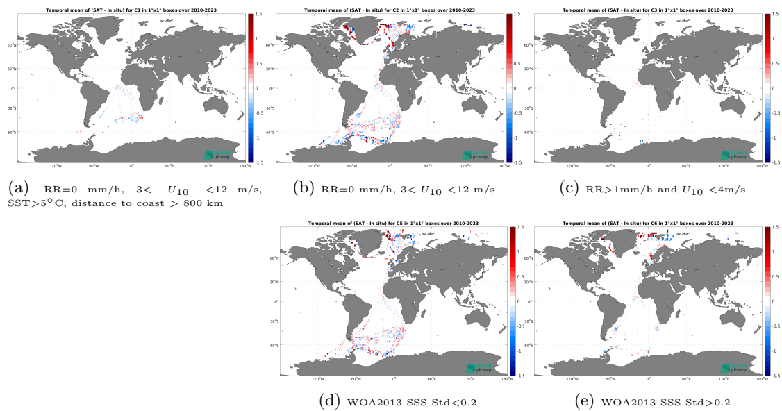
Figure 14: Temporal mean gridded over spatial boxes of size 1^\circ \times 1^\circ of \Delta SSS (SMOS SSS L4 OI v346 - Weekly (CMEMS-CATDS-LOPS) - TSG (Polarstern)) for 5 different subdatasets corresponding to: RR=0 mm/h, 3 < U_{10} < 12 m/s, SST > 5^\circ\text{C} , distance to coast > 800 km (a), RR=0 mm/h, 3 < U_{10} < 12 m/s (b), RR > 1 mm/h and U_{10} < 4 m/s (c), WOA2013 SSS Std < 0.2 (d), WOA2013 SSS Std > 0.2 (e).
