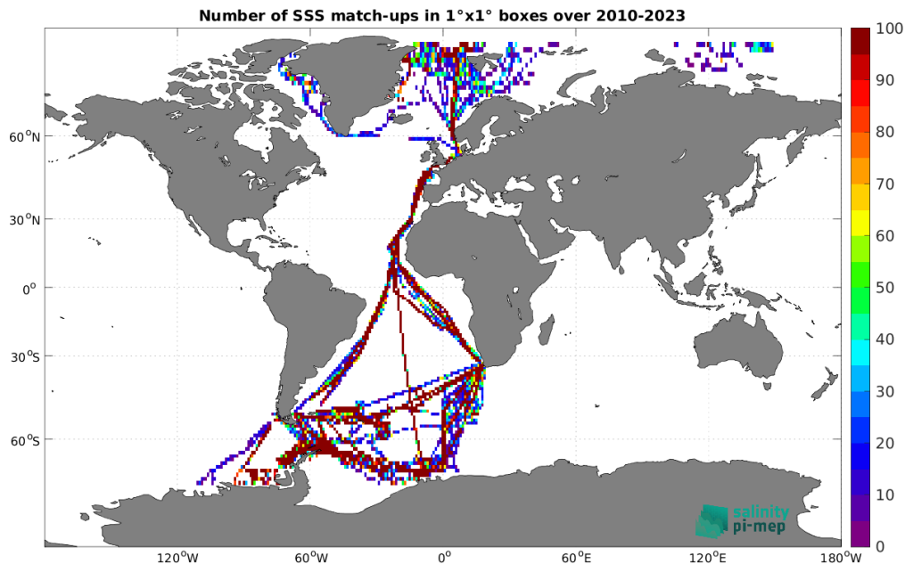
Figure 5: Number of SSS match-ups between TSG (Polarstern) SSS and the SMOS SSS L4 OI v346 - Weekly (CMEMS-CATDS-LOPS) SSS product for the Global Ocean Pi-MEP region over 1^\circ \times 1^\circ boxes and for the full satellite product period.
