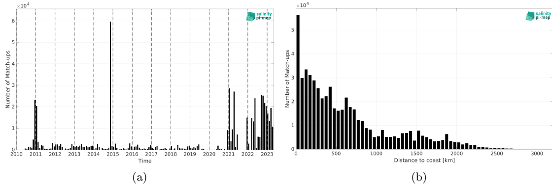
Figure 2: Number of match-ups between TSG (Polarstern) and SMOS SSS L4 OI v346 - Weekly (CMEMS-CATDS-LOPS) SSS as a function of time (a) and as function of the distance to coast (b) over the Global Ocean Pi-MEP region and for the full satellite product period.
