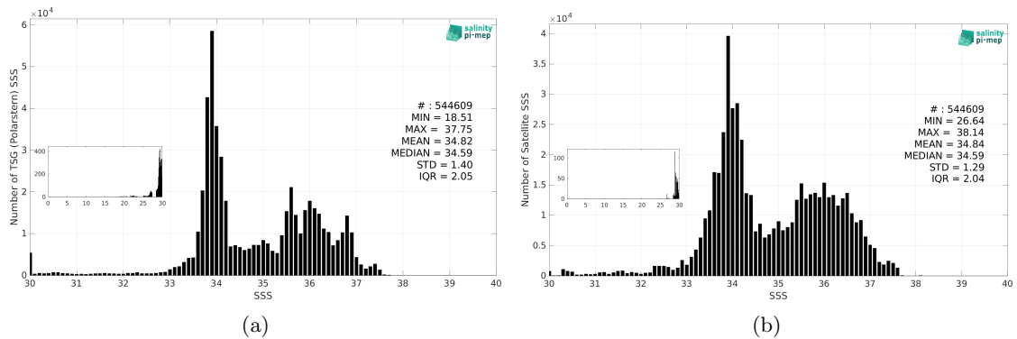
Figure 3: Histograms of SSS from TSG (Polarstern) (a) and SMOS SSS L4 OI v346 - Weekly (CMEMS-CATDS-LOPS) (b) considering all match-up pairs per bins of 0.1 over the Global Ocean Pi-MEP region and for the full satellite product period.
