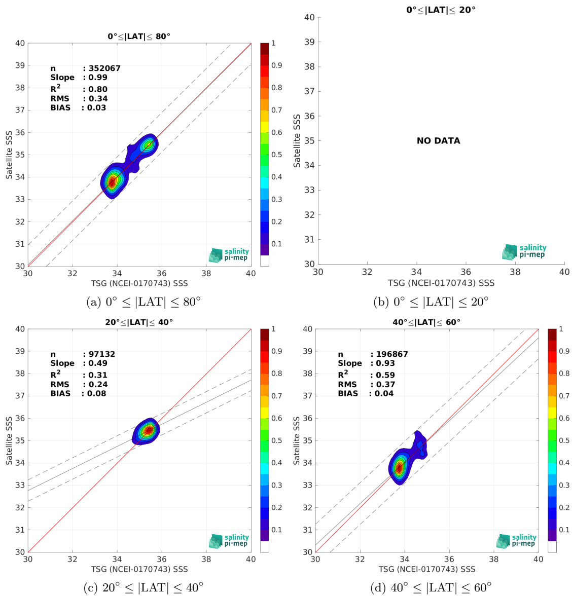
Figure 10: Contour maps of the concentration of SMOS SSS L4 OI v346 - Weekly (CMEMS-CATDS-LOPS) SSS (y-axis) versus TSG (NCEI-0170743) SSS (x-axis) at match-up pairs for different latitude bands. For each plot, the red line shows x=y . The black thin and dashed lines indicate a linear fit through the data cloud and the \pm 95\% confidence levels, respectively. The number match-up pairs n , the slope and R^2 coefficient of the linear fit, the root mean square (RMS) and the mean bias between satellite and in situ data are indicated for each latitude band in each plots.
