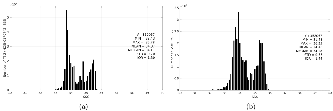
Figure 3: Histograms of SSS from TSG (NCEI-0170743) (a) and SMOS SSS L4 OI v346 - Weekly (CMEMS-CATDS-LOPS) (b) considering all match-up pairs per bins of 0.1 over the Global Ocean Pi-MEP region and for the full satellite product period.
