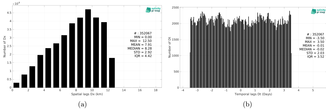
Figure 6: Histograms of the spatial (a) and temporal (b) lags between the location/time of the TSG (NCEI-0170743) measurement and the date of the corresponding SMOS SSS L4 OI v346 - Weekly (CMEMS-CATDS-LOPS) SSS pixel.
