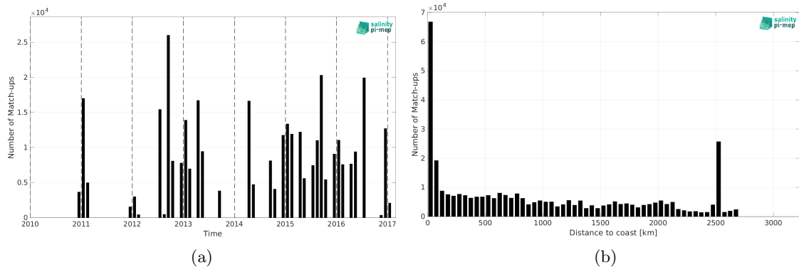
Figure 2: Number of match-ups between TSG (NCEI-0170743) and SMOS SSS L4 OI v346 - Weekly (CMEMS-CATDS-LOPS) SSS as a function of time (a) and as function of the distance to coast (b) over the Global Ocean Pi-MEP region and for the full satellite product period.
