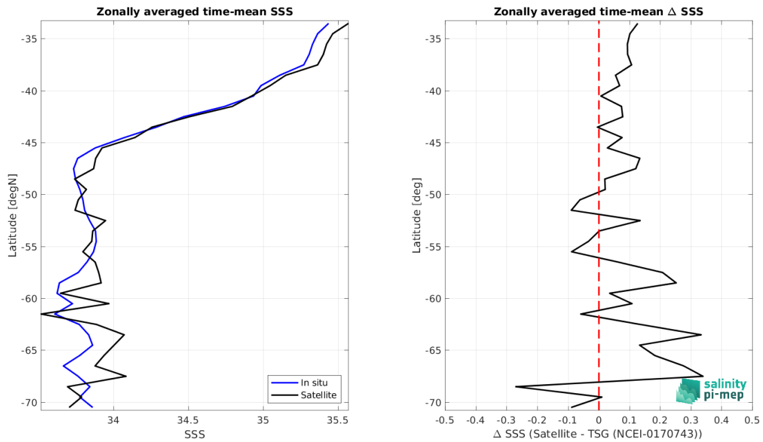
Figure 9: Left panel: Zonal mean SSS from SMOS SSS L4 OI v346 - Weekly (CMEMS-CATDS-LOPS) satellite product (black) and from TSG (NCEI-0170743) (blue). Right panel: Zonal mean of \Delta SSS (Satellite - TSG (NCEI-0170743)) for all the collected Pi-MEP match-up pairs estimated over the full satellite product period.
