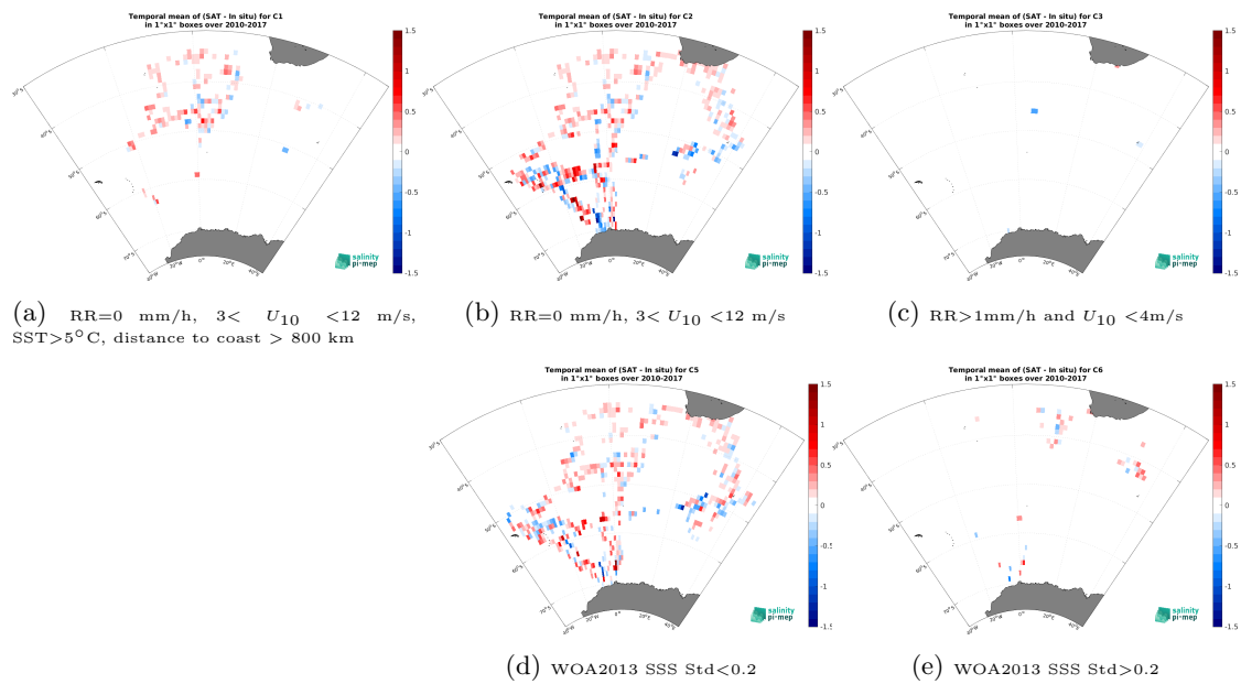
Figure 14: Temporal mean gridded over spatial boxes of size 1^\circ \times 1^\circ of \Delta SSS (SMOS SSS L4 OI v346 - Weekly (CMEMS-CATDS-LOPS) - TSG (NCEI-0170743)) for 5 different subdatasets corresponding to:RR=0 mm/h, 3 < U_{10} < 12 m/s, SST >5^\circ\text{C} , distance to coast > 800 km (a), RR=0 mm/h, 3 < U_{10} < 12 m/s (b), RR >1 mm/h and U_{10} < 4 m/s (c), WOA2013 SSS Std <0.2 (d), WOA2013 SSS Std >0.2 (e).
