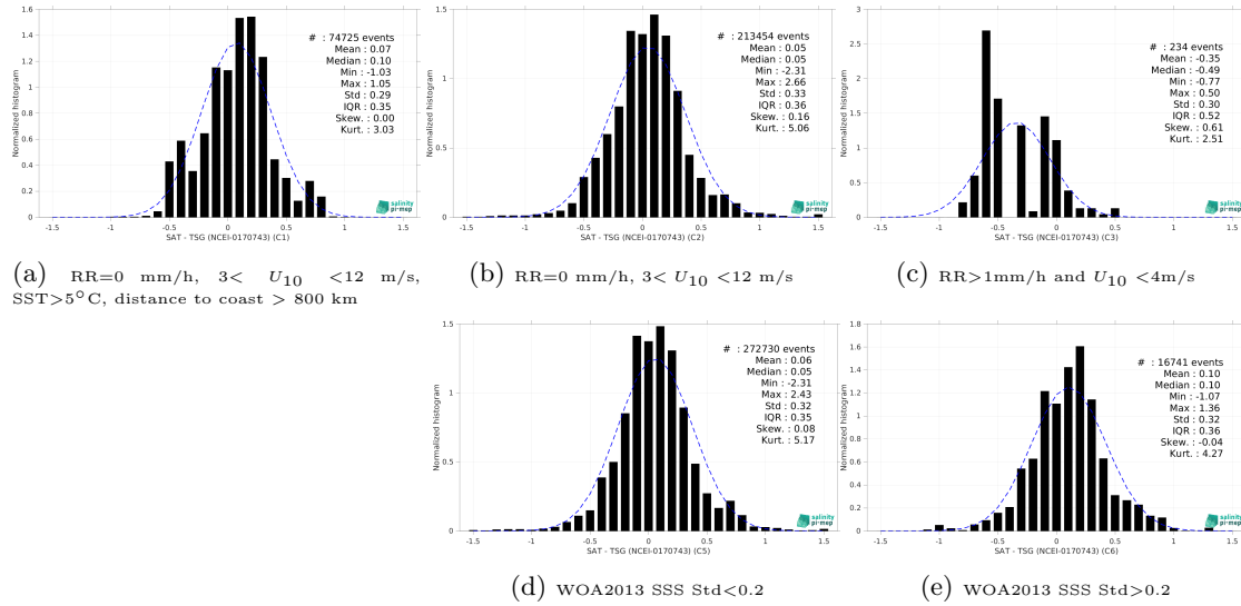
Figure 15: Normalized histogram of \Delta SSS (SMOS SSS L4 OI v346 - Weekly (CMEMS-CATDS-LOPS) - TSG (NCEI-0170743)) for 5 different subdatasets corresponding to: RR=0 mm/h, 3 < U_{10} < 12 m/s, SST>5°C, distance to coast > 800 km (a), RR=0 mm/h, 3 < U_{10} < 12 m/s (b), RR>1mm/h and U_{10} < 4 m/s (c), WOA2013 SSS Std<0.2 (d), WOA2013 SSS Std>0.2 (e).
