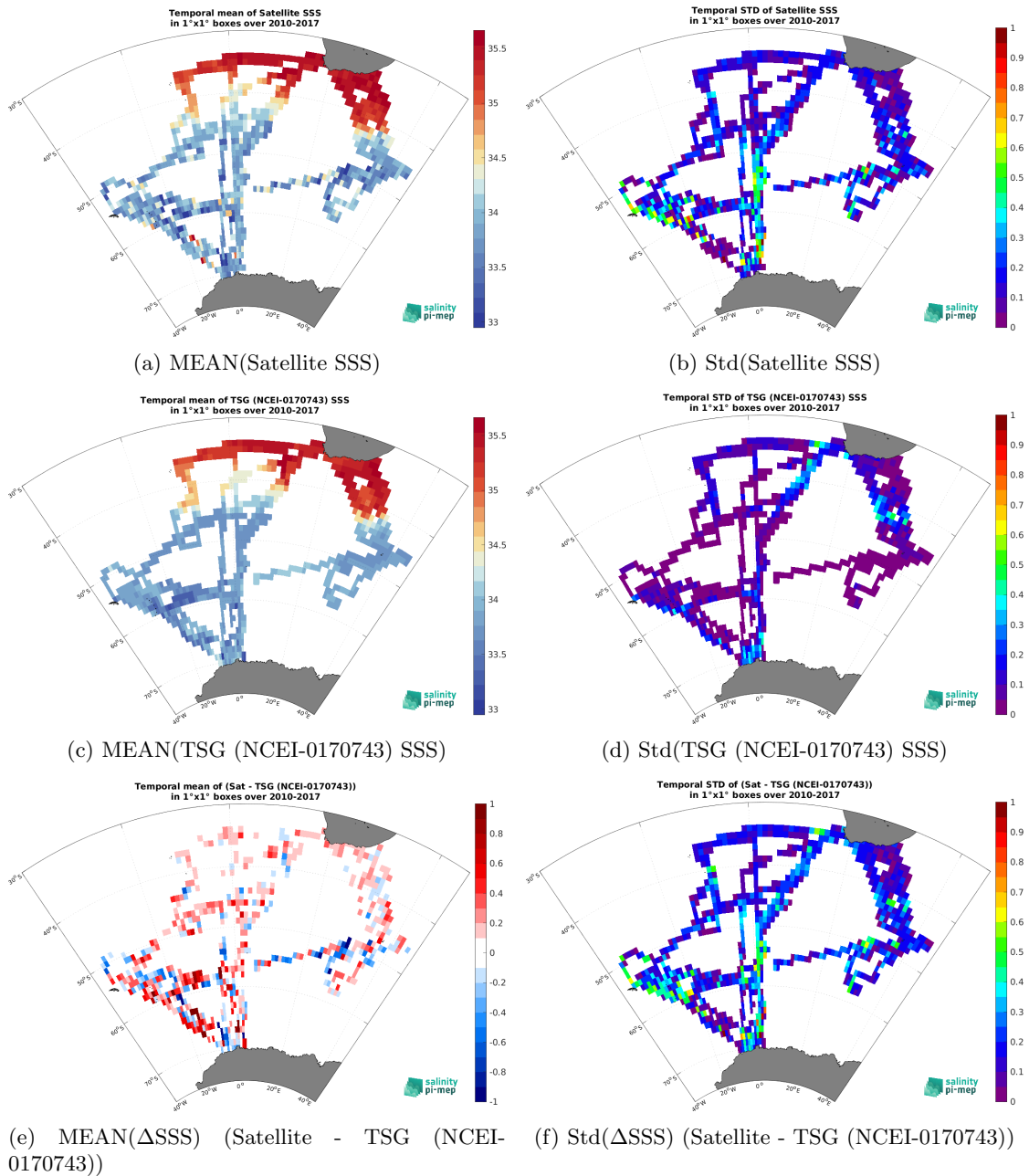
Figure 7: Temporal mean (left) and Std (right) of SSS from SMOS SSS L4 OI v346 - Weekly (CMEMS-CATDS-LOPS) (top), TSG (NCEI-0170743) (middle), and of \Delta SSS (Satellite - TSG (NCEI-0170743)). Only match-up pairs are used to generate these maps.
