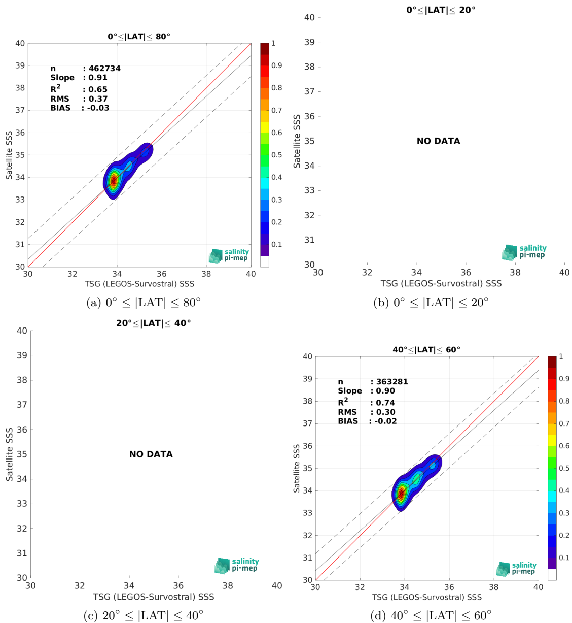
Figure 10: Contour maps of the concentration of SMOS SSS L4 OI v346 - Weekly (CMEMS-CATDS-LOPS) SSS (y-axis) versus TSG (LEGOS-Survostral) SSS (x-axis) at match-up pairs for different latitude bands. For each plot, the red line shows x=y . The black thin and dashed lines indicate a linear fit through the data cloud and the \pm 95\% confidence levels, respectively. The number match-up pairs n , the slope and R^2 coefficient of the linear fit, the root mean square (RMS) and the mean bias between satellite and in situ data are indicated for each latitude band in each plots.
