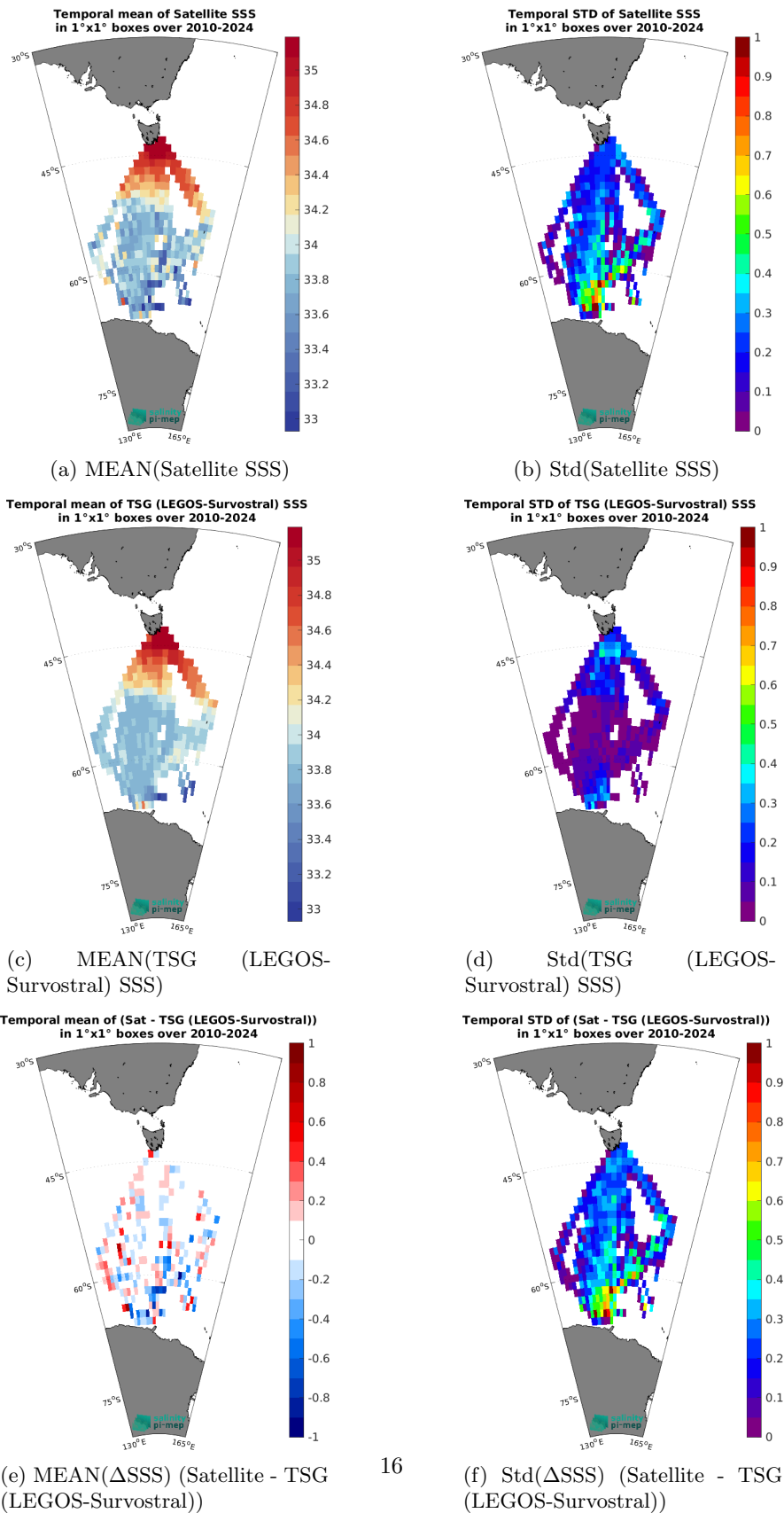
Figure 7: Temporal mean (left) and Std (right) of SSS from SMOS SSS L4 OI v346 - Weekly (CMEMS-CATDS-LOPS) (top), TSG (LEGOS-Survostral) (middle), and of \Delta SSS (Satellite - TSG (LEGOS-Survostral)). Only match-up pairs are used to generate these maps.
