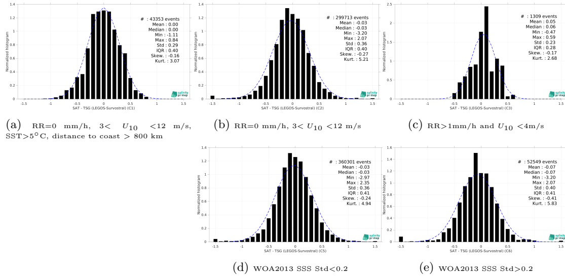
Figure 15: Normalized histogram of \Delta SSS (SMOS SSS L4 OI v346 - Weekly (CMEMS-CATDS-LOPS) - TSG (LEGOS-Survostral)) for 5 different subdatasets corresponding to: RR=0 mm/h, 3 < U_{10} < 12 m/s, SST>5°C, distance to coast > 800 km (a), RR=0 mm/h, 3 < U_{10} < 12 m/s (b), RR>1mm/h and U_{10} < 4 m/s (c), WOA2013 SSS Std<0.2 (d), WOA2013 SSS Std>0.2 (e).
