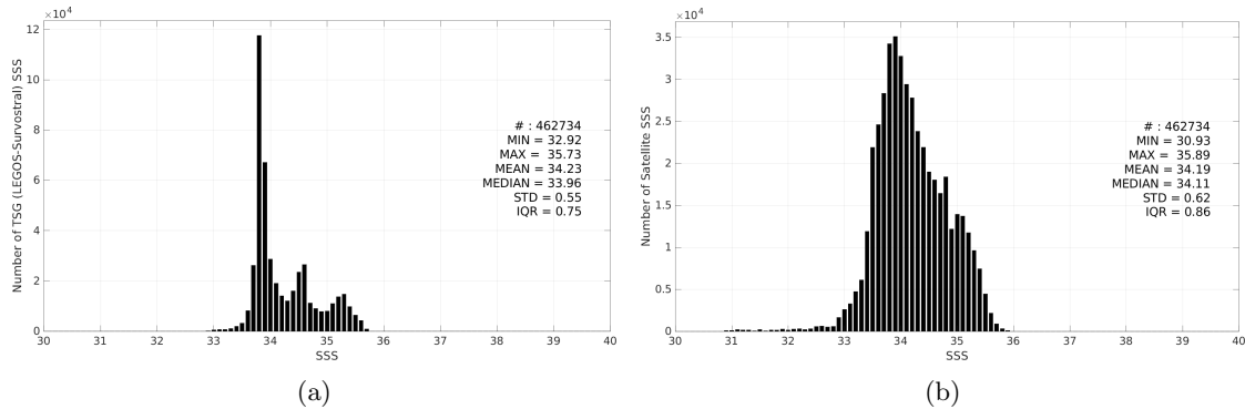
Figure 3: Histograms of SSS from TSG (LEGOS-Survostral) (a) and SMOS SSS L4 OI v346 - Weekly (CMEMS-CATDS-LOPS) (b) considering all match-up pairs per bins of 0.1 over the Global Ocean Pi-MEP region and for the full satellite product period.
