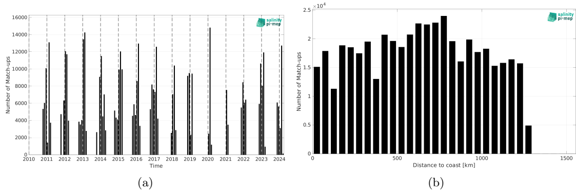
Figure 2: Number of match-ups between TSG (LEGOS-Survostral) and SMOS SSS L4 OI v346 - Weekly (CMEMS-CATDS-LOPS) SSS as a function of time (a) and as function of the distance to coast (b) over the Global Ocean Pi-MEP region and for the full satellite product period.
