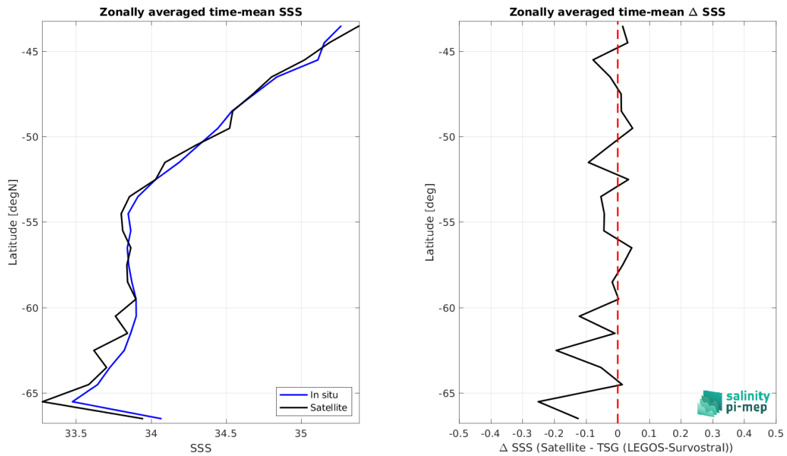
Figure 9: Left panel: Zonal mean SSS from SMOS SSS L4 OI v346 - Weekly (CMEMS-CATDS-LOPS) satellite product (black) and from TSG (LEGOS-Survostral) (blue). Right panel: Zonal mean of \Delta SSS (Satellite - TSG (LEGOS-Survostral)) for all the collected Pi-MEP match-up pairs estimated over the full satellite product period.
