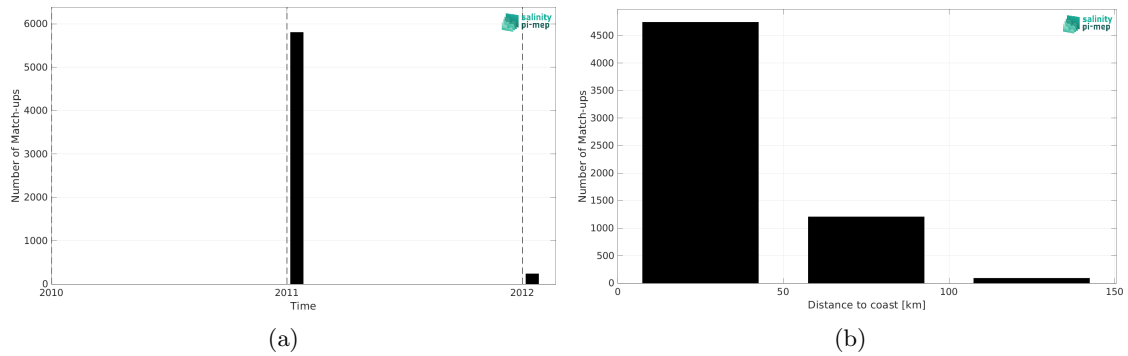
Figure 2: Number of match-ups between TSG (LEGOS-Surv-Adel) and SMOS SSS L4 OI v346 - Weekly (CMEMS-CATDS-LOPS) SSS as a function of time (a) and as function of the distance to coast (b) over the Global Ocean Pi-MEP region and for the full satellite product period.
