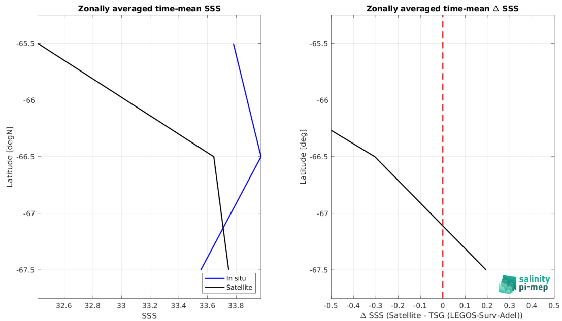
Figure 9: Left panel: Zonal mean SSS from SMOS SSS L4 OI v346 - Weekly (CMEMS-CATDS-LOPS) satellite product (black) and from TSG (LEGOS-Surv-Adel) (blue). Right panel: Zonal mean of \Delta SSS (Satellite - TSG (LEGOS-Surv-Adel)) for all the collected Pi-MEP match-up pairs estimated over the full satellite product period.
