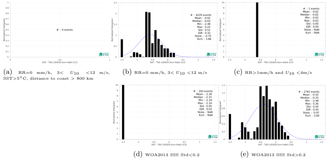
Figure 15: Normalized histogram of \Delta\text{SSS} (SMOS SSS L4 OI v346 - Weekly (CMEMS-CATDS-LOPS) - TSG (LEGOS-Surv-Adel)) for 5 different subdatasets corresponding to: RR=0 mm/h, 3 < U_{10} < 12 m/s, SST > 5^{\circ}\text{C} , distance to coast > 800 km (a), RR=0 mm/h, 3 < U_{10} < 12 m/s (b), RR > 1\text{mm/h} and U_{10} < 4\text{m/s} (c), WOA2013 SSS Std < 0.2 (d), WOA2013 SSS Std > 0.2 (e).
