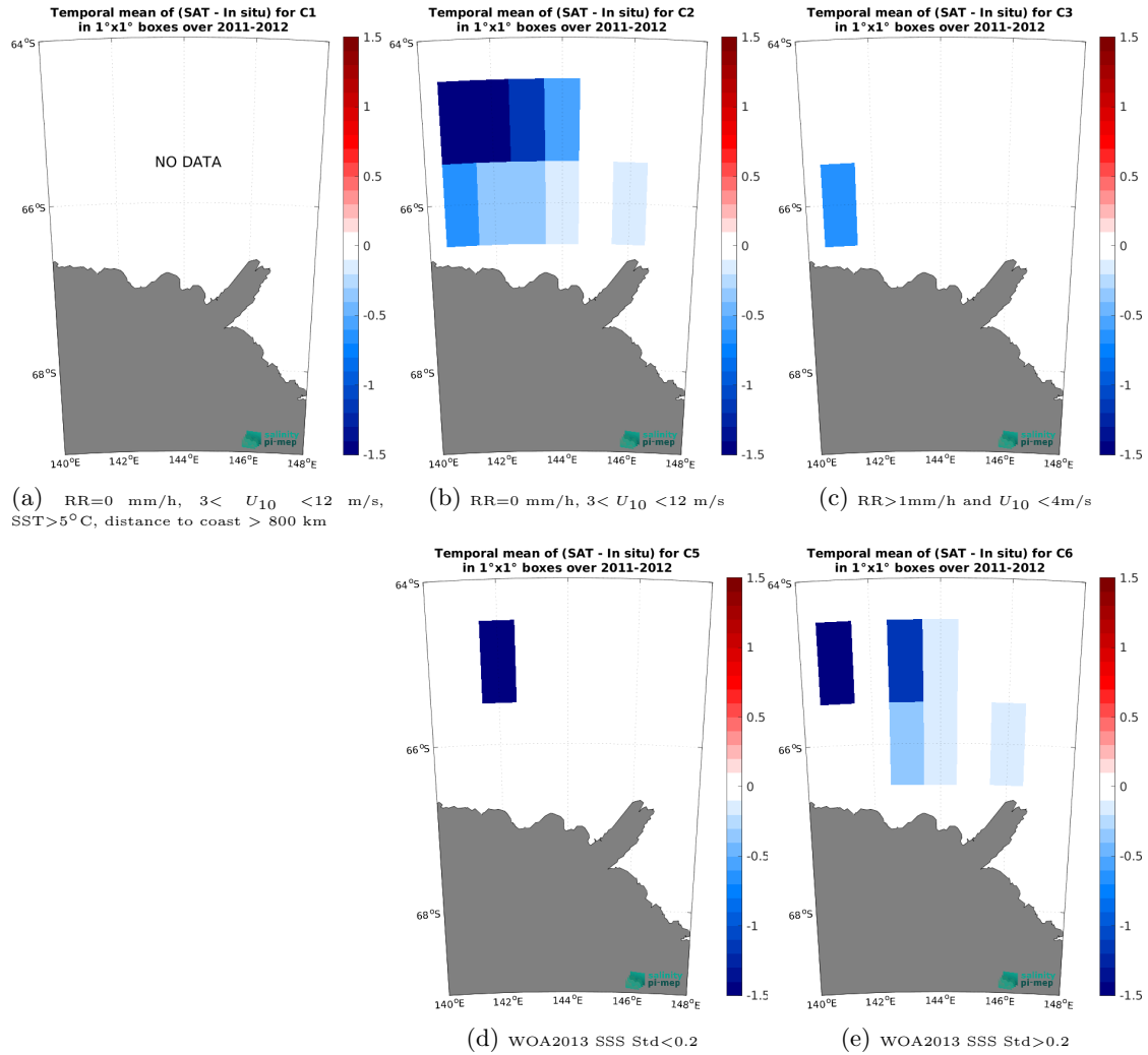
Figure 14: Temporal mean gridded over spatial boxes of size 1^\circ \times 1^\circ of \Delta SSS (SMOS SSS L4 OI v346 - Weekly (CMEMS-CATDS-LOPS) - TSG (LEGOS-Surv-Adel)) for 5 different subdatasets corresponding to: RR=0 mm/h, 3 < U_{10} < 12 m/s, SST>5°C, distance to coast > 800 km (a), RR=0 mm/h, 3 < U_{10} < 12 m/s (b), RR>1mm/h and U_{10} < 4 m/s (c), WOA2013 SSS Std<0.2 (d), WOA2013 SSS Std>0.2 (e).
