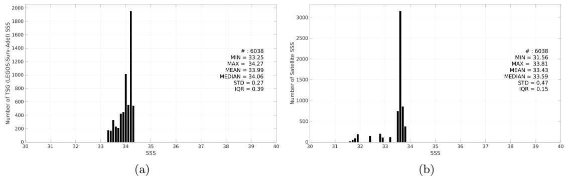
Figure 3: Histograms of SSS from TSG (LEGOS-Surv-Adel) (a) and SMOS SSS L4 OI v346 - Weekly (CMEMS-CATDS-LOPS) (b) considering all match-up pairs per bins of 0.1 over the Global Ocean Pi-MEP region and for the full satellite product period.
