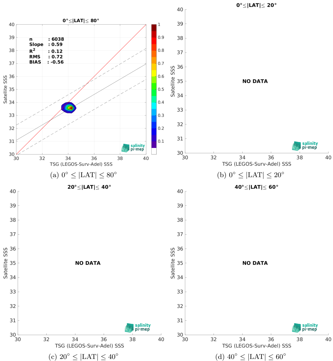
Figure 10: Contour maps of the concentration of SMOS SSS L4 OI v346 - Weekly (CMEMS-CATDS-LOPS) SSS (y-axis) versus TSG (LEGOS-Surv-Adel) SSS (x-axis) at match-up pairs for different latitude bands. For each plot, the red line shows x=y . The black thin and dashed lines indicate a linear fit through the data cloud and the \pm 95\% confidence levels, respectively. The number match-up pairs n , the slope and R^2 coefficient of the linear fit, the root mean square (RMS) and the mean bias between satellite and in situ data are indicated for each latitude band in each plots.
