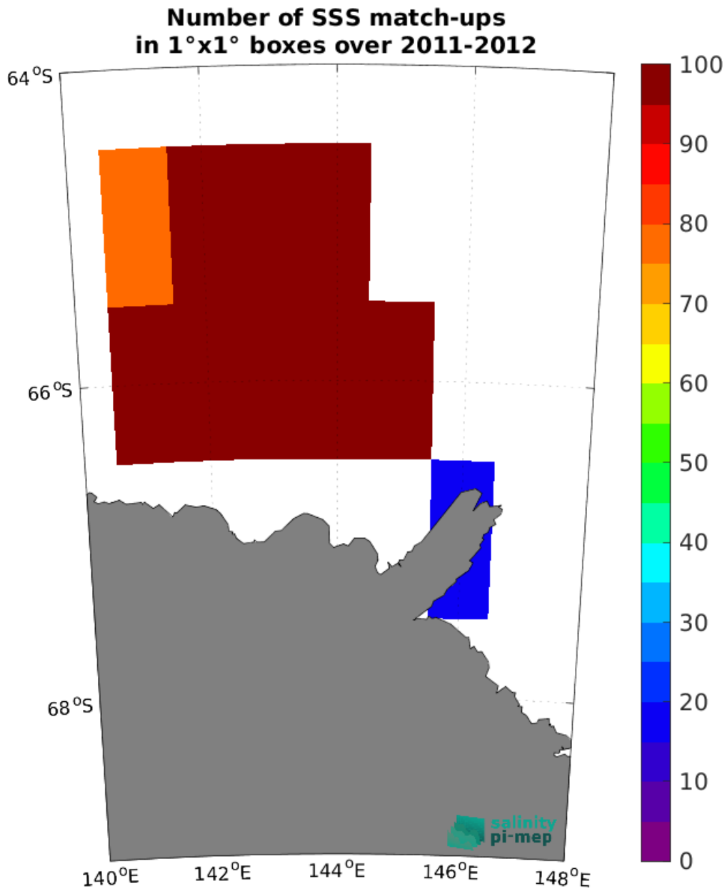
Figure 5: Number of SSS match-ups between TSG (LEGOS-Surv-Adel) SSS and the SMOS SSS L4 OI v346 - Weekly (CMEMS-CATDS-LOPS) SSS product for the Global Ocean Pi-MEP region over 1^\circ \times 1^\circ boxes and for the full satellite product period.
