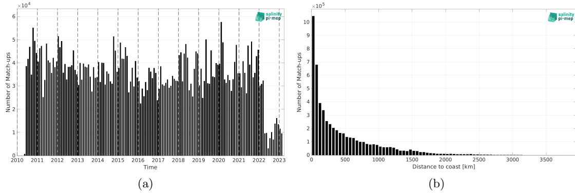
Figure 2: Number of match-ups between TSG (LEGOS-DM) and SMOS SSS L4 OI v346 - Weekly (CMEMS-CATDS-LOPS) SSS as a function of time (a) and as function of the distance to coast (b) over the Global Ocean Pi-MEP region and for the full satellite product period.
