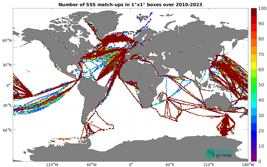
Figure 5: Number of SSS match-ups between TSG (LEGOS-DM) SSS and the SMOS SSS L4 OI v346 - Weekly (CMEMS-CATDS-LOPS) SSS product for the Global Ocean Pi-MEP region over 1^\circ \times 1^\circ boxes and for the full satellite product period.
