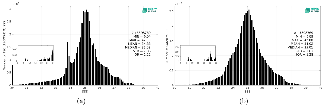
Figure 3: Histograms of SSS from TSG (LEGOS-DM) (a) and SMOS SSS L4 OI v346 - Weekly (CMEMS-CATDS-LOPS) (b) considering all match-up pairs per bins of 0.1 over the Global Ocean Pi-MEP region and for the full satellite product period.
