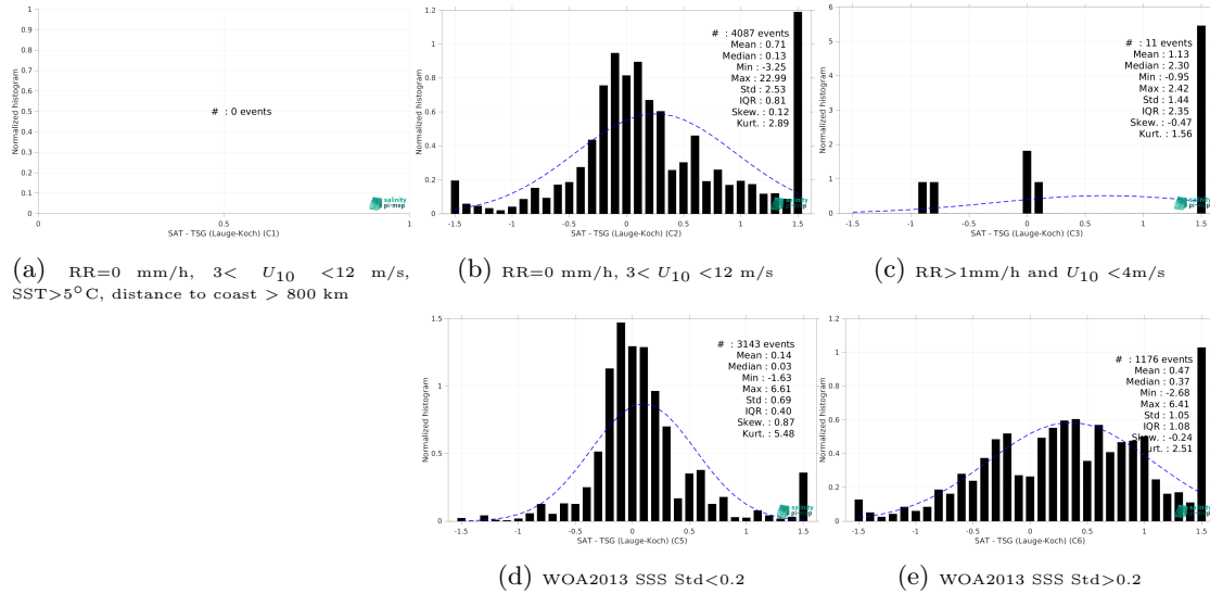
Figure 15: Normalized histogram of \Delta SSS (SMOS SSS L4 OI v346 - Weekly (CMEMS-CATDS-LOPS) - TSG (Lauge-Koch)) for 5 different subdatasets corresponding to: RR=0 mm/h, 3 < U_{10} < 12 m/s, SST>5°C, distance to coast > 800 km (a), RR=0 mm/h, 3 < U_{10} < 12 m/s (b), RR>1mm/h and U_{10} < 4 m/s (c), WOA2013 SSS Std<0.2 (d), WOA2013 SSS Std>0.2 (e).
