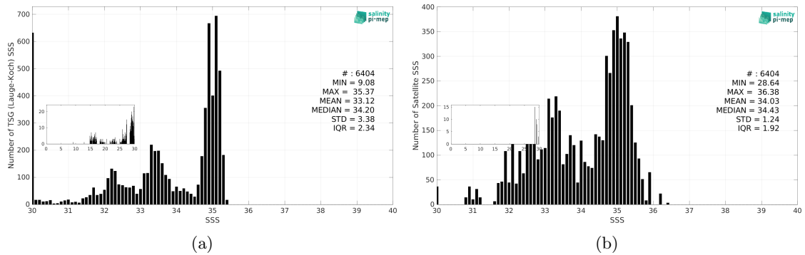
Figure 3: Histograms of SSS from TSG (Lauge-Koch) (a) and SMOS SSS L4 OI v346 - Weekly (CMEMS-CATDS-LOPS) (b) considering all match-up pairs per bins of 0.1 over the Global Ocean Pi-MEP region and for the full satellite product period.
