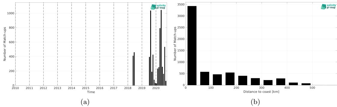
Figure 2: Number of match-ups between TSG (Lauge-Koch) and SMOS SSS L4 OI v346 - Weekly (CMEMS-CATDS-LOPS) SSS as a function of time (a) and as function of the distance to coast (b) over the Global Ocean Pi-MEP region and for the full satellite product period.
