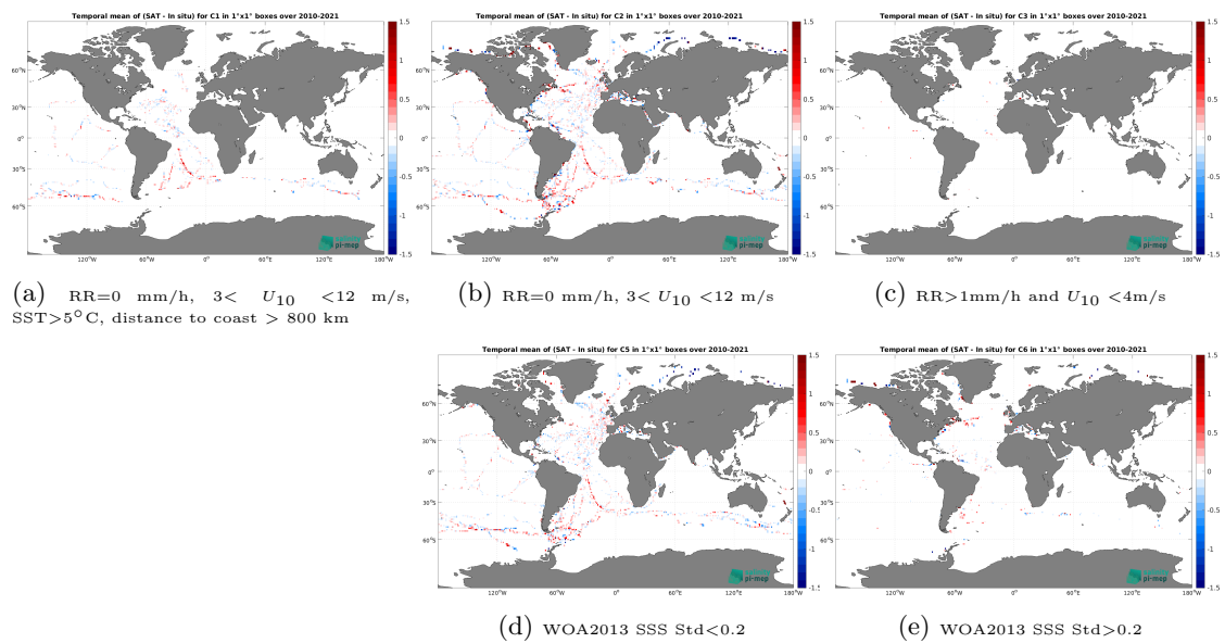
Figure 14: Temporal mean gridded over spatial boxes of size 1^\circ \times 1^\circ of \Delta SSS (SMOS SSS L4 OI v346 - Weekly (CMEMS-CATDS-LOPS) - TSG (GOSUD-Sailing-ship)) for 5 different sub-datasets corresponding to: RR=0 mm/h, 3 < U_{10} < 12 m/s, SST > 5^\circ\text{C} , distance to coast > 800 km (a), RR=0 mm/h, 3 < U_{10} < 12 m/s (b), RR > 1 mm/h and U_{10} < 4 m/s (c), WOA2013 SSS Std < 0.2 (d), WOA2013 SSS Std > 0.2 (e).
