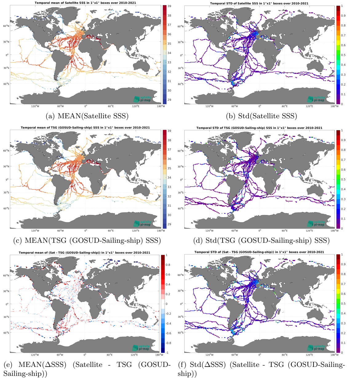
Figure 7: Temporal mean (left) and Std (right) of SSS from SMOS SSS L4 OI v346 - Weekly (CMEMS-CATDS-LOPS) (top), TSG (GOSUD-Sailing-ship) (middle), and of \Delta SSS (Satellite - TSG (GOSUD-Sailing-ship)). Only match-up pairs are used to generate these maps.
