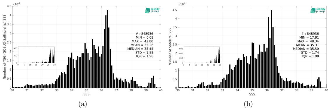
Figure 3: Histograms of SSS from TSG (GOSUD-Sailing-ship) (a) and SMOS SSS L4 OI v346 - Weekly (CMEMS-CATDS-LOPS) (b) considering all match-up pairs per bins of 0.1 over the Global Ocean Pi-MEP region and for the full satellite product period.
