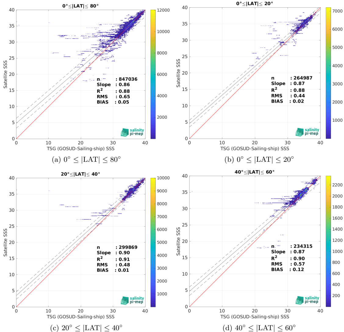
Figure 10: Contour maps of the concentration of SMOS SSS L4 OI v346 - Weekly (CMEMS-CATDS-LOPS) SSS (y-axis) versus TSG (GOSUD-Sailing-ship) SSS (x-axis) at match-up pairs for different latitude bands. For each plot, the red line shows x=y . The black thin and dashed lines indicate a linear fit through the data cloud and the \pm 95\% confidence levels, respectively. The number match-up pairs n , the slope and R^2 coefficient of the linear fit, the root mean square (RMS) and the mean bias between satellite and in situ data are indicated for each latitude band in each plots.
