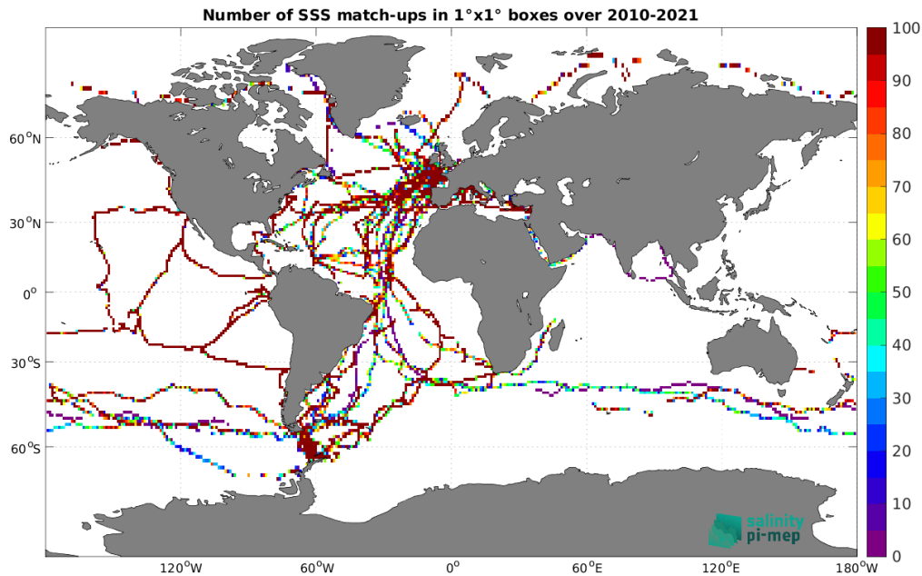
Figure 5: Number of SSS match-ups between TSG (GOSUD-Sailing-ship) SSS and the SMOS SSS L4 OI v346 - Weekly (CMEMS-CATDS-LOPS) SSS product for the Global Ocean Pi-MEP region over 1^\circ \times 1^\circ boxes and for the full satellite product period.
