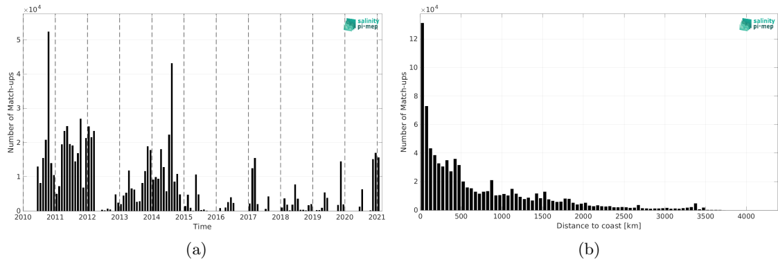
Figure 2: Number of match-ups between TSG (GOSUD-Sailing-ship) and SMOS SSS L4 OI v346 - Weekly (CMEMS-CATDS-LOPS) SSS as a function of time (a) and as function of the distance to coast (b) over the Global Ocean Pi-MEP region and for the full satellite product period.
