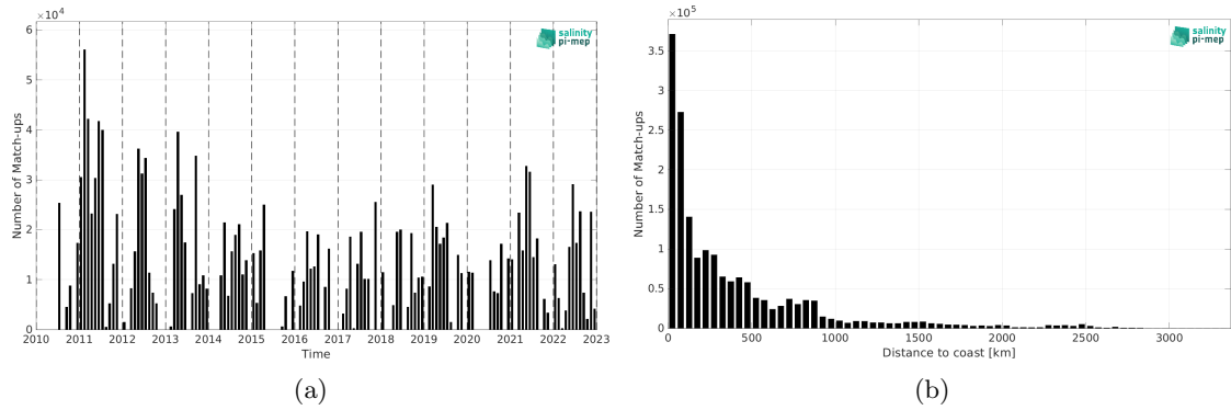
Figure 2: Number of match-ups between TSG (CSIC-UTM) and SMOS SSS L4 OI v346 - Weekly (CMEMS-CATDS-LOPS) SSS as a function of time (a) and as function of the distance to coast (b) over the Global Ocean Pi-MEP region and for the full satellite product period.
