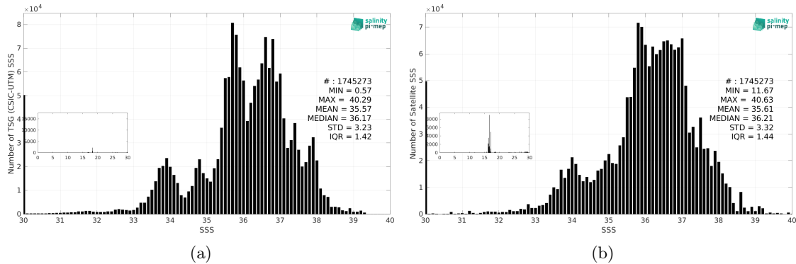
Figure 3: Histograms of SSS from TSG (CSIC-UTM) (a) and SMOS SSS L4 OI v346 - Weekly (CMEMS-CATDS-LOPS) (b) considering all match-up pairs per bins of 0.1 over the Global Ocean Pi-MEP region and for the full satellite product period.
