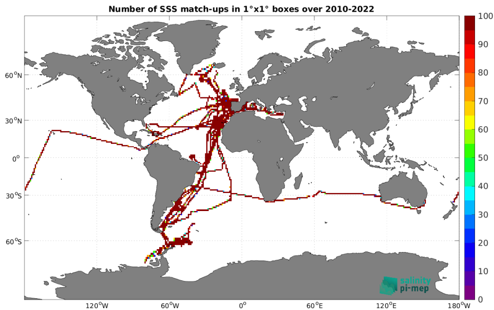
Figure 5: Number of SSS match-ups between TSG (CSIC-UTM) SSS and the SMOS SSS L4 OI v346 - Weekly (CMEMS-CATDS-LOPS) SSS product for the Global Ocean Pi-MEP region over 1^\circ \times 1^\circ boxes and for the full satellite product period.
