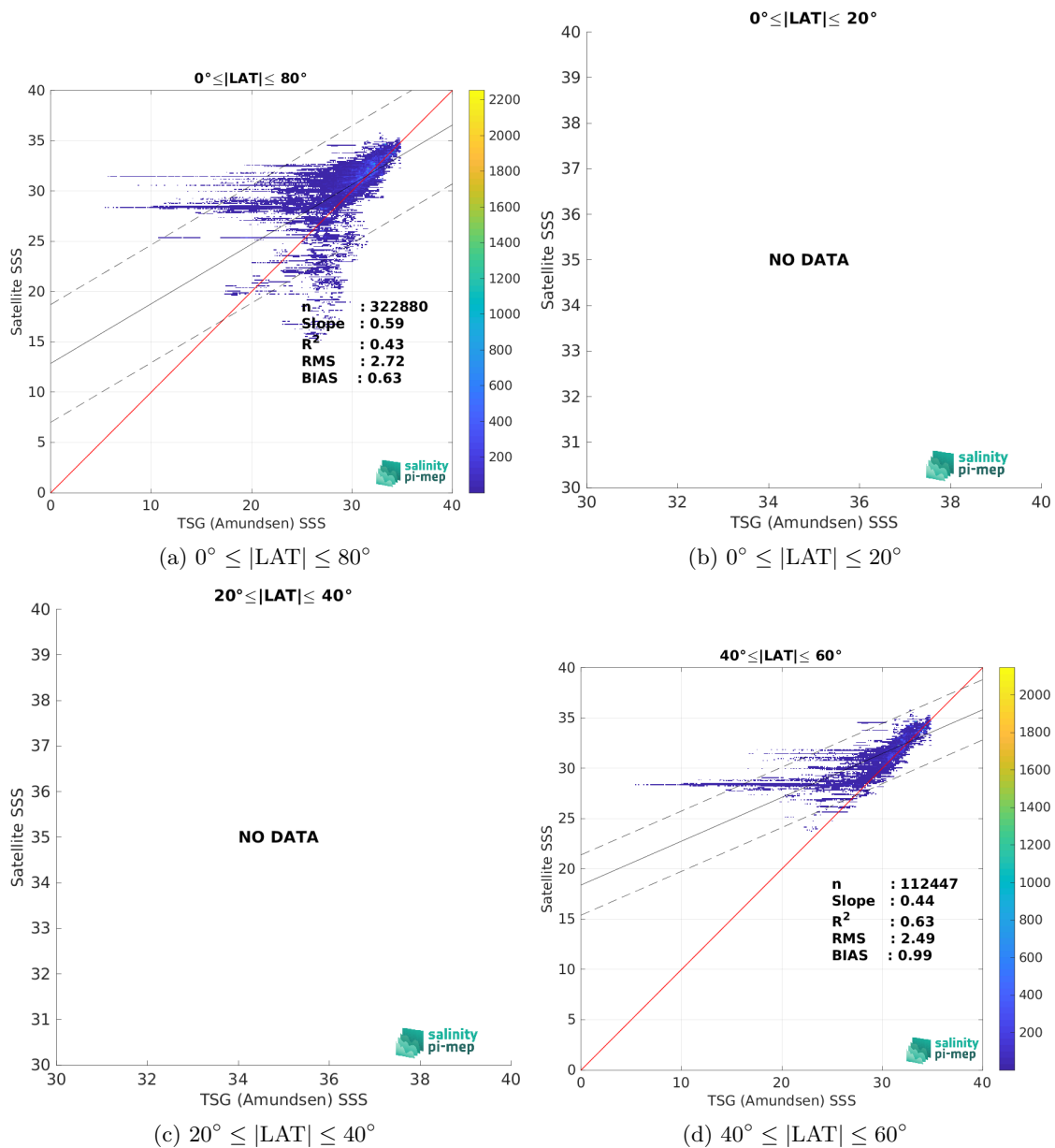
Figure 10: Contour maps of the concentration of SMOS SSS L4 OI v346 - Weekly (CMEMS-CATDS-LOPS) SSS (y-axis) versus TSG (Amundsen) SSS (x-axis) at match-up pairs for different latitude bands. For each plot, the red line shows x=y . The black thin and dashed lines indicate a linear fit through the data cloud and the \pm 95\% confidence levels, respectively. The number match-up pairs n , the slope and R^2 coefficient of the linear fit, the root mean square (RMS) and the mean bias between satellite and in situ data are indicated for each latitude band in each plots.
