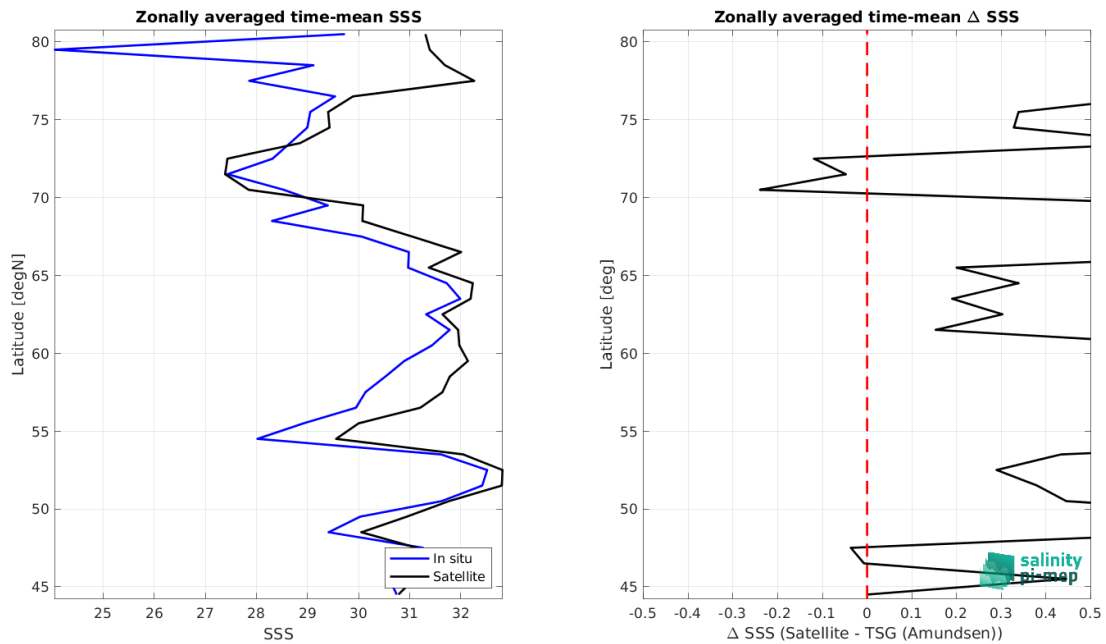
Figure 9: Left panel: Zonal mean SSS from SMOS SSS L4 OI v346 - Weekly (CMEMS-CATDS-LOPS) satellite product (black) and from TSG (Amundsen) (blue). Right panel: Zonal mean of \Delta SSS (Satellite - TSG (Amundsen)) for all the collected Pi-MEP match-up pairs estimated over the full satellite product period.
