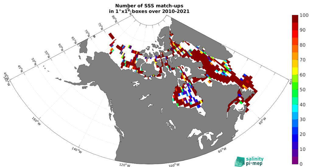
Figure 5: Number of SSS match-ups between TSG (Amundsen) SSS and the SMOS SSS L4 OI v346 - Weekly (CMEMS-CATDS-LOPS) SSS product for the Global Ocean Pi-MEP region over 1^\circ \times 1^\circ boxes and for the full satellite product period.
