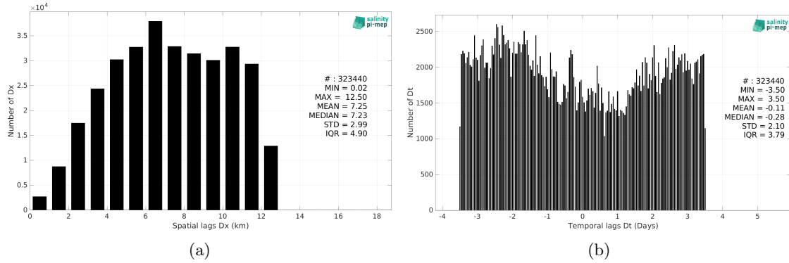
Figure 6: Histograms of the spatial (a) and temporal (b) lags between the location/time of the TSG (Amundsen) measurement and the date of the corresponding SMOS SSS L4 OI v346 - Weekly (CMEMS-CATDS-LOPS) SSS pixel.
