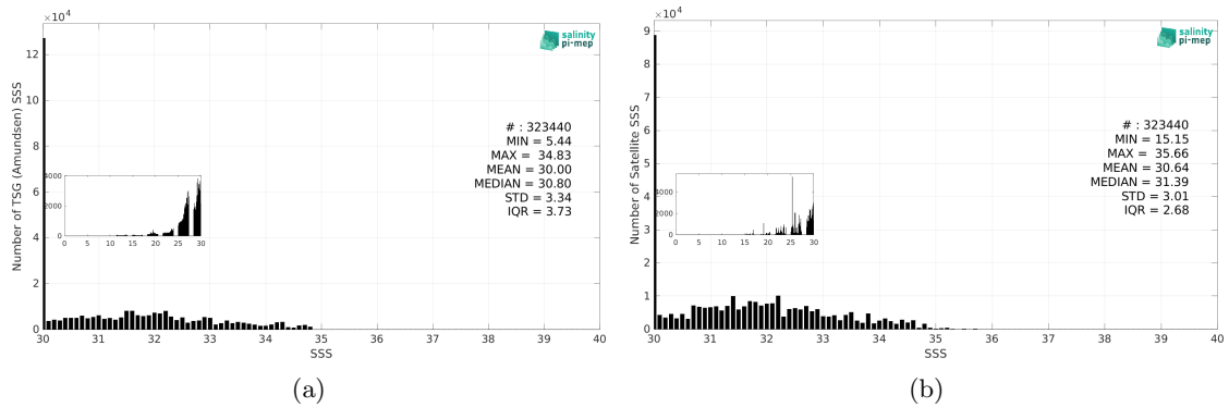
Figure 3: Histograms of SSS from TSG (Amundsen) (a) and SMOS SSS L4 OI v346 - Weekly (CMEMS-CATDS-LOPS) (b) considering all match-up pairs per bins of 0.1 over the Global Ocean Pi-MEP region and for the full satellite product period.
