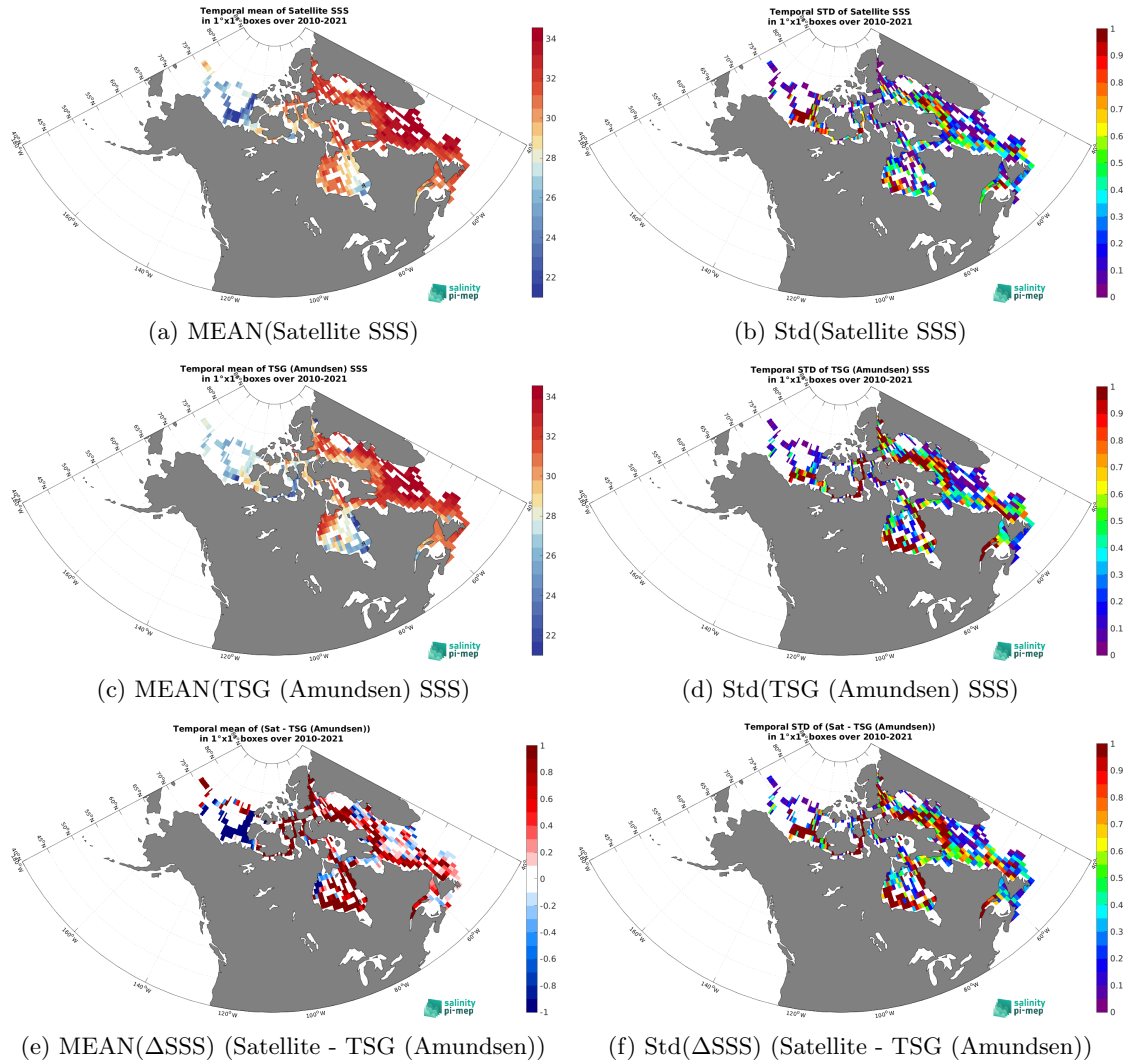
Figure 7: Temporal mean (left) and Std (right) of SSS from SMOS SSS L4 OI v346 - Weekly (CMEMS-CATDS-LOPS) (top), TSG (Amundsen) (middle), and of \Delta SSS (Satellite - TSG (Amundsen)). Only match-up pairs are used to generate these maps.
