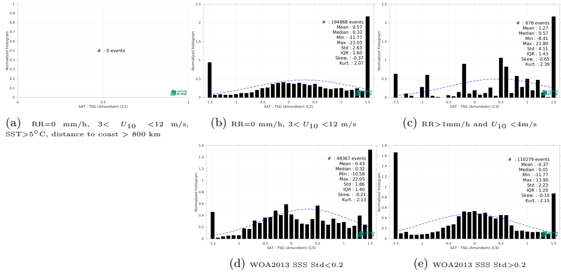
Figure 15: Normalized histogram of \Delta SSS (SMOS SSS L4 OI v346 - Weekly (CMEMS-CATDS-LOPS) - TSG (Amundsen)) for 5 different subdatasets corresponding to: RR=0 mm/h, 3 < U_{10} < 12 m/s, SST > 5°C, distance to coast > 800 km (a), RR=0 mm/h, 3 < U_{10} < 12 m/s (b), RR > 1mm/h and U_{10} < 4 m/s (c), WOA2013 SSS Std < 0.2 (d), WOA2013 SSS Std > 0.2 (e).
