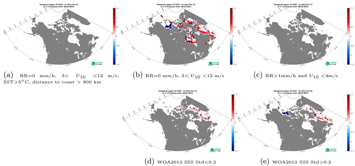
Figure 14: Temporal mean gridded over spatial boxes of size 1^\circ \times 1^\circ of \Delta SSS (SMOS SSS L4 OI v346 - Weekly (CMEMS-CATDS-LOPS) - TSG (Amundsen)) for 5 different subdatasets corresponding to: RR=0 mm/h, 3 < U_{10} < 12 m/s, SST>5°C, distance to coast > 800 km (a), RR=0 mm/h, 3 < U_{10} < 12 m/s (b), RR>1mm/h and U_{10} < 4 m/s (c), WOA2013 SSS Std<0.2 (d), WOA2013 SSS Std>0.2 (e).
