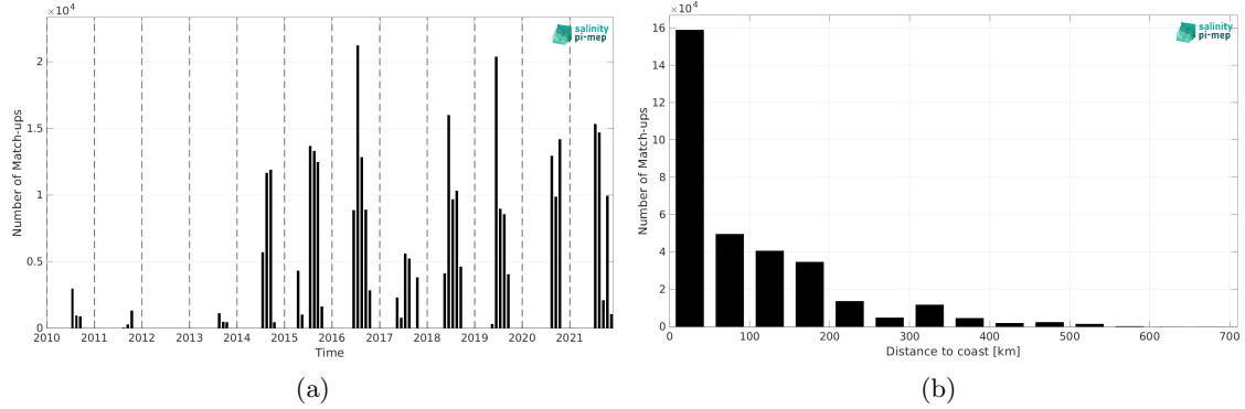
Figure 2: Number of match-ups between TSG (Amundsen) and SMOS SSS L4 OI v346 - Weekly (CMEMS-CATDS-LOPS) SSS as a function of time (a) and as function of the distance to coast (b) over the Global Ocean Pi-MEP region and for the full satellite product period.
