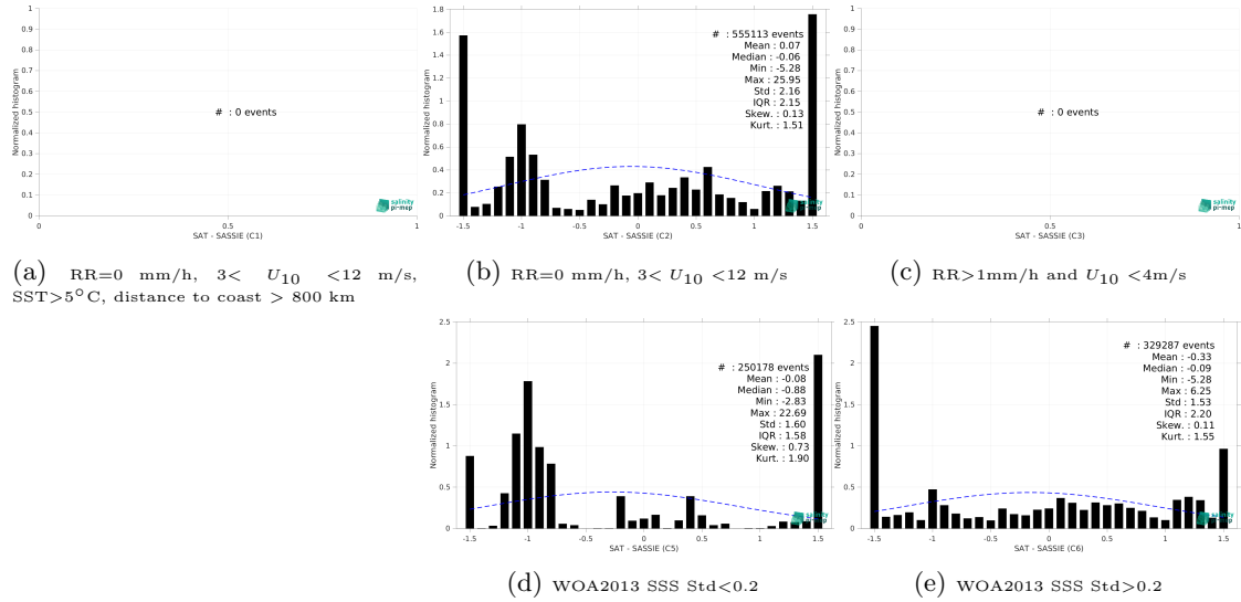
Figure 15: Normalized histogram of \Delta SSS (SMOS SSS L4 OI v346 - Weekly (CMEMS-CATDS-LOPS) - SASSIE) for 5 different subdatasets corresponding to: RR=0 mm/h, 3 < U_{10} < 12 m/s, SST>5°C, distance to coast > 800 km (a), RR=0 mm/h, 3 < U_{10} < 12 m/s (b), RR>1mm/h and U_{10} < 4 m/s (c), WOA2013 SSS Std<0.2 (d), WOA2013 SSS Std>0.2 (e).
