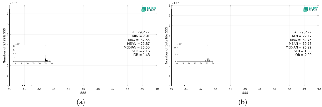
Figure 3: Histograms of SSS from SASSIE (a) and SMOS SSS L4 OI v346 - Weekly (CMEMS-CATDS-LOPS) (b) considering all match-up pairs per bins of 0.1 over the Global Ocean Pi-MEP region and for the full satellite product period.
