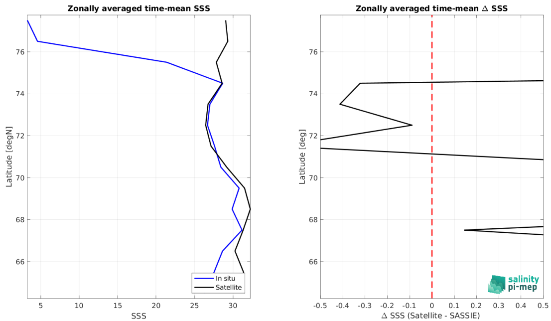
Figure 9: Left panel: Zonal mean SSS from SMOS SSS L4 OI v346 - Weekly (CMEMS-CATDS-LOPS) satellite product (black) and from SASSIE (blue). Right panel: Zonal mean of \Delta SSS (Satellite - SASSIE) for all the collected Pi-MEP match-up pairs estimated over the full satellite product period.
