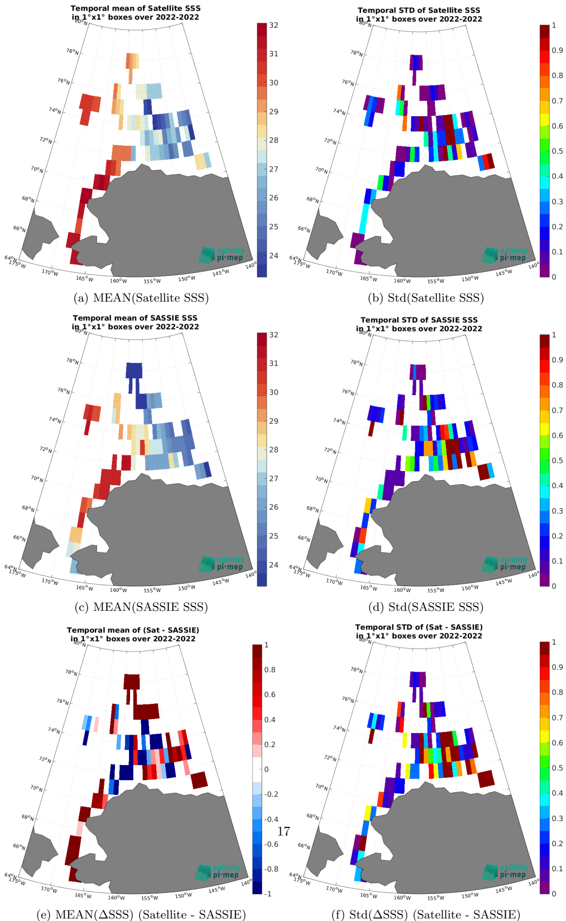
Figure 7: Temporal mean (left) and Std (right) of SSS from SMOS SSS L4 OI v346 - Weekly (CMEMS-CATDS-LOPS) (top), SASSIE (middle), and of \Delta SSS (Satellite - SASSIE). Only match-up pairs are used to generate these maps.
