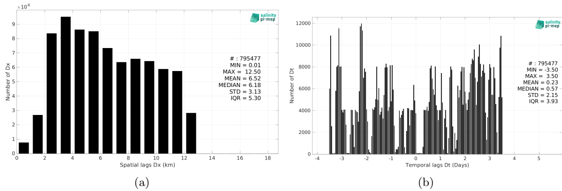
Figure 6: Histograms of the spatial (a) and temporal (b) lags between the location/time of the SASSIE measurement and the date of the corresponding SMOS SSS L4 OI v346 - Weekly (CMEMS-CATDS-LOPS) SSS pixel.
