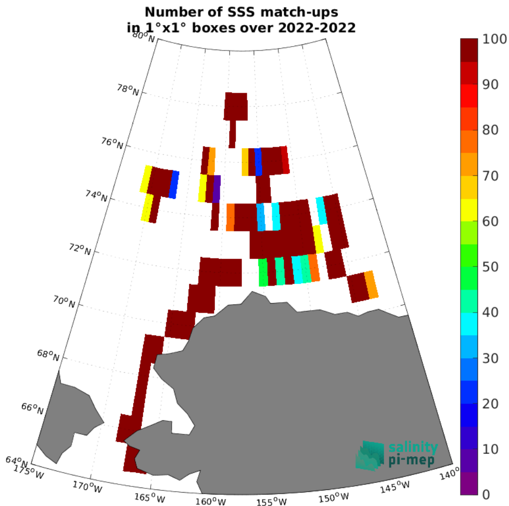
Figure 5: Number of SSS match-ups between SASSIE SSS and the SMOS SSS L4 OI v346 - Weekly (CMEMS-CATDS-LOPS) SSS product for the Global Ocean Pi-MEP region over 1^\circ \times 1^\circ boxes and for the full satellite product period.
