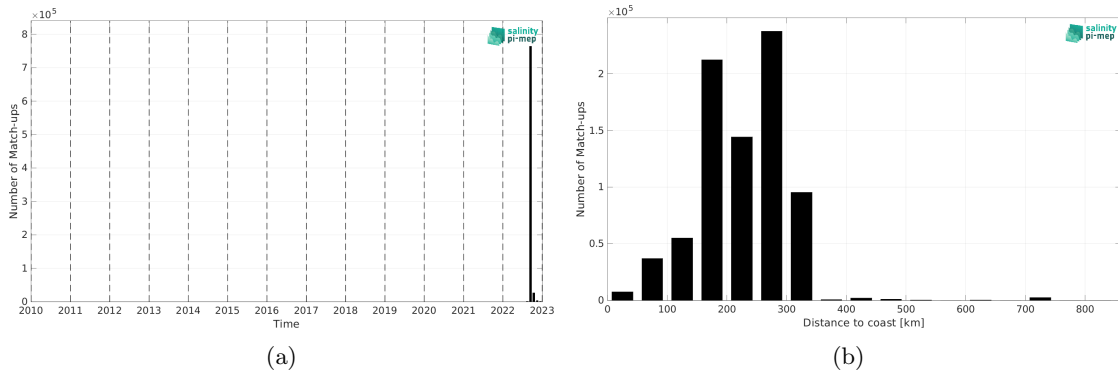
Figure 2: Number of match-ups between SASSIE and SMOS SSS L4 OI v346 - Weekly (CMEMS-CATDS-LOPS) SSS as a function of time (a) and as function of the distance to coast (b) over the Global Ocean Pi-MEP region and for the full satellite product period.
