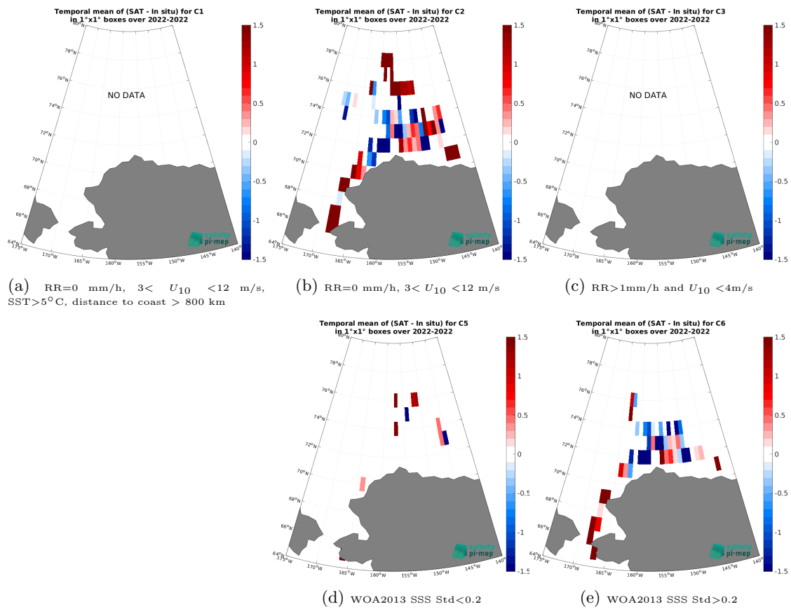
Figure 14: Temporal mean gridded over spatial boxes of size 1^\circ \times 1^\circ of \Delta SSS (SMOS SSS L4 OI v346 - Weekly (CMEMS-CATDS-LOPS) - SASSIE) for 5 different subdatasets corresponding to:RR=0 mm/h, 3 < U_{10} < 12 m/s, SST>5°C, distance to coast > 800 km (a), RR=0 mm/h, 3 < U_{10} < 12 m/s (b), RR>1mm/h and U_{10} < 4 m/s (c), WOA2013 SSS Std<0.2 (d), WOA2013 SSS Std>0.2 (e).
