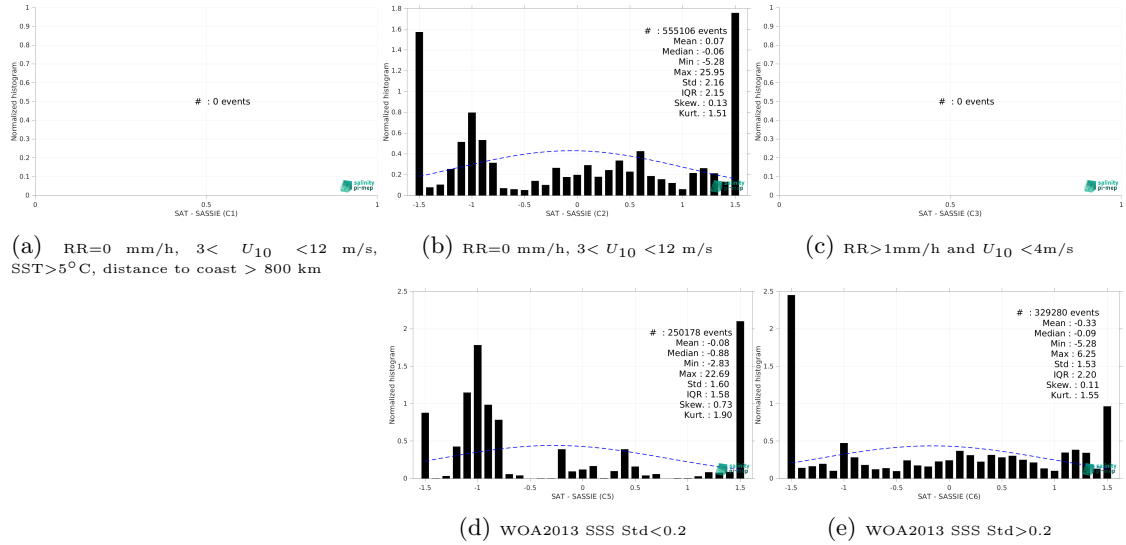
Figure 15: Normalized histogram of \Delta SSS (SMOS SSS L4 OI v346 - Weekly (CMEMS-CATDS-LOPS) - SASSIE) for 5 different subdatasets corresponding to: RR=0 mm/h, 3 < U_{10} < 12 m/s, SST > 5°C, distance to coast > 800 km (a), RR=0 mm/h, 3 < U_{10} < 12 m/s (b), RR > 1mm/h and U_{10} < 4 m/s (c), WOA2013 SSS Std < 0.2 (d), WOA2013 SSS Std > 0.2 (e).
