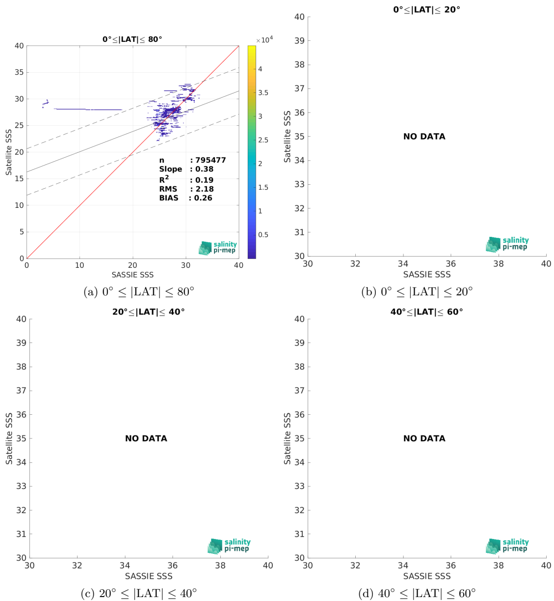
Figure 10: Contour maps of the concentration of SMOS SSS L4 OI v346 - Weekly (CMEMS-CATDS-LOPS) SSS (y-axis) versus SASSIE SSS (x-axis) at match-up pairs for different latitude bands. For each plot, the red line shows x=y . The black thin and dashed lines indicate a linear fit through the data cloud and the \pm 95\% confidence levels, respectively. The number match-up pairs n , the slope and R^2 coefficient of the linear fit, the root mean square (RMS) and the mean bias between satellite and in situ data are indicated for each latitude band in each plots.
