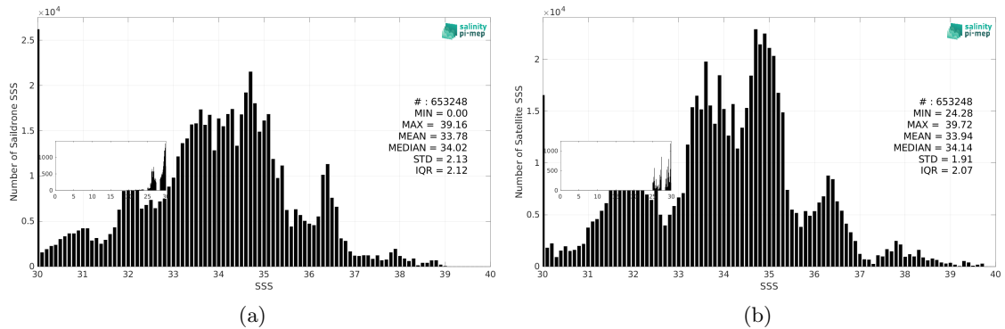
Figure 3: Histograms of SSS from Sailldrone (a) and SMOS SSS L4 OI v346 - Weekly (CMEMS-CATDS-LOPS) (b) considering all match-up pairs per bins of 0.1 over the Global Ocean Pi-MEP region and for the full satellite product period.
