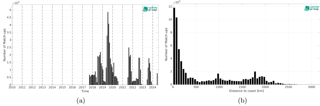
Figure 2: Number of match-ups between Sailldrone and SMOS SSS L4 OI v346 - Weekly (CMEMS-CATDS-LOPS) SSS as a function of time (a) and as function of the distance to coast (b) over the Global Ocean Pi-MEP region and for the full satellite product period.
