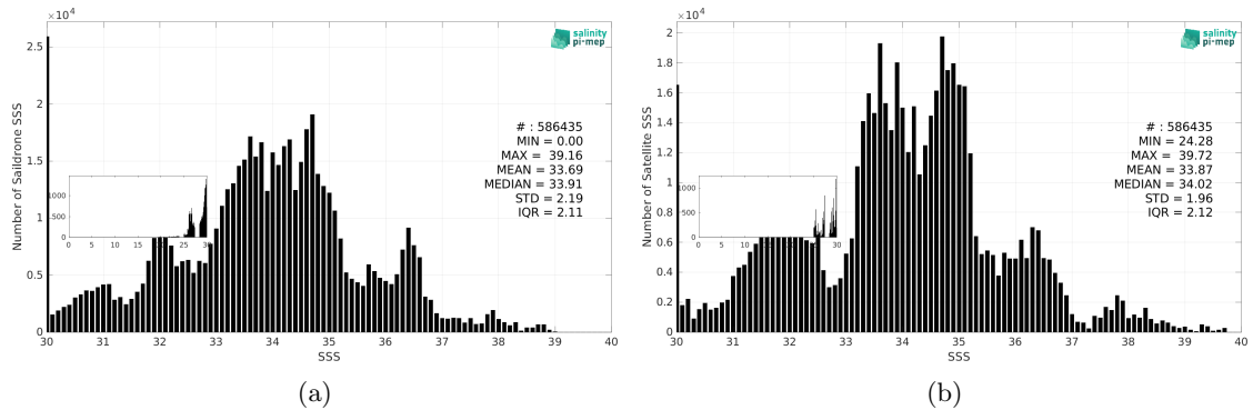
Figure 3: Histograms of SSS from Saildrone (a) and SMOS SSS L4 OI v346 - Weekly (CMEMS-CATDS-LOPS) (b) considering all match-up pairs per bins of 0.1 over the Global Ocean Pi-MEP region and for the full satellite product period.
