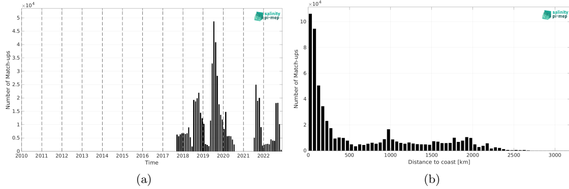
Figure 2: Number of match-ups between Saildrone and SMOS SSS L4 OI v346 - Weekly (CMEMS-CATDS-LOPS) SSS as a function of time (a) and as function of the distance to coast (b) over the Global Ocean Pi-MEP region and for the full satellite product period.
