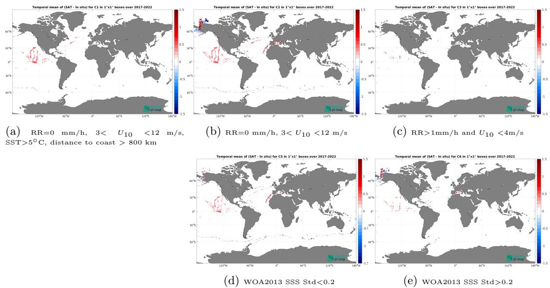
Figure 14: Temporal mean gridded over spatial boxes of size 1^\circ \times 1^\circ of \Delta SSS (SMOS SSS L4 OI v346 - Weekly (CMEMS-CATDS-LOPS) - Saildrone) for 5 different subdatasets corresponding to: RR=0 mm/h, 3 < U_{10} < 12 m/s, SST > 5^\circ\text{C} , distance to coast > 800 km (a), RR=0 mm/h, 3 < U_{10} < 12 m/s (b), RR > 1 mm/h and U_{10} < 4 m/s (c), WOA2013 SSS Std < 0.2 (d), WOA2013 SSS Std > 0.2 (e).
