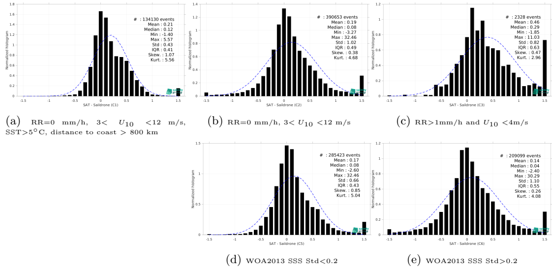
Figure 15: Normalized histogram of \Delta SSS (SMOS SSS L4 OI v346 - Weekly (CMEMS-CATDS-LOPS) - Saiddrone) for 5 different subdatasets corresponding to: RR=0 mm/h, 3 < U_{10} < 12 m/s, SST>5°C, distance to coast > 800 km (a), RR=0 mm/h, 3 < U_{10} < 12 m/s (b), RR>1mm/h and U_{10} < 4 m/s (c), WOA2013 SSS Std<0.2 (d), WOA2013 SSS Std>0.2 (e).
