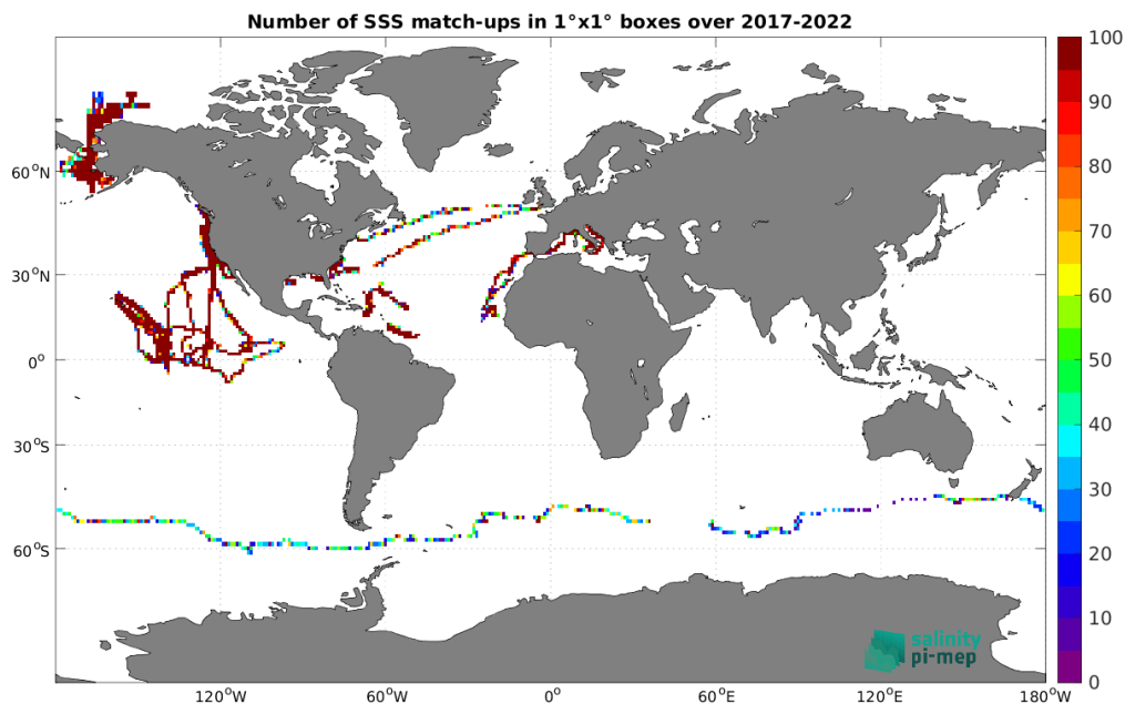
Figure 5: Number of SSS match-ups between Saildrone SSS and the SMOS SSS L4 OI v346 - Weekly (CMEMS-CATDS-LOPS) SSS product for the Global Ocean Pi-MEP region over 1^\circ \times 1^\circ boxes and for the full satellite product period.
