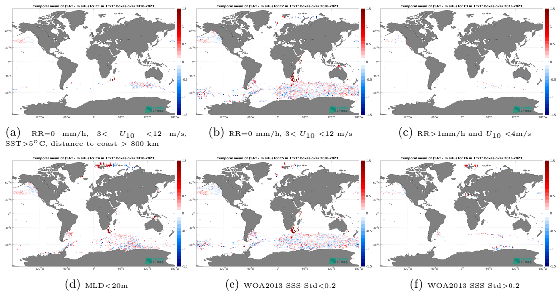
Figure 14: Temporal mean gridded over spatial boxes of size 1^\circ \times 1^\circ of \Delta\text{SSS} (SMOS SSS L4 OI v346 - Weekly (CMEMS-CATDS-LOPS) - Marine mammals) for 6 different subdatasets corresponding to:RR=0 mm/h, 3 < U_{10} < 12 m/s, SST>5°C, distance to coast > 800 km (a), RR=0 mm/h, 3 < U_{10} < 12 m/s (b), RR>1mm/h and U_{10} < 4 m/s (c),MLD<20m (d),WOA2013 SSS Std<0.2 (e),WOA2013 SSS Std>0.2 (f).
