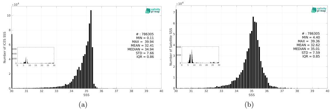
Figure 3: Histograms of SSS from ICES (a) and SMOS SSS L4 OI v346 - Weekly (CMEMS-CATDS-LOPS) (b) considering all match-up pairs per bins of 0.1 over the Global Ocean Pi-MEP region and for the full satellite product period.
