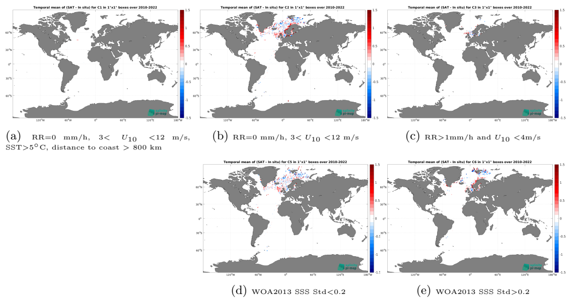
Figure 14: Temporal mean gridded over spatial boxes of size 1^\circ \times 1^\circ of \Delta SSS (SMOS SSS L4 OI v346 - Weekly (CMEMS-CATDS-LOPS) - ICES) for 5 different subdatasets corresponding to: RR=0 mm/h, 3 < U_{10} < 12 m/s, SST > 5^\circ\text{C} , distance to coast > 800 km (a), RR=0 mm/h, 3 < U_{10} < 12 m/s (b), RR > 1 mm/h and U_{10} < 4 m/s (c), WOA2013 SSS Std < 0.2 (d), WOA2013 SSS Std > 0.2 (e).
