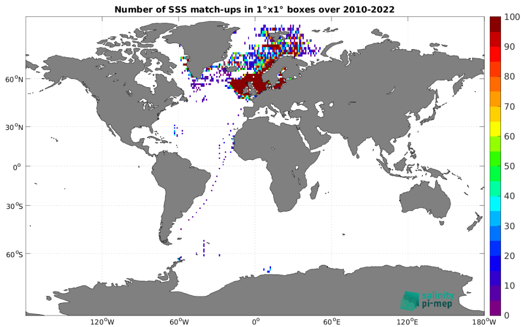
Figure 5: Number of SSS match-ups between ICES SSS and the SMOS SSS L4 OI v346 - Weekly (CMEMS-CATDS-LOPS) SSS product for the Global Ocean Pi-MEP region over 1^\circ \times 1^\circ boxes and for the full satellite product period.
