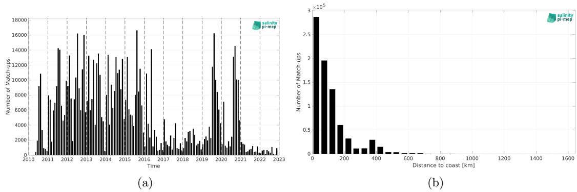
Figure 2: Number of match-ups between ICES and SMOS SSS L4 OI v346 - Weekly (CMEMS-CATDS-LOPS) SSS as a function of time (a) and as function of the distance to coast (b) over the Global Ocean Pi-MEP region and for the full satellite product period.
