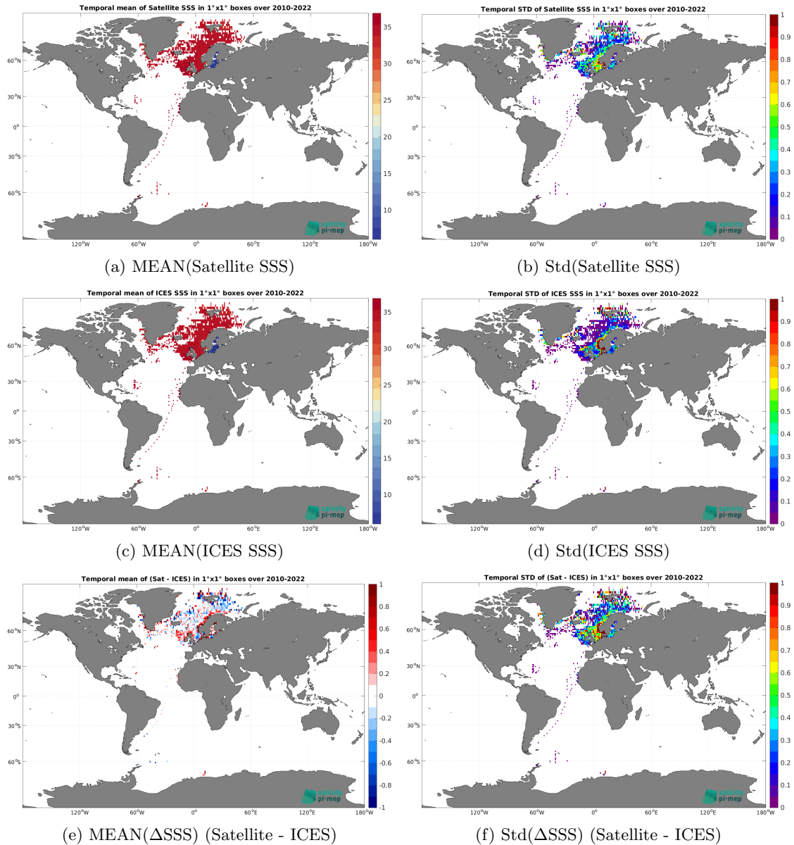
Figure 7: Temporal mean (left) and Std (right) of SSS from SMOS SSS L4 OI v346 - Weekly (CMEMS-CATDS-LOPS) (top), ICES (middle), and of \Delta SSS (Satellite - ICES). Only match-up pairs are used to generate these maps.
