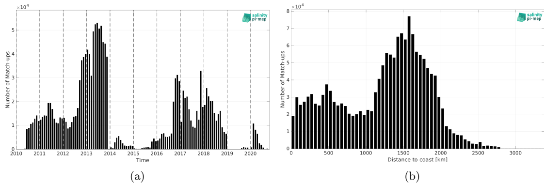
Figure 2: Number of match-ups between Surface drifters and SMOS SSS L4 OI v346 - Weekly (CMEMS-CATDS-LOPS) SSS as a function of time (a) and as function of the distance to coast (b) over the Global Ocean Pi-MEP region and for the full satellite product period.
