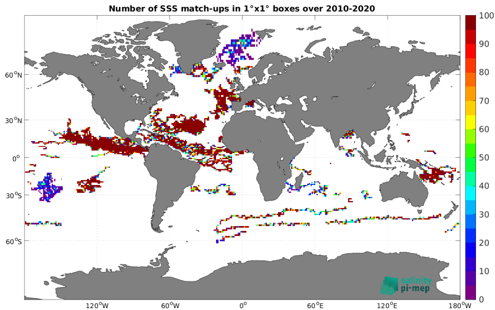
Figure 4: Number of SSS match-ups between Surface drifters SSS and the SMOS SSS L4 OI v346 - Weekly (CMEMS-CATDS-LOPS) SSS product for the Global Ocean Pi-MEP region over 1^\circ \times 1^\circ boxes and for the full satellite product period.
