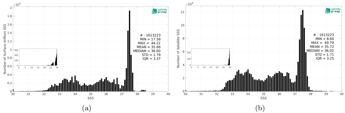
Figure 3: Histograms of SSS from Surface drifters (a) and SMOS SSS L4 OI v346 - Weekly (CMEMS-CATDS-LOPS) (b) considering all match-up pairs per bins of 0.1 over the Global Ocean Pi-MEP region and for the full satellite product period.
