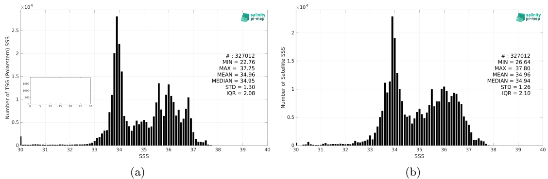
Figure 2: Histograms of SSS from TSG (Polarstern) (a) and SMOS SSS L4 OI v342 - Weekly (CMEMS-CATDS-LOPS) (b) considering all match-up pairs per bins of 0.1 over the Global Ocean Pi-MEP region and for the full satellite product period.
