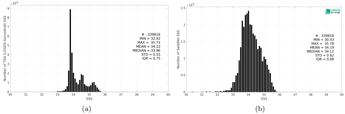
Figure 2: Histograms of SSS from TSG (LEGOS-Survostral) (a) and SMOS SSS L4 OI v342 - Weekly (CMEMS-CATDS-LOPS) (b) considering all match-up pairs per bins of 0.1 over the Global Ocean Pi-MEP region and for the full satellite product period.
