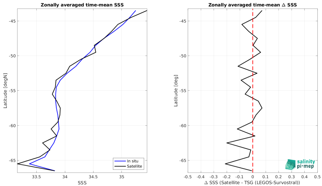
Figure 8: Left panel: Zonal mean SSS from SMOS SSS L4 OI v342 - Weekly (CMEMS-CATDS-LOPS) satellite product (black) and from TSG (LEGOS-Survostral) (blue). Right panel: Zonal mean of \Delta SSS (Satellite - TSG (LEGOS-Survostral)) for all the collected Pi-MEP match-up pairs estimated over the full satellite product period.
