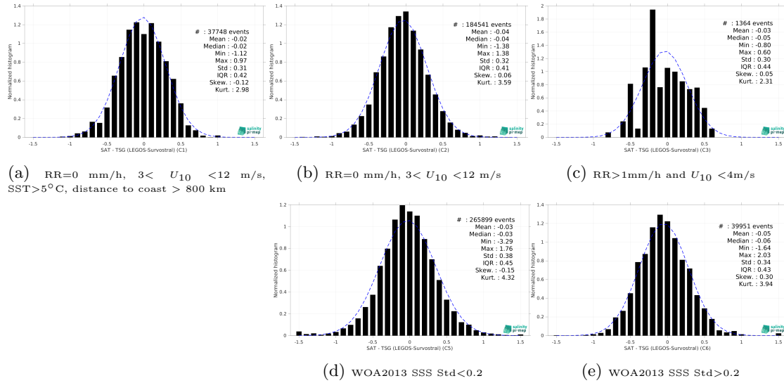
Figure 13: Normalized histogram of \Delta SSS (SMOS SSS L4 OI v342 - Weekly (CMEMS-CATDS-LOPS) - TSG (LEGOS-Survostral)) for 5 different subdatasets corresponding to: RR=0 mm/h, 3 < U_{10} < 12 m/s, SST>5°C, distance to coast > 800 km (a), RR=0 mm/h, 3 < U_{10} < 12 m/s (b), RR>1mm/h and U_{10} < 4 m/s (c), WOA2013 SSS Std<0.2 (d), WOA2013 SSS Std>0.2 (e).
