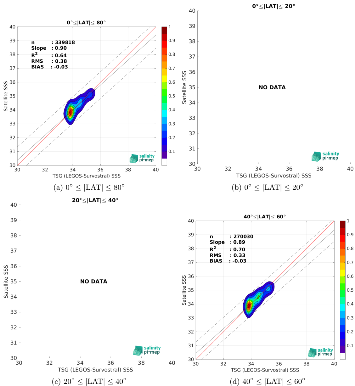
Figure 9: Contour maps of the concentration of SMOS SSS L4 OI v342 - Weekly (CMEMS-CATDS-LOPS) SSS (y-axis) versus TSG (LEGOS-Survostral) SSS (x-axis) at match-up pairs for different latitude bands. For each plot, the red line shows x=y . The black thin and dashed lines indicate a linear fit through the data cloud and the \pm 95\% confidence levels, respectively. The number match-up pairs n , the slope and R^2 coefficient of the linear fit, the root mean square (RMS) and the mean bias between satellite and in situ data are indicated for each latitude band in each plots.
