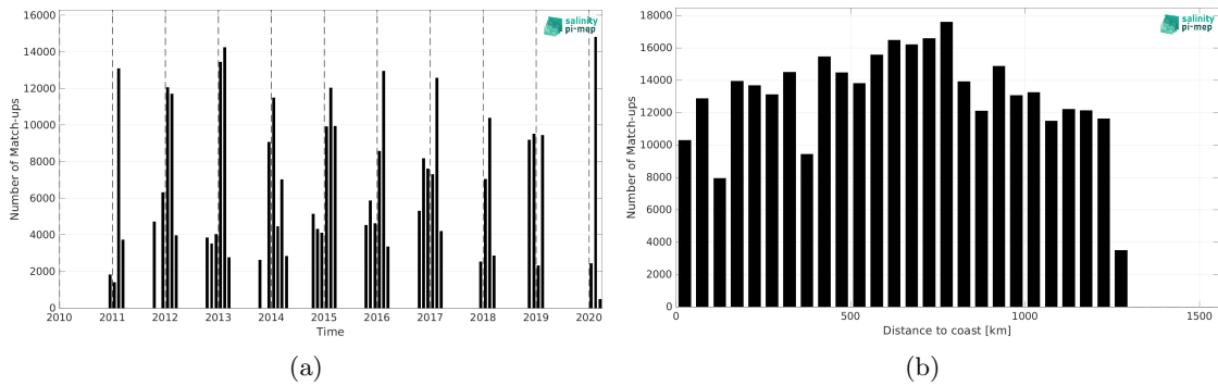
Figure 1: Number of match-ups between TSG (LEGOS-Survostral) and SMOS SSS L4 OI v342 - Weekly (CMEMS-CATDS-LOPS) SSS as a function of time (a) and as function of the distance to coast (b) over the Global Ocean Pi-MEP region and for the full satellite product period.
