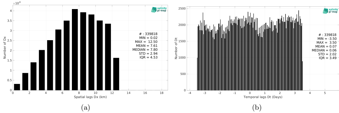
Figure 5: Histograms of the spatial (a) and temporal (b) lags between the location/time of the TSG (LEGOS-Survostral) measurement and the date of the corresponding SMOS SSS L4 OI v342 - Weekly (CMEMS-CATDS-LOPS) SSS pixel.
