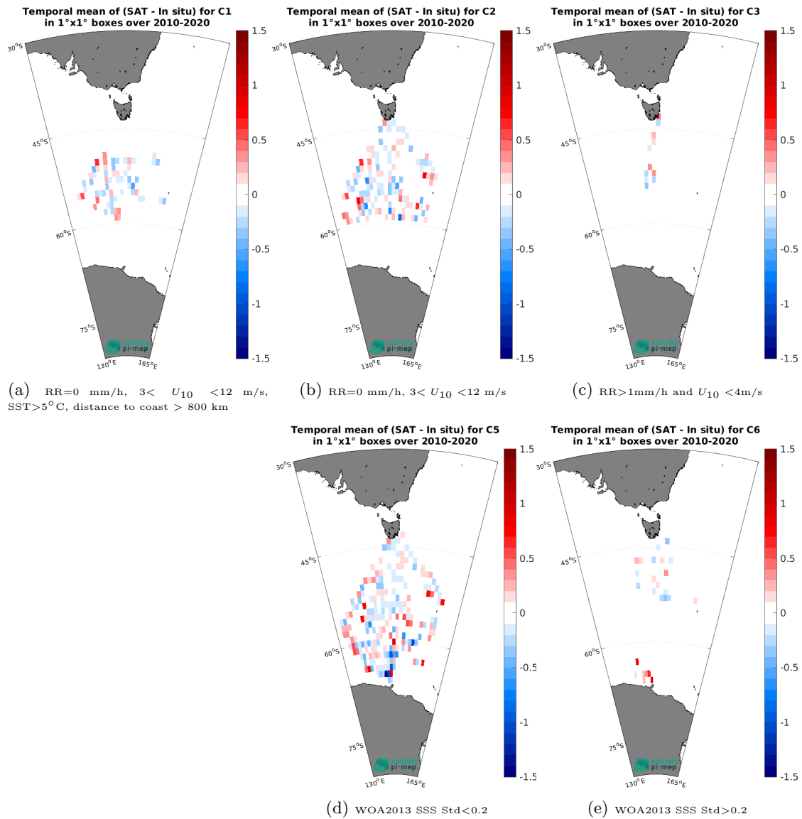
Figure 12: Temporal mean gridded over spatial boxes of size 1^\circ \times 1^\circ of \Delta\text{SSS} (SMOS SSS L4 OI v342 - Weekly (CMEMS-CATDS-LOPS) - TSG (LEGOS-Survostral)) for 5 different subdatasets corresponding to: RR=0 mm/h, 3 < U_{10} < 12 m/s, SST > 5^\circ\text{C} , distance to coast > 800 km (a), RR=0 mm/h, 3 < U_{10} < 12 m/s (b), RR > 1 mm/h and U_{10} < 4 m/s (c), WOA2013 SSS Std < 0.2 (d), WOA2013 SSS Std > 0.2 (e).
