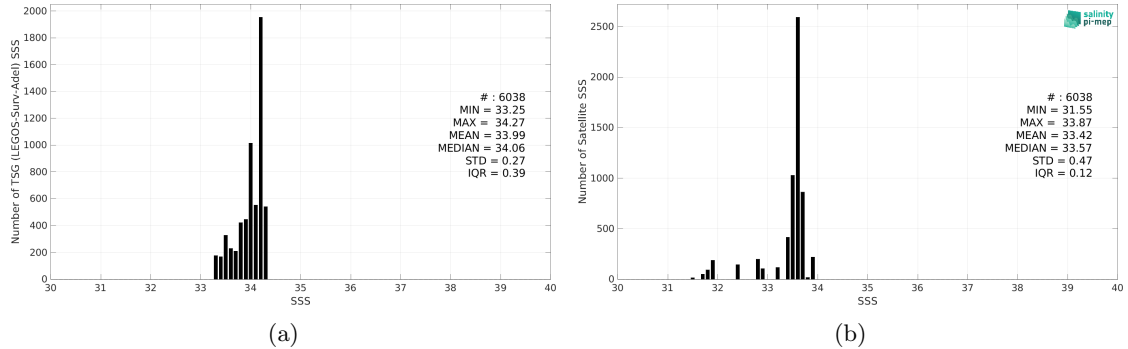
Figure 2: Histograms of SSS from TSG (LEGOS-Surv-Adel) (a) and SMOS SSS L4 OI v342 - Weekly (CMEMS-CATDS-LOPS) (b) considering all match-up pairs per bins of 0.1 over the Global Ocean Pi-MEP region and for the full satellite product period.
