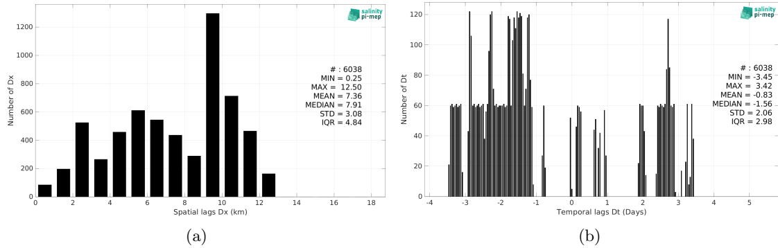
Figure 5: Histograms of the spatial (a) and temporal (b) lags between the location/time of the TSG (LEGOS-Surv-Adel) measurement and the date of the corresponding SMOS SSS L4 OI v342 - Weekly (CMEMS-CATDS-LOPS) SSS pixel.
