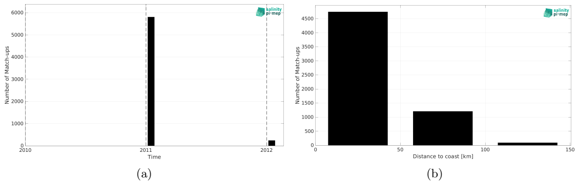
Figure 1: Number of match-ups between TSG (LEGOS-Surv-Adel) and SMOS SSS L4 OI v342 - Weekly (CMEMS-CATDS-LOPS) SSS as a function of time (a) and as function of the distance to coast (b) over the Global Ocean Pi-MEP region and for the full satellite product period.
