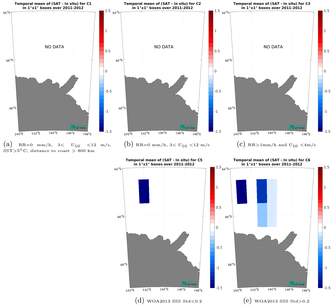
Figure 12: Temporal mean gridded over spatial boxes of size 1^\circ \times 1^\circ of \Delta SSS (SMOS SSS L4 OI v342 - Weekly (CMEMS-CATDS-LOPS) - TSG (LEGOS-Surv-Adel)) for 5 different subdatasets corresponding to: RR=0 mm/h, 3 < U_{10} < 12 m/s, SST>5°C, distance to coast > 800 km (a), RR=0 mm/h, 3 < U_{10} < 12 m/s (b), RR>1mm/h and U_{10} < 4 m/s (c), WOA2013 SSS Std<0.2 (d), WOA2013 SSS Std>0.2 (e).
