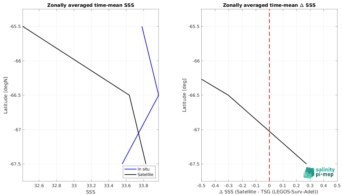
Figure 8: Left panel: Zonal mean SSS from SMOS SSS L4 OI v342 - Weekly (CMEMS-CATDS-LOPS) satellite product (black) and from TSG (LEGOS-Surv-Adel) (blue). Right panel: Zonal mean of \Delta SSS (Satellite - TSG (LEGOS-Surv-Adel)) for all the collected Pi-MEP match-up pairs estimated over the full satellite product period.
