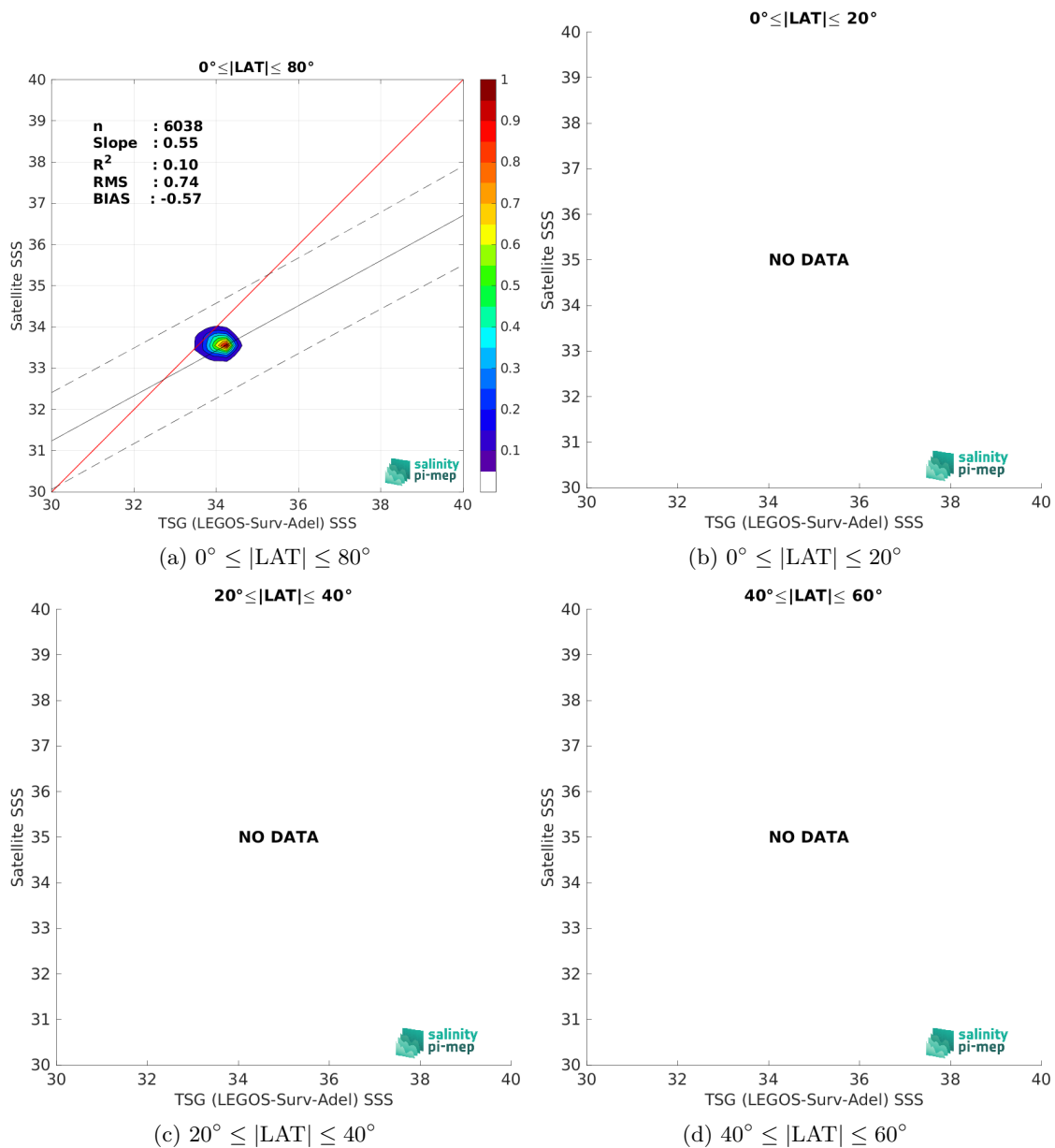
Figure 9: Contour maps of the concentration of SMOS SSS L4 OI v342 - Weekly (CMEMS-CATDS-LOPS) SSS (y-axis) versus TSG (LEGOS-Surv-Adel) SSS (x-axis) at match-up pairs for different latitude bands. For each plot, the red line shows x=y . The black thin and dashed lines indicate a linear fit through the data cloud and the \pm 95\% confidence levels, respectively. The number match-up pairs n , the slope and R^2 coefficient of the linear fit, the root mean square (RMS) and the mean bias between satellite and in situ data are indicated for each latitude band in each plots.
