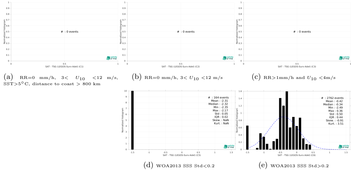
Figure 13: Normalized histogram of \Delta SSS (SMOS SSS L4 OI v342 - Weekly (CMEMS-CATDS-LOPS) - TSG (LEGOS-Surv-Adel)) for 5 different subdatasets corresponding to: RR=0 mm/h, 3 < U_{10} < 12 m/s, SST > 5°C, distance to coast > 800 km (a), RR=0 mm/h, 3 < U_{10} < 12 m/s (b), RR > 1mm/h and U_{10} < 4 m/s (c), WOA2013 SSS Std < 0.2 (d), WOA2013 SSS Std > 0.2 (e).
