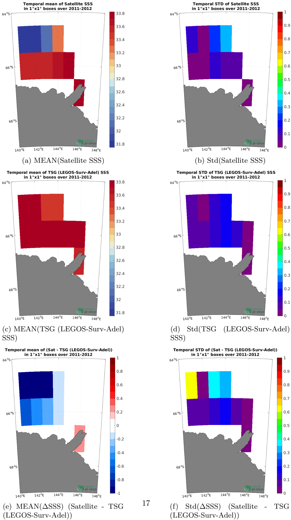
Figure 6: Temporal mean (left) and Std (right) of SSS from SMOS SSS L4 OI v342 - Weekly (CMEMS-CATDS-LOPS) (top), TSG (LEGOS-Surv-Adel) (middle), and of \Delta SSS (Satellite - TSG (LEGOS-Surv-Adel)). Only match-up pairs are used to generate these maps.
