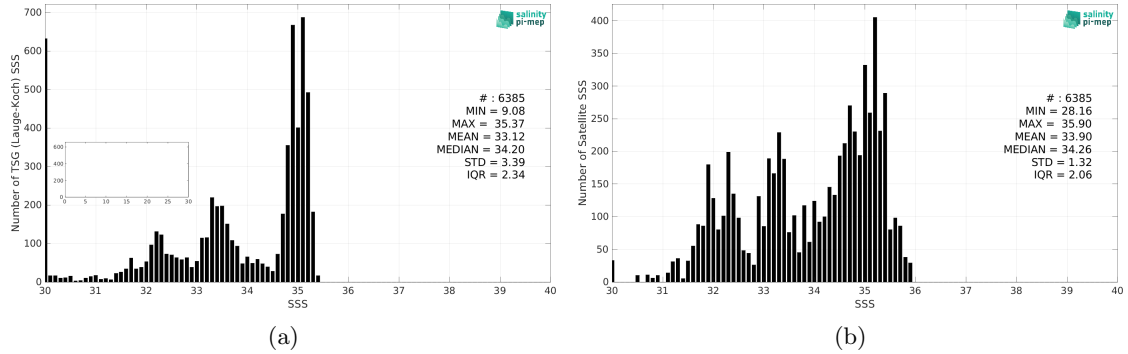
Figure 2: Histograms of SSS from TSG (Lauge-Koch) (a) and SMOS SSS L4 OI v342 - Weekly (CMEMS-CATDS-LOPS) (b) considering all match-up pairs per bins of 0.1 over the Global Ocean Pi-MEP region and for the full satellite product period.
