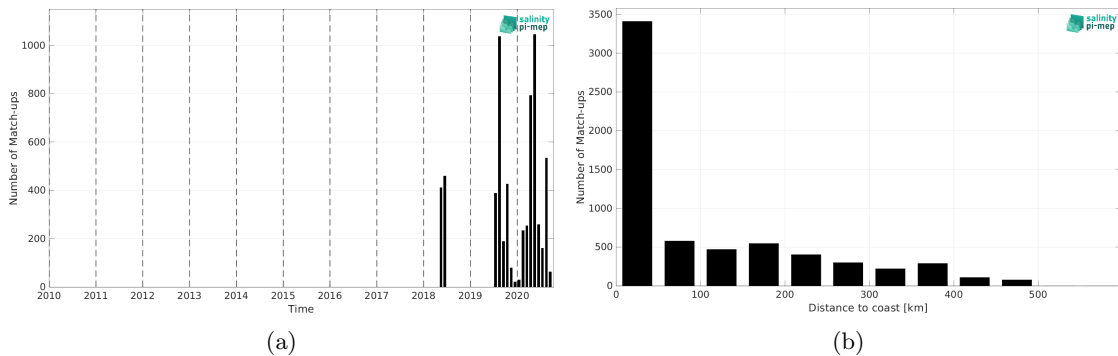
Figure 1: Number of match-ups between TSG (Lauge-Koch) and SMOS SSS L4 OI v342 - Weekly (CMEMS-CATDS-LOPS) SSS as a function of time (a) and as function of the distance to coast (b) over the Global Ocean Pi-MEP region and for the full satellite product period.
