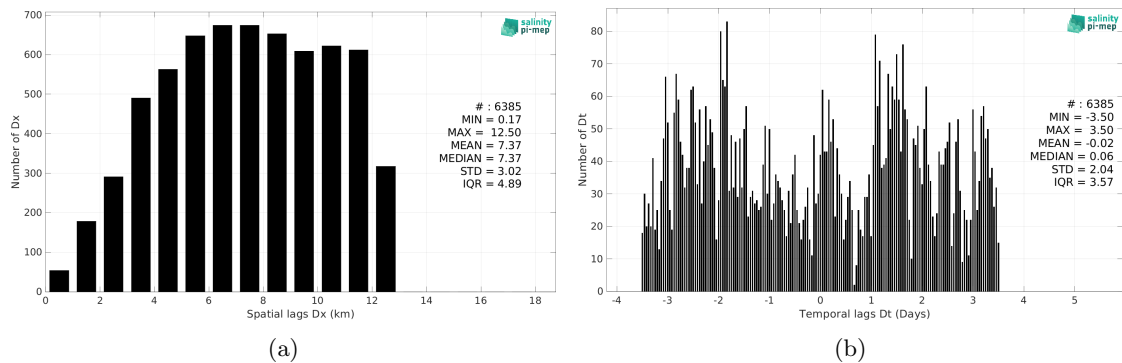
Figure 5: Histograms of the spatial (a) and temporal (b) lags between the location/time of the TSG (Lauge-Koch) measurement and the date of the corresponding SMOS SSS L4 OI v342 - Weekly (CMEMS-CATDS-LOPS) SSS pixel.
