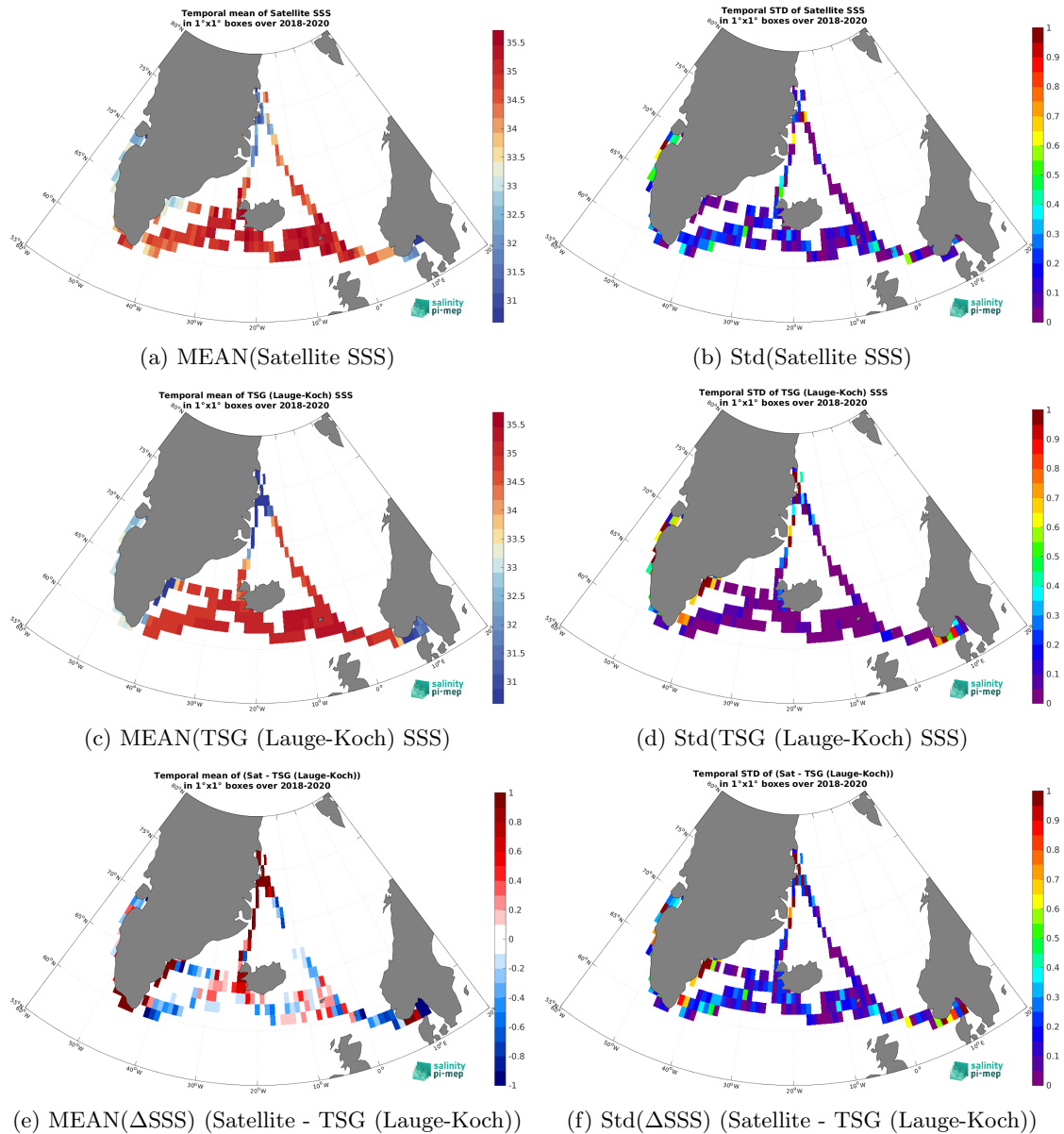
Figure 6: Temporal mean (left) and Std (right) of SSS from SMOS SSS L4 OI v342 - Weekly (CMEMS-CATDS-LOPS) (top), TSG (Lauge-Koch) (middle), and of \Delta SSS (Satellite - TSG (Lauge-Koch)). Only match-up pairs are used to generate these maps.
