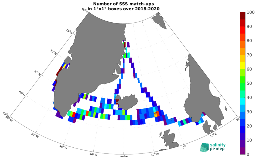
Figure 4: Number of SSS match-ups between TSG (Lauge-Koch) SSS and the SMOS SSS L4 OI v342 - Weekly (CMEMS-CATDS-LOPS) SSS product for the Global Ocean Pi-MEP region over 1^\circ \times 1^\circ boxes and for the full satellite product period.
