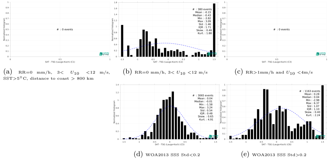
Figure 13: Normalized histogram of \Delta SSS (SMOS SSS L4 OI v342 - Weekly (CMEMS-CATDS-LOPS) - TSG (Lauge-Koch)) for 5 different subdatasets corresponding to: RR=0 mm/h, 3 < U_{10} < 12 m/s, SST > 5°C, distance to coast > 800 km (a), RR=0 mm/h, 3 < U_{10} < 12 m/s (b), RR > 1mm/h and U_{10} < 4 m/s (c), WOA2013 SSS Std < 0.2 (d), WOA2013 SSS Std > 0.2 (e).
