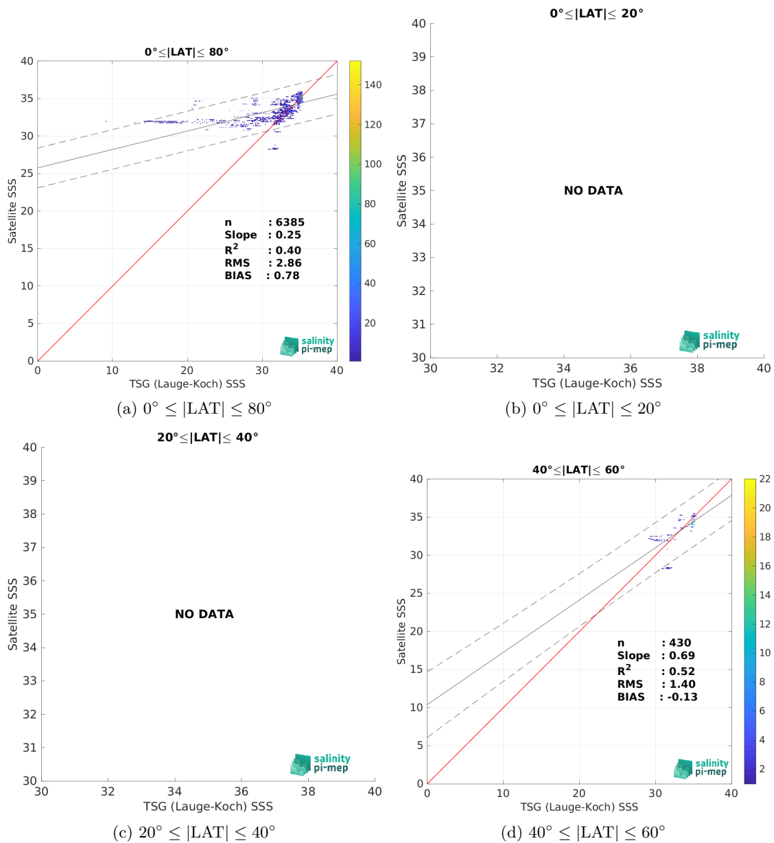
Figure 9: Contour maps of the concentration of SMOS SSS L4 OI v342 - Weekly (CMEMS-CATDS-LOPS) SSS (y-axis) versus TSG (Lauge-Koch) SSS (x-axis) at match-up pairs for different latitude bands. For each plot, the red line shows x=y . The black thin and dashed lines indicate a linear fit through the data cloud and the \pm 95\% confidence levels, respectively. The number match-up pairs n , the slope and R^2 coefficient of the linear fit, the root mean square (RMS) and the mean bias between satellite and in situ data are indicated for each latitude band in each plots.
