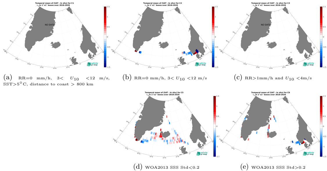
Figure 12: Temporal mean gridded over spatial boxes of size 1^{\circ}\times 1^{\circ} of \Delta\text{SSS} (SMOS SSS L4 OI v342 - Weekly (CMEMS-CATDS-LOPS) - TSG (Lauge-Koch)) for 5 different subdatasets corresponding to:RR=0 mm/h, 3 < U_{10} < 12 m/s, SST >5^{\circ}\text{C} , distance to coast > 800 km (a), RR=0 mm/h, 3 < U_{10} < 12 m/s (b), RR >1 mm/h and U_{10} < 4 m/s (c), WOA2013 SSS Std <0.2 (d), WOA2013 SSS Std >0.2 (e).
