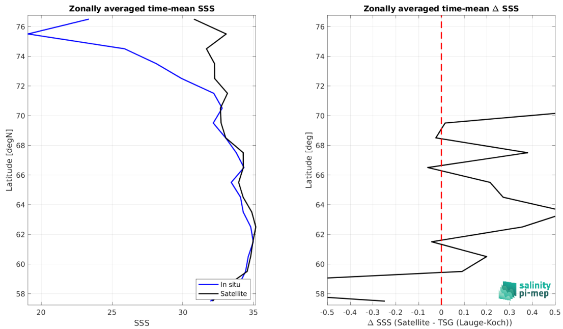
Figure 8: Left panel: Zonal mean SSS from SMOS SSS L4 OI v342 - Weekly (CMEMS-CATDS-LOPS) satellite product (black) and from TSG (Lauge-Koch) (blue). Right panel: Zonal mean of \Delta SSS (Satellite - TSG (Lauge-Koch)) for all the collected Pi-MEP match-up pairs estimated over the full satellite product period.
