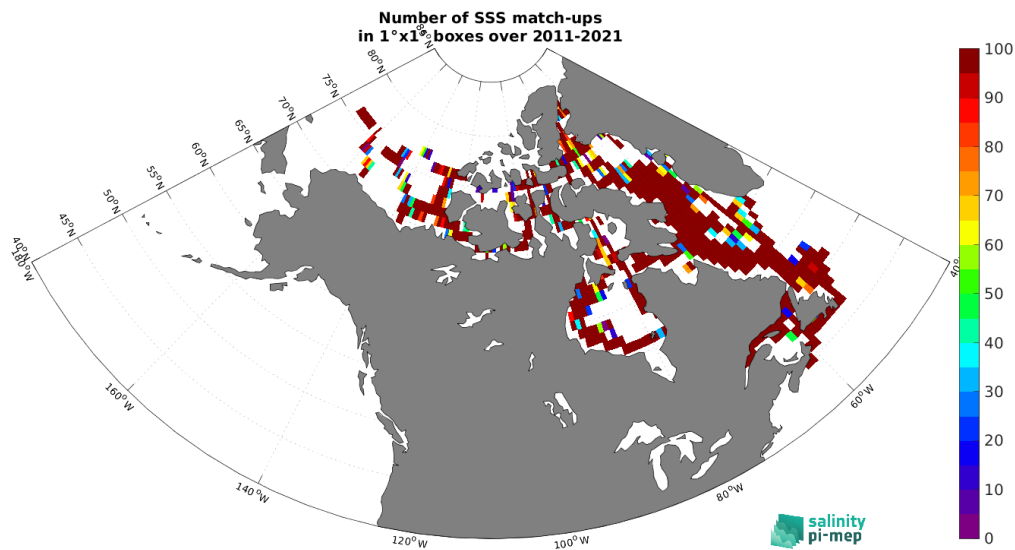
Figure 4: Number of SSS match-ups between TSG (Amundsen) SSS and the SMOS SSS L4 OI v342 - Weekly (CMEMS-CATDS-LOPS) SSS product for the Global Ocean Pi-MEP region over 1^\circ \times 1^\circ boxes and for the full satellite product period.
