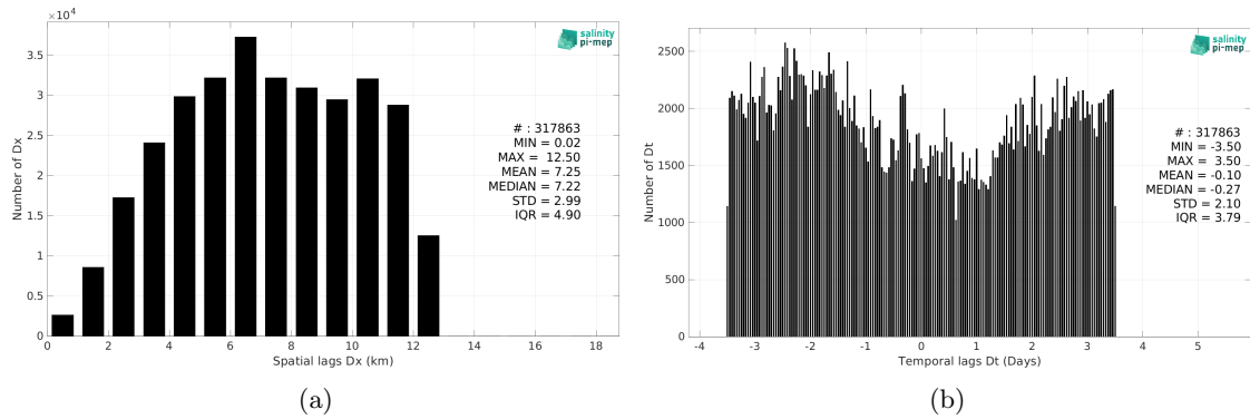
Figure 5: Histograms of the spatial (a) and temporal (b) lags between the location/time of the TSG (Amundsen) measurement and the date of the corresponding SMOS SSS L4 OI v342 - Weekly (CMEMS-CATDS-LOPS) SSS pixel.
