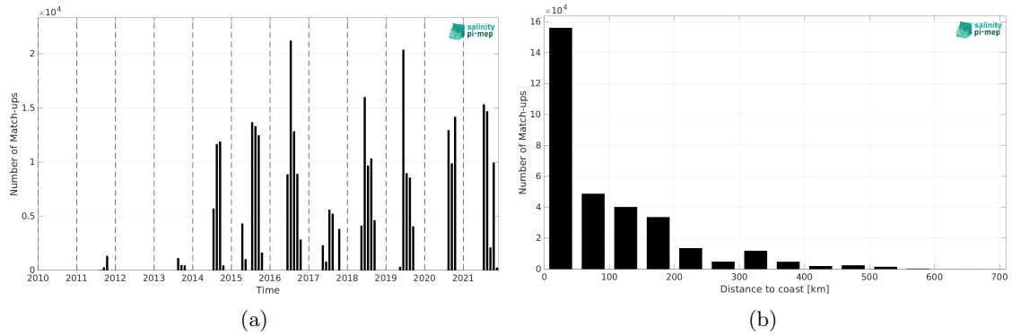
Figure 1: Number of match-ups between TSG (Amundsen) and SMOS SSS L4 OI v342 - Weekly (CMEMS-CATDS-LOPS) SSS as a function of time (a) and as function of the distance to coast (b) over the Global Ocean Pi-MEP region and for the full satellite product period.
