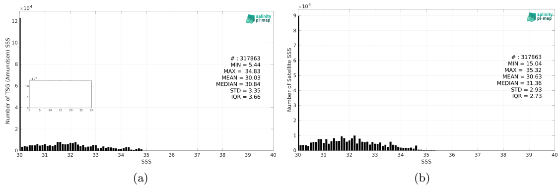
Figure 2: Histograms of SSS from TSG (Amundsen) (a) and SMOS SSS L4 OI v342 - Weekly (CMEMS-CATDS-LOPS) (b) considering all match-up pairs per bins of 0.1 over the Global Ocean Pi-MEP region and for the full satellite product period.
