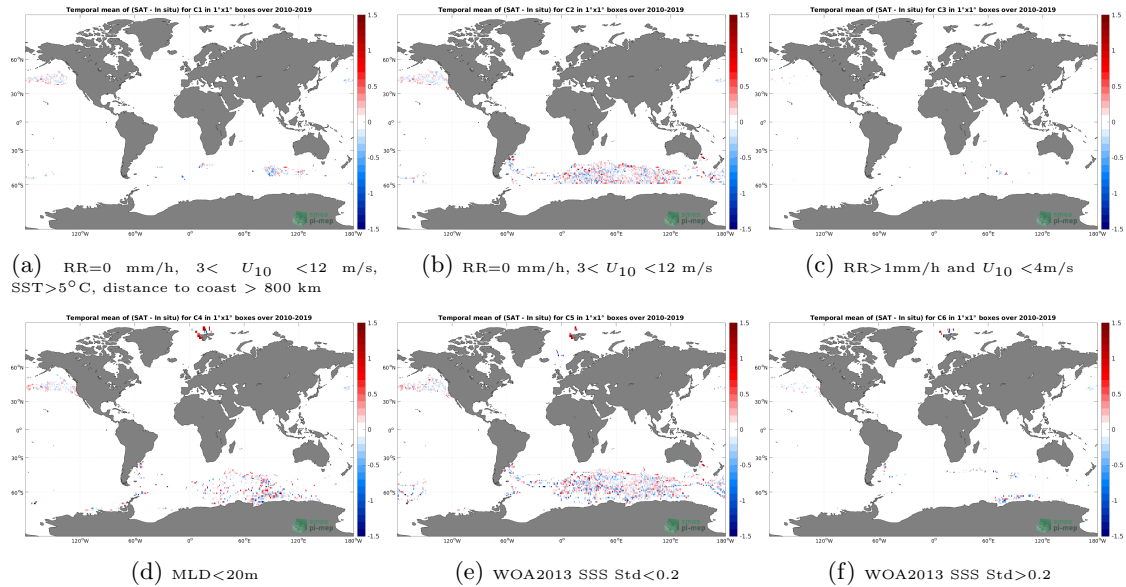
Figure 12: Temporal mean gridded over spatial boxes of size 1^{\circ}\times 1^{\circ} of \Delta\text{SSS} (SMOS SSS L4 OI v342 - Weekly (CMEMS-CATDS-LOPS) - Marine mammals) for 6 different subdatasets corresponding to:RR=0 mm/h, 3 < U_{10} < 12 m/s, SST > 5^{\circ}\text{C} , distance to coast > 800 km (a), RR=0 mm/h, 3 < U_{10} < 12 m/s (b), RR > 1\text{mm/h} and U_{10} < 4\text{m/s} (c),MLD < 20\text{m} (d),WOA2013 SSS Std < 0.2 (e),WOA2013 SSS Std > 0.2 (f).
