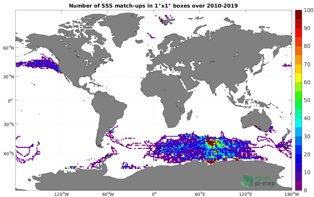
Figure 4: Number of SSS match-ups between Marine mammals SSS and the SMOS SSS L4 OI v342 - Weekly (CMEMS-CATDS-LOPS) SSS product for the Global Ocean Pi-MEP region over 1^\circ \times 1^\circ boxes and for the full satellite product period.
