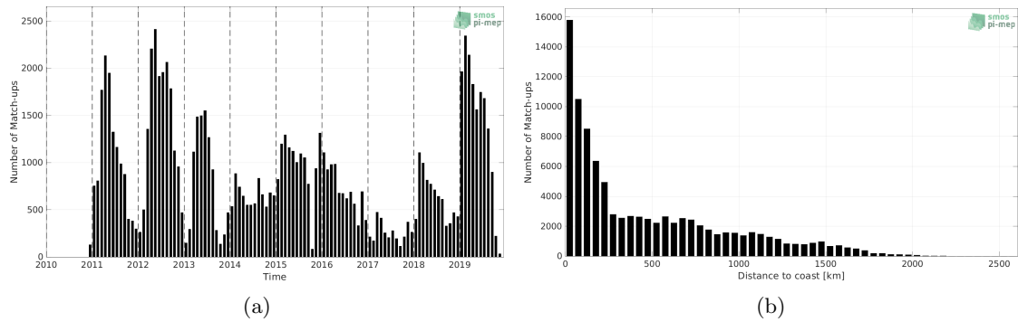
Figure 1: Number of match-ups between Marine mammals and SMOS SSS L4 OI v342 - Weekly (CMEMS-CATDS-LOPS) SSS as a function of time (a) and as function of the distance to coast (b) over the Global Ocean Pi-MEP region and for the full satellite product period.
