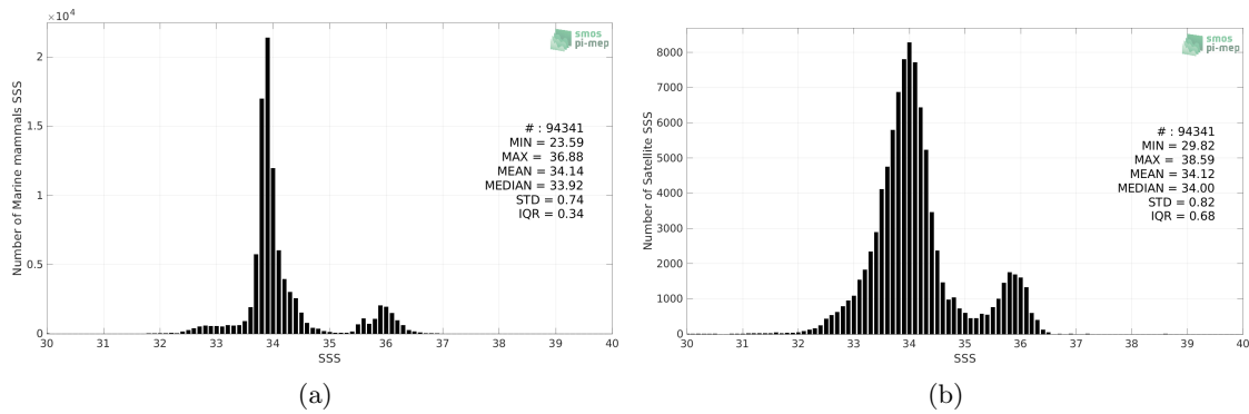
Figure 2: Histograms of SSS from Marine mammals (a) and SMOS SSS L4 OI v342 - Weekly (CMEMS-CATDS-LOPS) (b) considering all match-up pairs per bins of 0.1 over the Global Ocean Pi-MEP region and for the full satellite product period.
