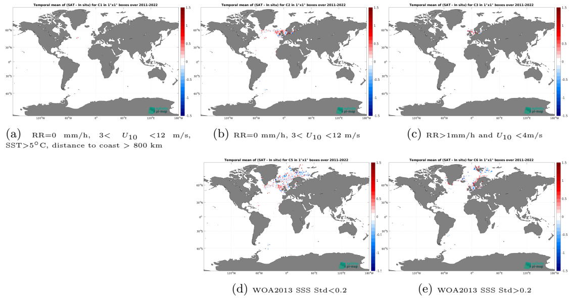
Figure 12: Temporal mean gridded over spatial boxes of size 1^\circ \times 1^\circ of \Delta SSS (SMOS SSS L4 OI v342 - Weekly (CMEMS-CATDS-LOPS) - ICES) for 5 different subdatasets corresponding to: RR=0 mm/h, 3 < U_{10} < 12 m/s, SST > 5^\circ\text{C} , distance to coast > 800 km (a), RR=0 mm/h, 3 < U_{10} < 12 m/s (b), RR > 1 mm/h and U_{10} < 4 m/s (c), WOA2013 SSS Std < 0.2 (d), WOA2013 SSS Std > 0.2 (e).
