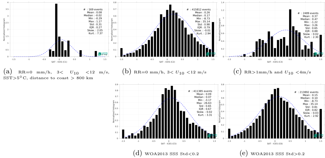
Figure 13: Normalized histogram of \Delta SSS (SMOS SSS L4 OI v342 - Weekly (CMEMS-CATDS-LOPS) - ICES) for 5 different subdatasets corresponding to: RR=0 mm/h, 3 < U_{10} < 12 m/s, SST>5°C, distance to coast > 800 km (a), RR=0 mm/h, 3 < U_{10} < 12 m/s (b), RR>1mm/h and U_{10} < 4 m/s (c), WOA2013 SSS Std<0.2 (d), WOA2013 SSS Std>0.2 (e).
