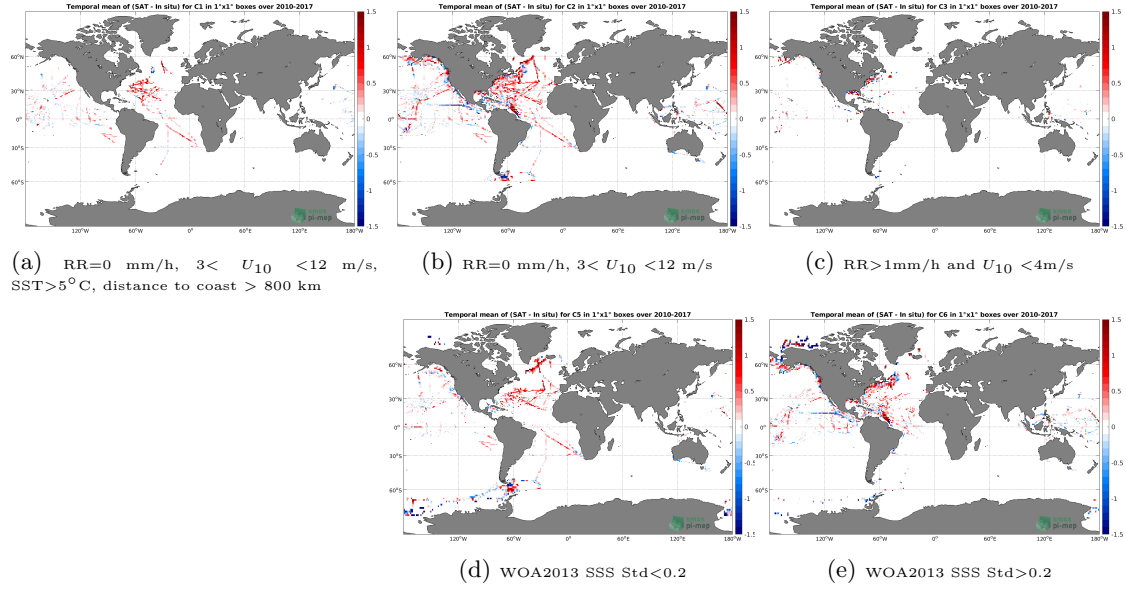
Figure 12: Temporal mean gridded over spatial boxes of size 1^\circ \times 1^\circ of \Delta SSS (SMOS L4 v2 Weekly (CATDS-CECOS-IFREMER) - TSG (SAMOS)) for 5 different subdatasets corresponding to:RR=0 mm/h, 3 < U_{10} < 12 m/s, SST >5^\circ C, distance to coast > 800 km (a), RR=0 mm/h, 3 < U_{10} < 12 m/s (b), RR >1 mm/h and U_{10} < 4 m/s (c), WOA2013 SSS Std <0.2 (d), WOA2013 SSS Std >0.2 (e).
