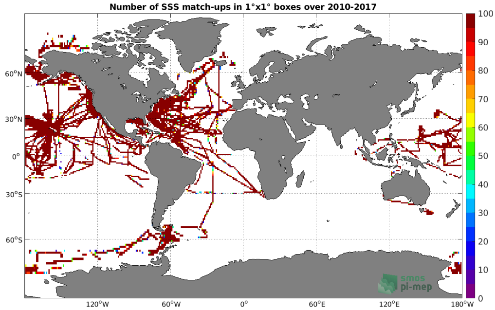
Figure 4: Number of SSS match-ups between TSG (SAMOS) SSS and the SMOS L4 v2 Weekly (CATDS-CECOS-IFREMER) SSS product for the Global Ocean Pi-MEP region over 1^\circ \times 1^\circ boxes and for the full satellite product period.
