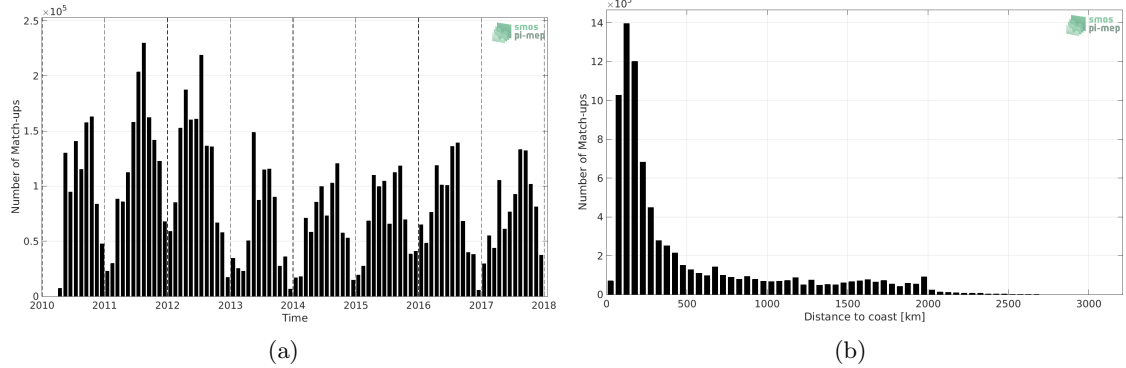
Figure 1: Number of match-ups between TSG (SAMOS) and SMOS L4 v2 Weekly (CATDS-CECOS-IFREMER) SSS as a function of time (a) and as function of the distance to coast (b) over the Global Ocean Pi-MEP region and for the full satellite product period.
