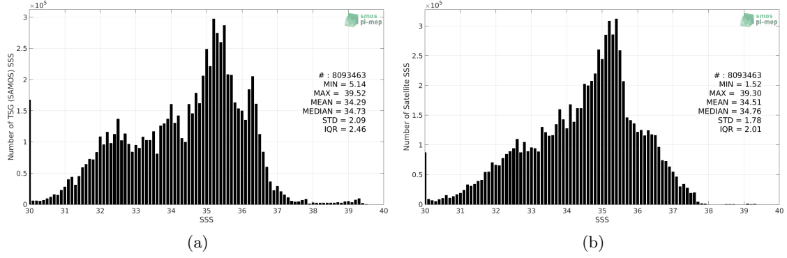
Figure 2: Histograms of SSS from TSG (SAMOS) (a) and SMOS L4 v2 Weekly (CATDS-CECOS-IFREMER) (b) considering all match-up pairs per bins of 0.1 over the Global Ocean Pi-MEP region and for the full satellite product period.
