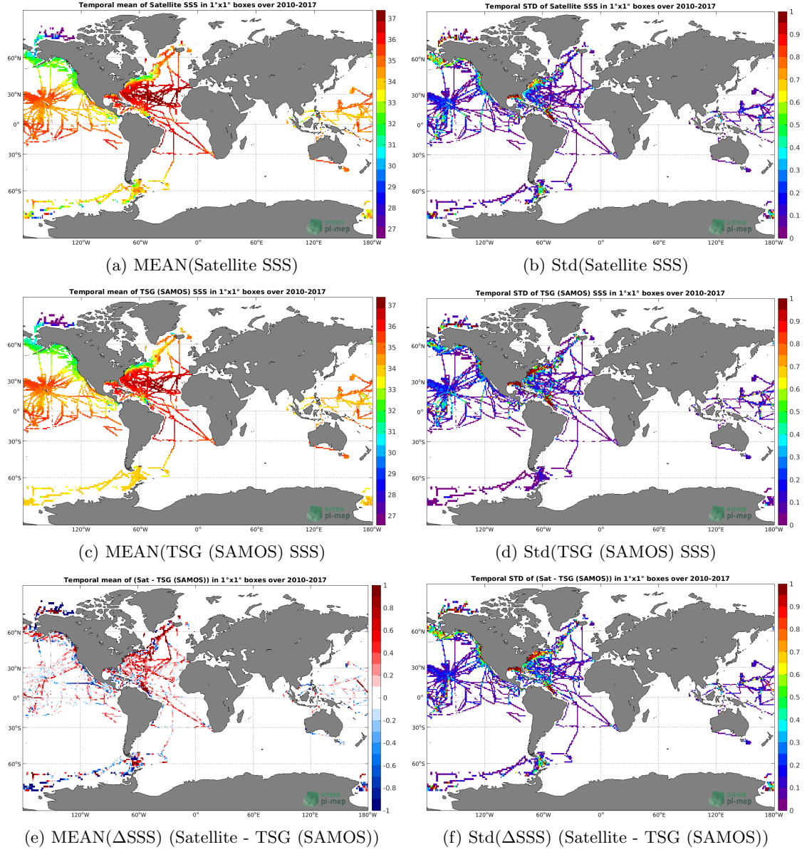
Figure 6: Temporal mean (left) and Std (right) of SSS from SMOS L4 v2 Weekly (CATDS-CECOS-IFREMER) (top), TSG (SAMOS) (middle), and of \Delta SSS (Satellite - TSG (SAMOS)). Only match-up pairs are used to generate these maps.
