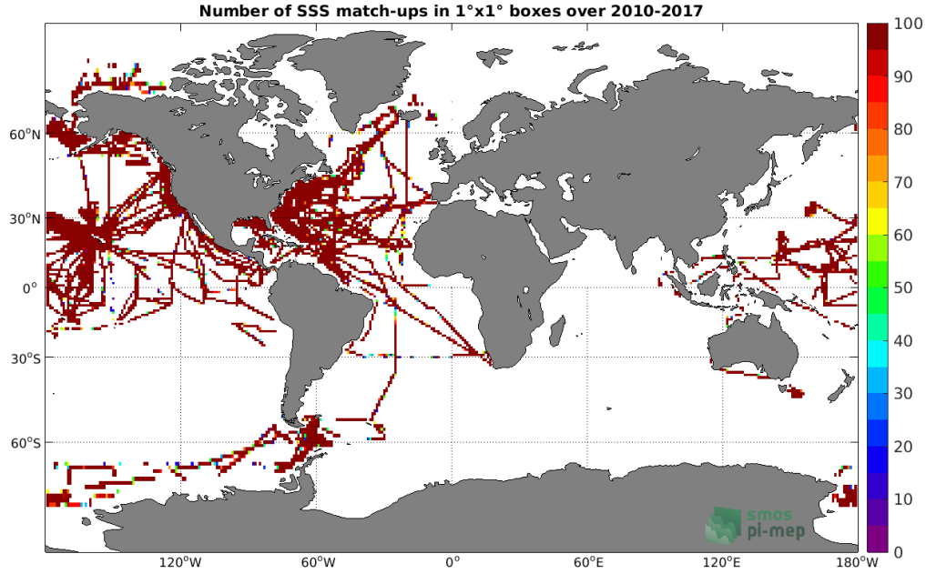
Figure 4: Number of SSS match-ups between TSG (SAMOS) SSS and the SMOS L4 v2 Weekly (CATDS-CECOS-IFREMER) SSS product for the Global Ocean Pi-MEP region over 1^\circ \times 1^\circ boxes and for the full satellite product period.
