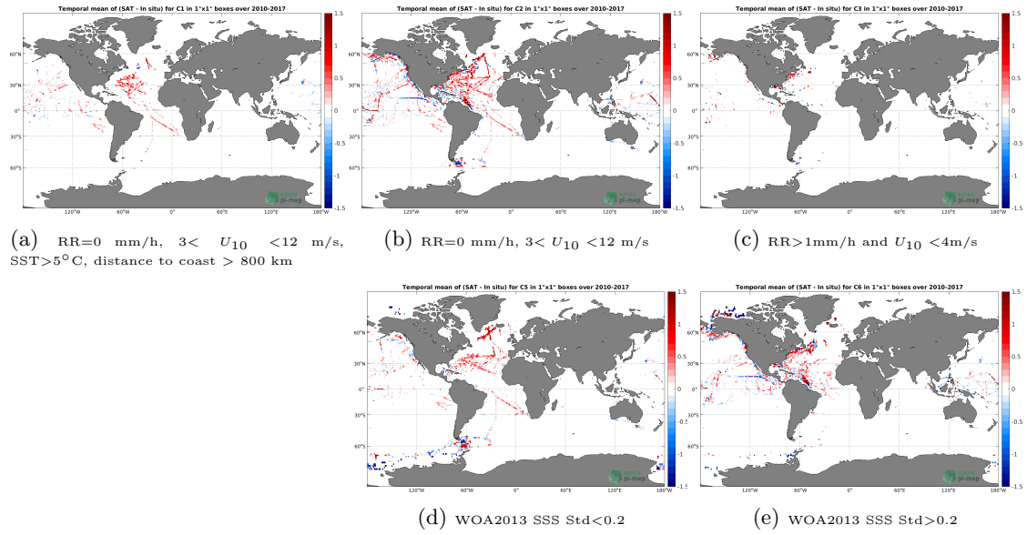
Figure 12: Temporal mean gridded over spatial boxes of size 1^\circ \times 1^\circ of \Delta SSS (SMOS L4 v2 Weekly (CATDS-CECOS-IFREMER) - TSG (SAMOS)) for 5 different subdatasets corresponding to: RR=0 mm/h, 3 < U_{10} < 12 m/s, SST > 5^\circ\text{C} , distance to coast > 800 km (a), RR=0 mm/h, 3 < U_{10} < 12 m/s (b), RR > 1 mm/h and U_{10} < 4 m/s (c), WOA2013 SSS Std < 0.2 (d), WOA2013 SSS Std > 0.2 (e).
