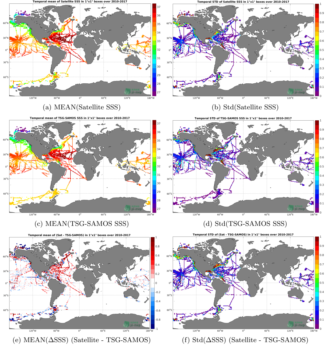
Figure 6: Temporal mean (left) and Std (right) of SSS from SMOS-L4-CATDS-CECOS-IFREMER-V2-WEEKLY-0.5DEG (top), TSG-SAMOS (middle), and of ΔSSS (Satellite - TSG-SAMOS). Only match-up pairs are used to generate these maps.
