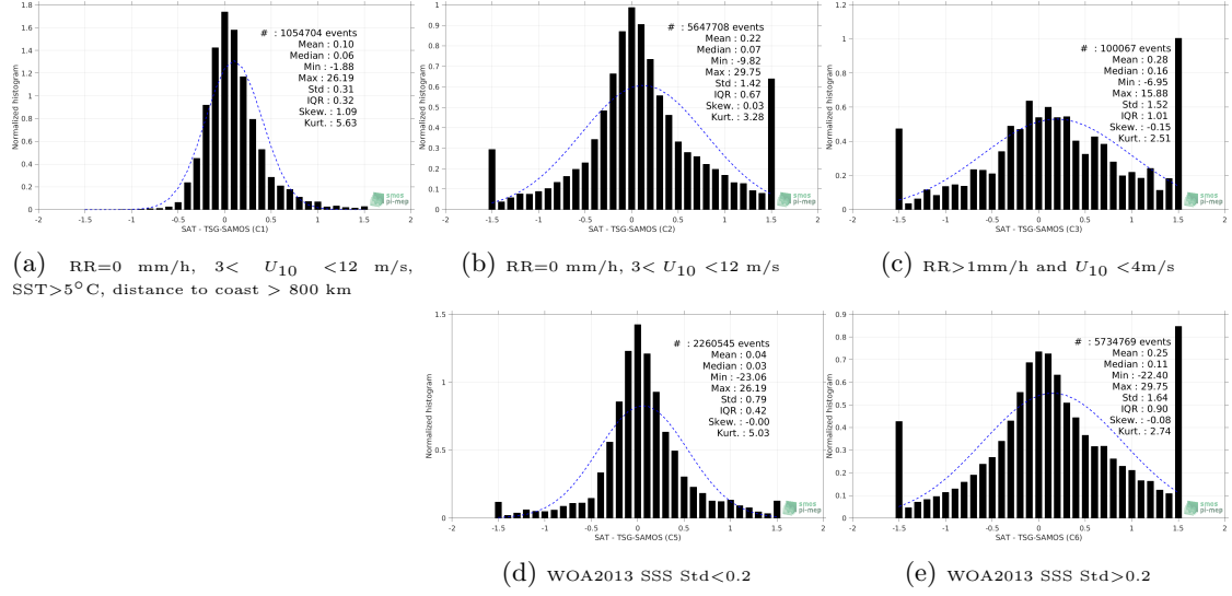
Figure 13: Normalized histogram of \Delta\text{SSS} (SMOS-L4-CATDS-CECOS-IFREMER-V2-WEEKLY-0.5DEG - TSG-SAMOS) for 5 different subdatasets corresponding to: RR=0 mm/h, 3 < U_{10} < 12 m/s, SST >5^{\circ}\text{C} , distance to coast > 800 km (a), RR=0 mm/h, 3 < U_{10} < 12 m/s (b), RR>1\text{mm/h} and U_{10} < 4\text{m/s} (c), WOA2013 SSS Std <0.2 (d), WOA2013 SSS Std >0.2 (e).
