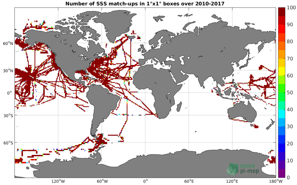
Figure 4: Number of SSS match-ups between TSG-SAMOS SSS and the SMOS-L4-CATDS-CECOS-IFREMER-V2-WEEKLY-0.5DEG SSS product for the Global Ocean Pi-MEP region over 1^\circ \times 1^\circ boxes and for the full satellite product period.
