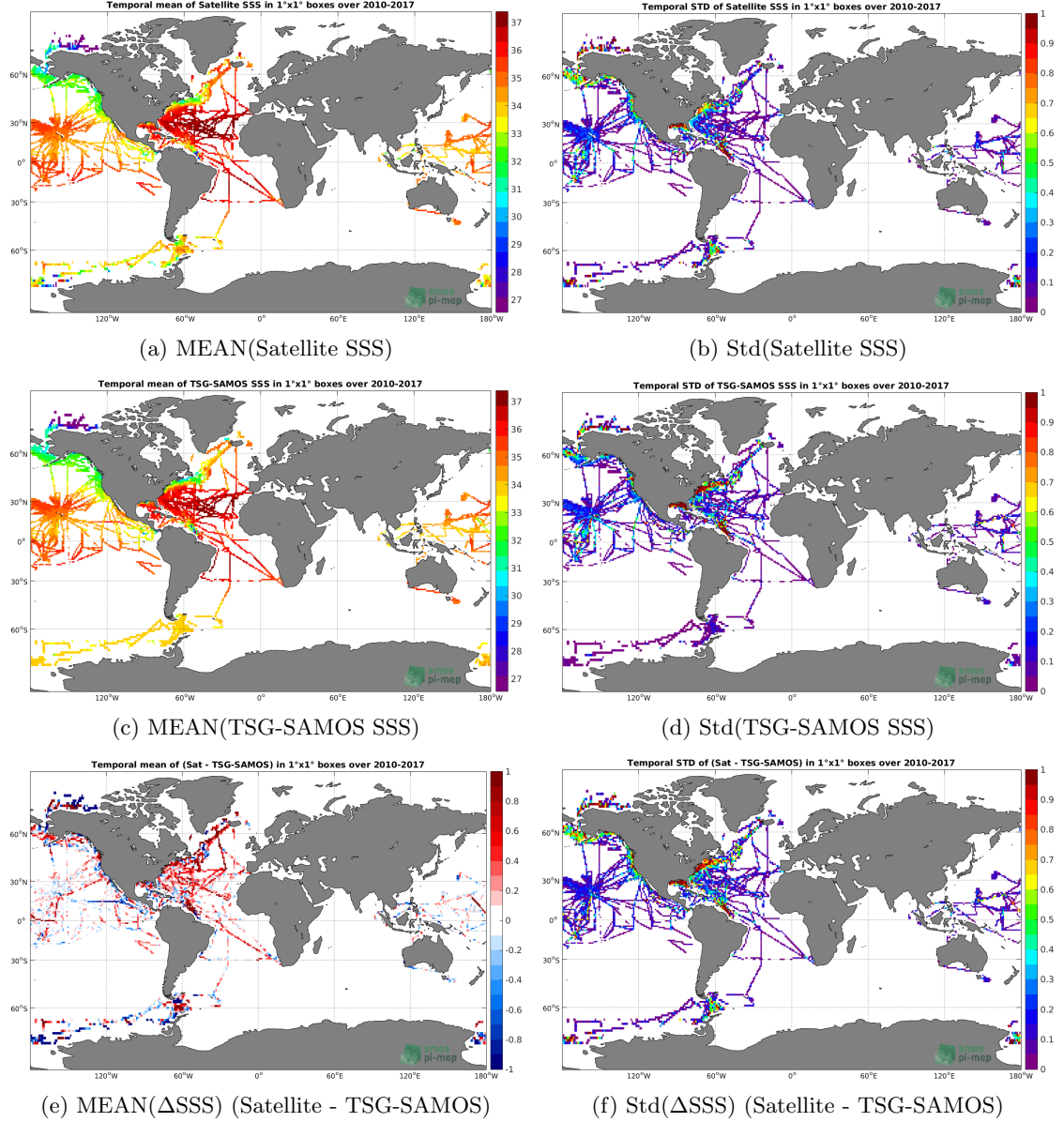
Figure 6: Temporal mean (left) and Std (right) of SSS from SMOS-L4-CATDS-CECOS-IFREMER-V2-WEEKLY-0.5DEG (top), TSG-SAMOS (middle), and of \Delta SSS (Satellite - TSG-SAMOS). Only match-up pairs are used to generate these maps.
