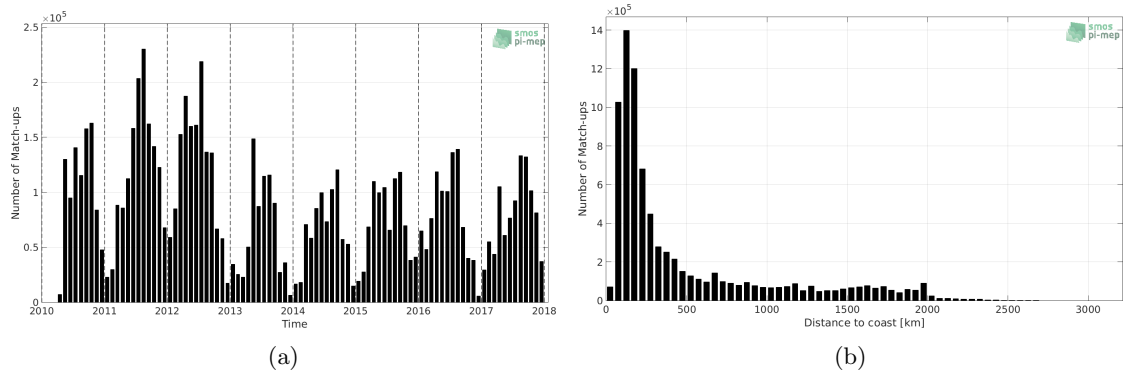
Figure 1: Number of match-ups between TSG-SAMOS and SMOS-L4-CATDS-CECOS-IFREMER-V2-WEEKLY-0.5DEG SSS as a function of time (a) and as function of the distance to coast (b) over the Global Ocean Pi-MEP region and for the full satellite product period.
