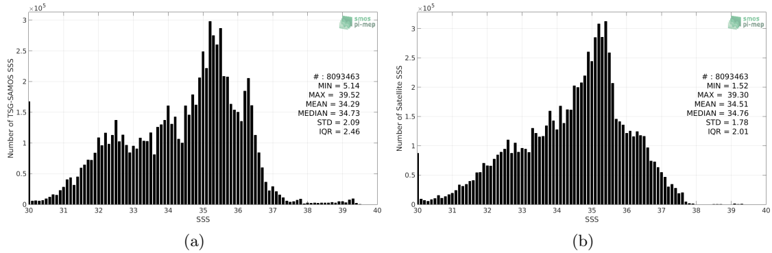
Figure 2: Histograms of SSS from TSG-SAMOS (a) and SMOS-L4-CATDS-CECOS-IFREMER-V2-WEEKLY-0.5DEG (b) considering all match-up pairs per bins of 0.1 over the Global Ocean Pi-MEP region and for the full satellite product period.
