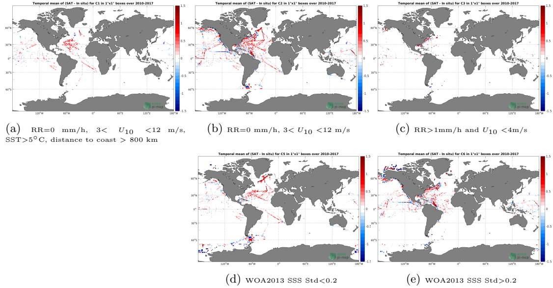
Figure 12: Temporal mean gridded over spatial boxes of size 1^\circ \times 1^\circ of \Delta SSS (SMOS-L4-CATDS-CECOS-IFREMER-V2-WEEKLY-0.5DEG - TSG-SAMOS) for 5 different subdatasets corresponding to:RR=0 mm/h, 3 < U_{10} < 12 m/s, SST >5^\circ\text{C} , distance to coast > 800 km (a), RR=0 mm/h, 3 < U_{10} < 12 m/s (b), RR >1 mm/h and U_{10} < 4 m/s (c), WOA2013 SSS Std <0.2 (d), WOA2013 SSS Std >0.2 (e).
